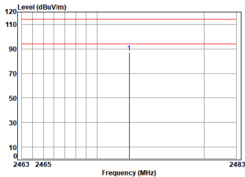
2.4G_SRD_HIGH_TX_Horizontal
