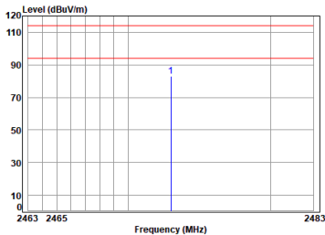
2.4G_SRD_HIGH_TX_Vertical
