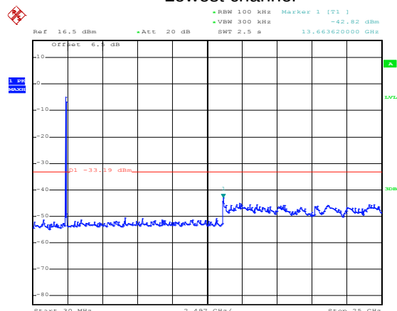
Test mode: 802.11n(H40) Lowest channel
