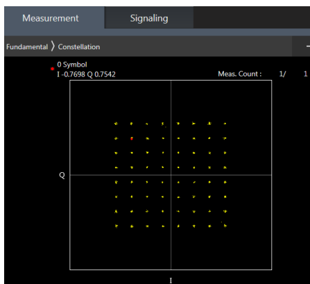
64QAM
