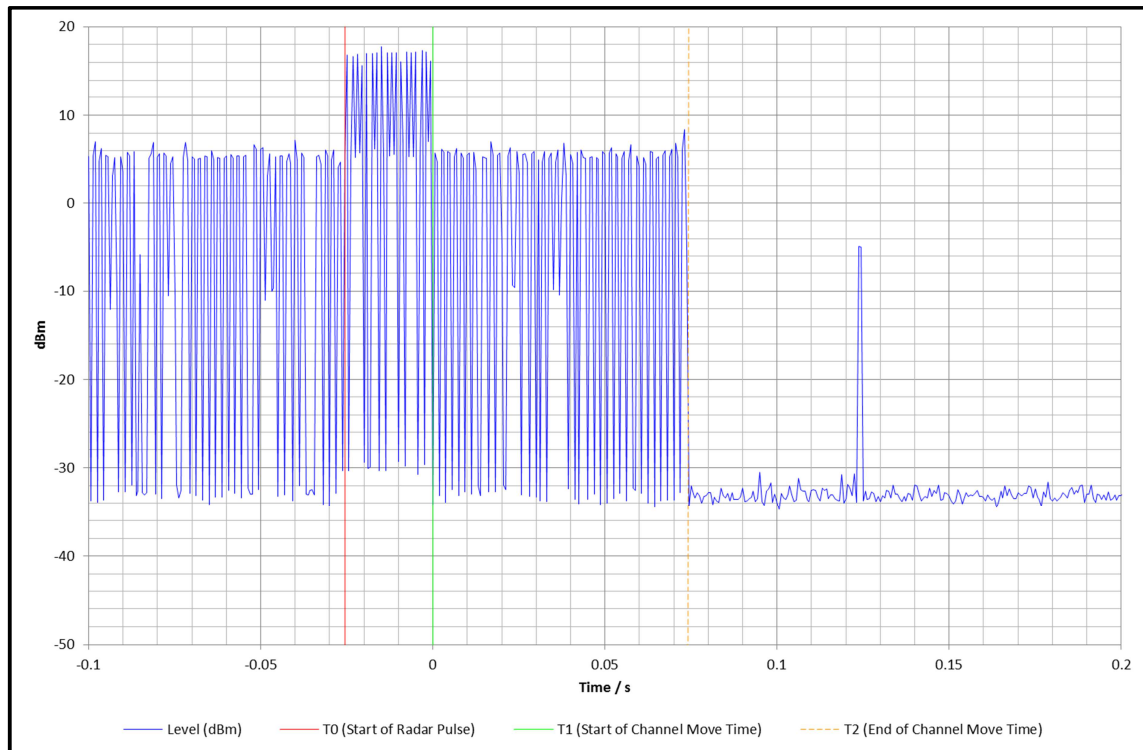
Channel Move Time 5320 MHz – Short Radar (Type 0) – Zoomed Plot
