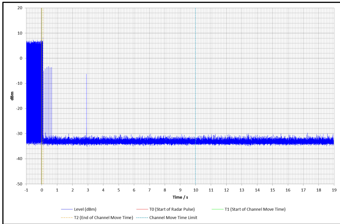
Channel Move Time 5320 MHz – Short Radar (Type 0) – Full 10 seconds
