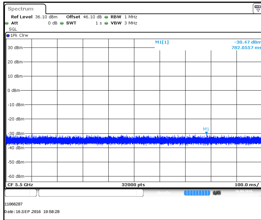
Noise Floor of Spectrum Analyser
