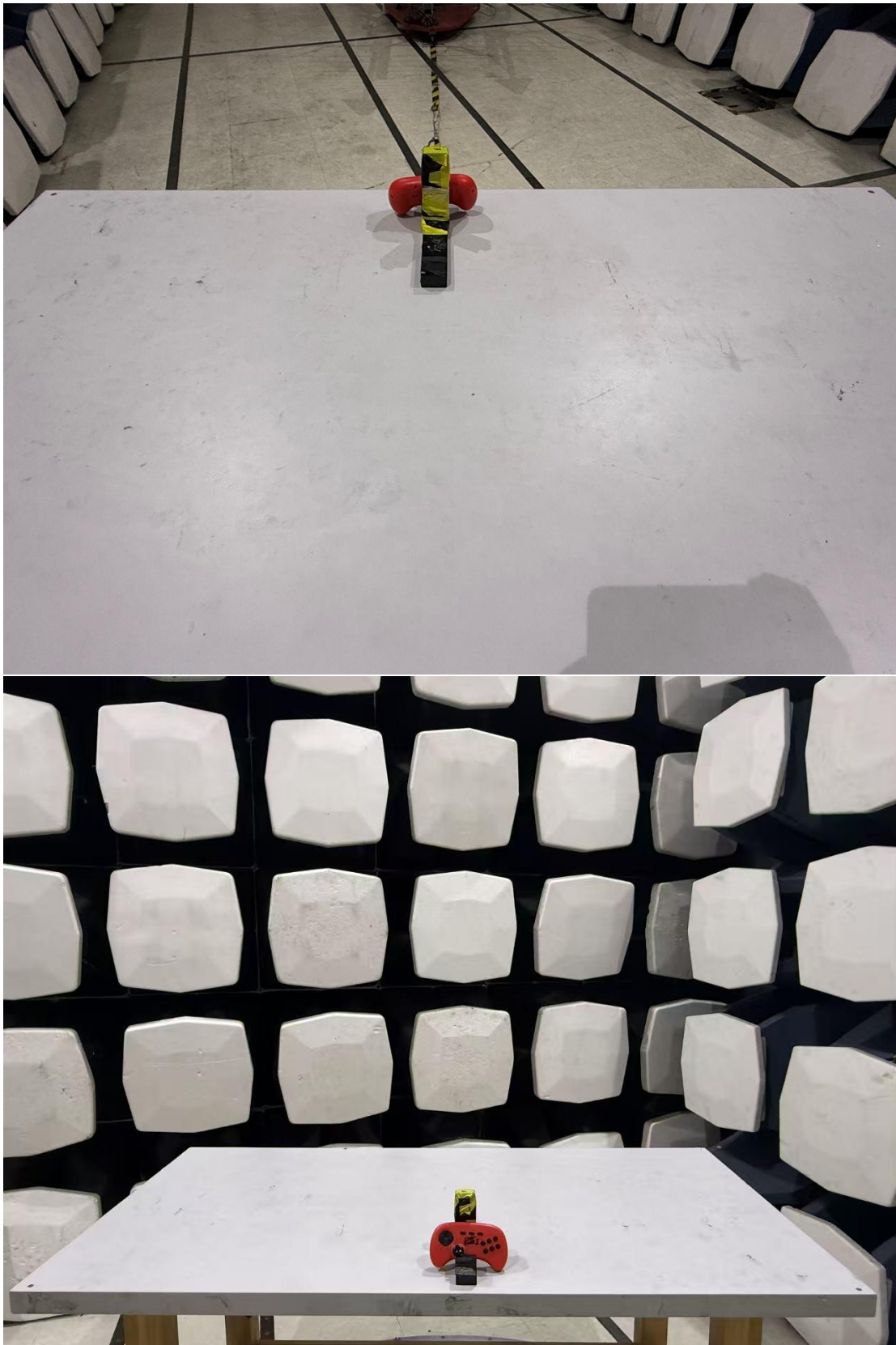
Up to 1GHz (The EUT placed at the center of the turntable)
