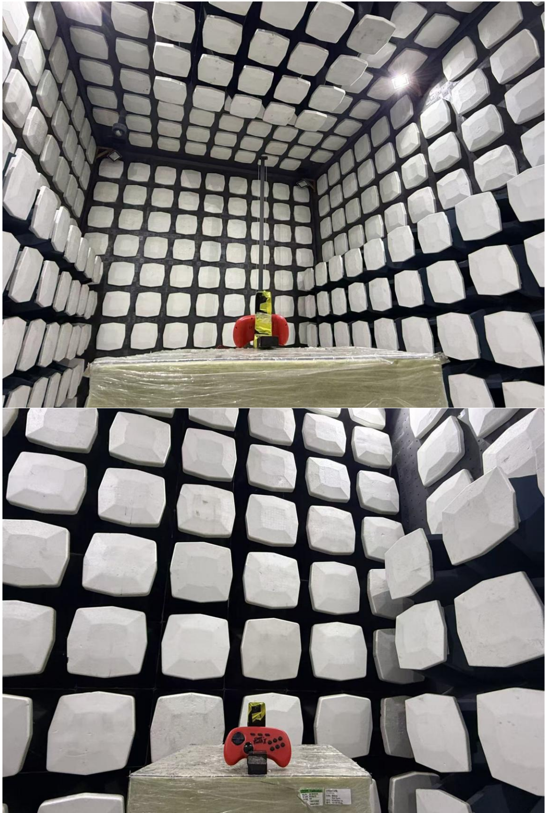
Above 1GHz (The EUT placed at the center of the turntable)
