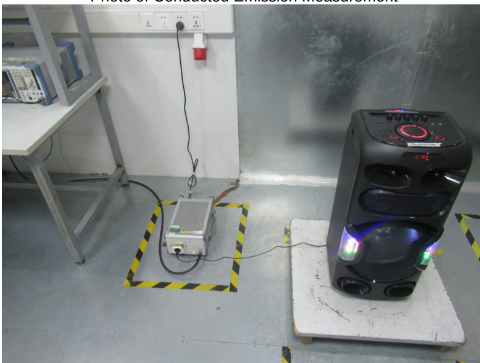
FCC ID: 2AIPR-PS112 Photo of Conducted Emission Measurement
