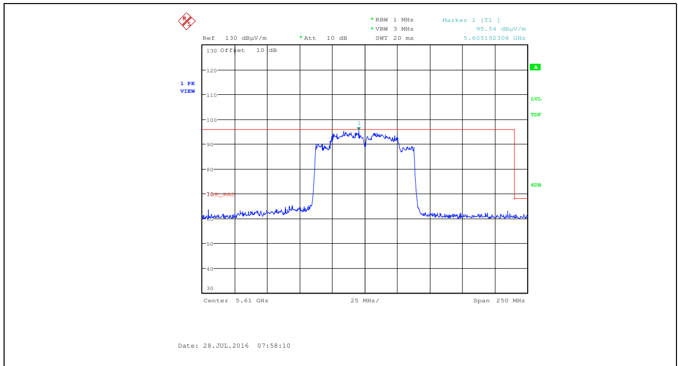
Plot 5.3.10.1.41. Band-Edge Rad Emissions, 802.11ac80, VHT6, Ch 122, 5610 MHz, SISO, Gain Control 23, Vert, Chain # 2
