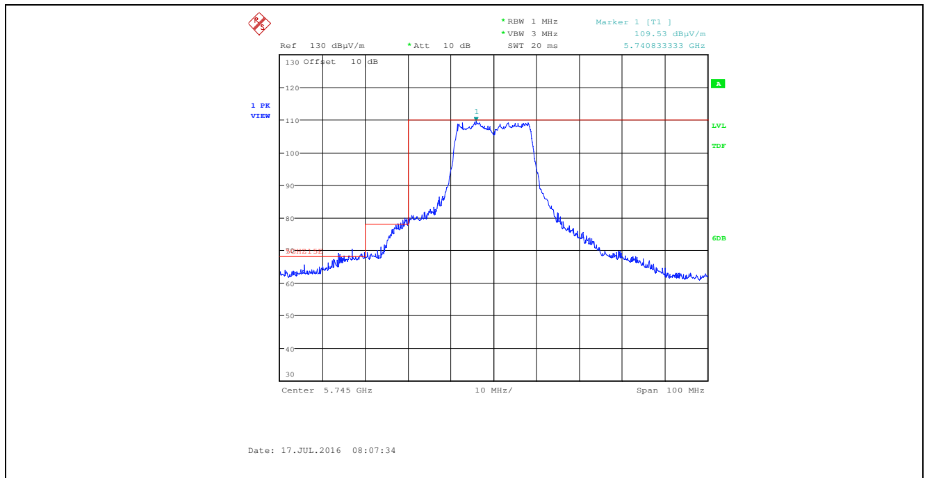
Plot 5.3.12.1.13. Band-Edge Rad Emissions, 802.11n HT20, HT4, Ch 149, 5745 MHz, SISO, Gain Control 33, Vert, Chain # 2
