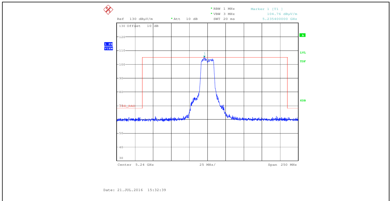
Plot 5.3.6.1.16. Band-Edge Rad Emissions, 802.11n HT20, HT4, Ch 48, 5240 MHz, SISO, Gain Control 31, Horiz, Chain # 2
