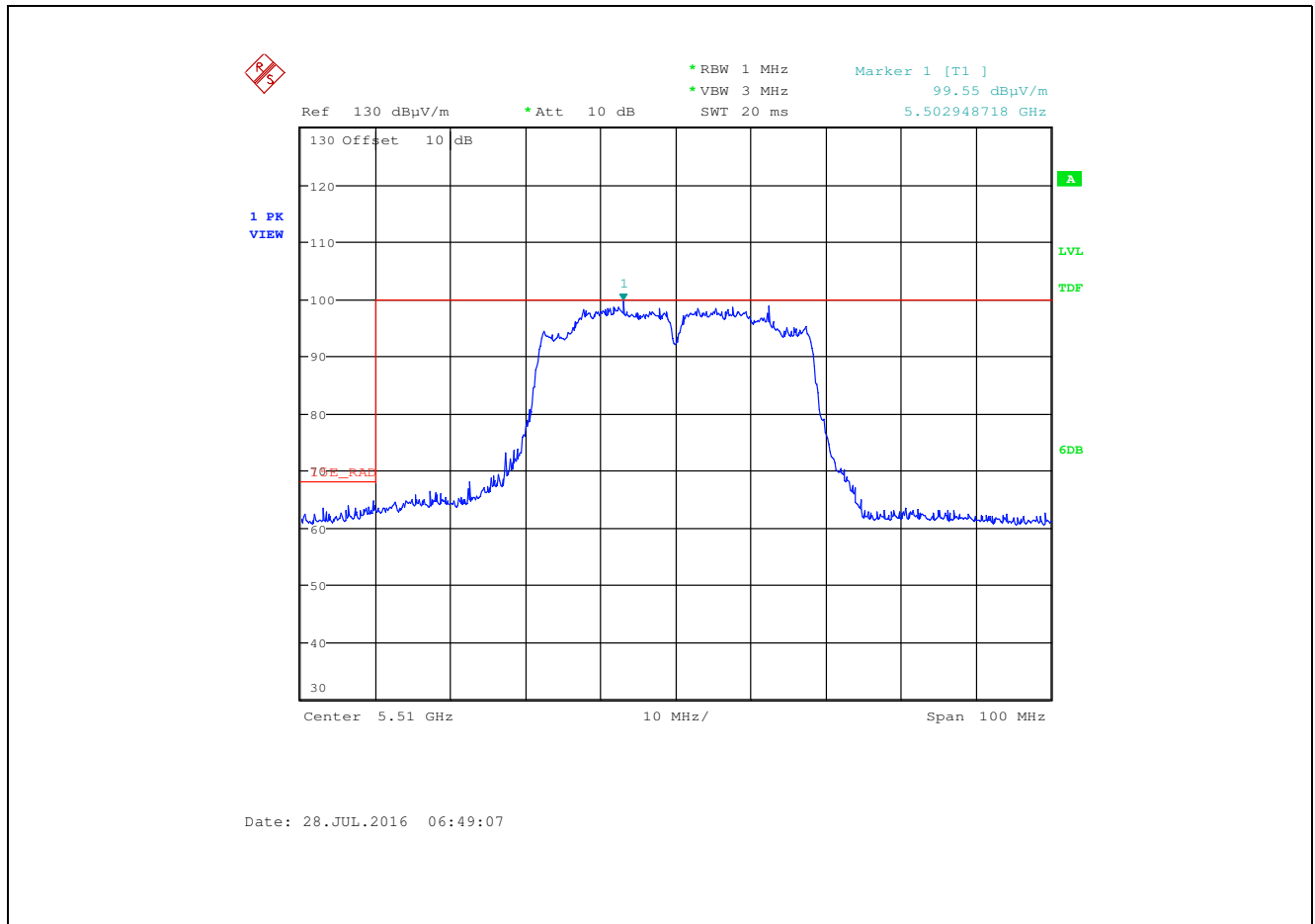
Plot 5.3.10.1.18. Band-Edge Rad Emissions, 802.11n HT20, HT4, Ch 102, 5510 MHz, MIMO, Gain Control 27, Horizontal Chain # 1 & 2
