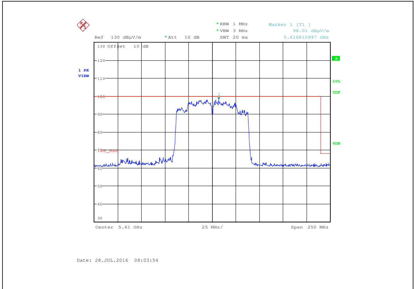
Plot 5.3.10.1.45. Band-Edge Rad Emissions, 802.11ac80, VHT6, Ch 122, 5610 MHz, MIMO, Gain Control 23, Vertical, Chain # 1 & 2
