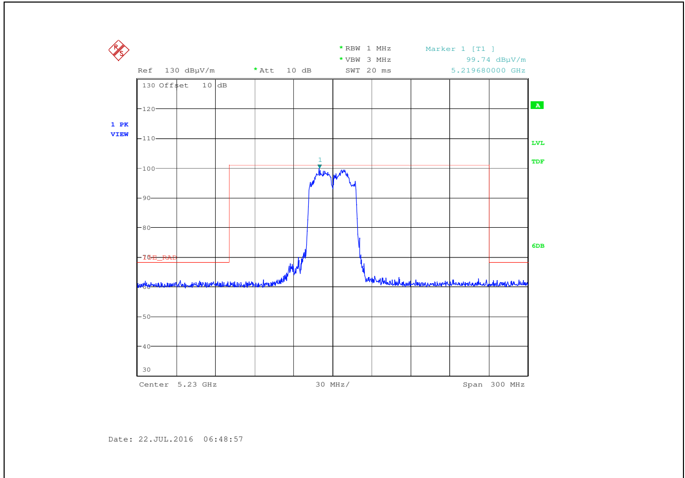
Plot 5.3.6.1.33. Band-Edge Rad Emissions, 802.11n HT40, HT4, Ch 46, 5230 MHz, MIMO, Gain Control 27.5, Horizontal Chain # 1 & 2
