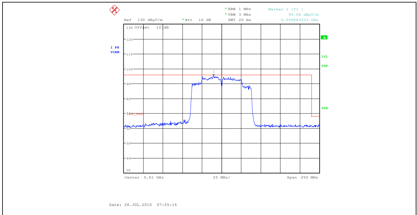
Plot 5.3.10.1.41. Band-Edge Rad Emissions, 802.11ac80, VHT6, Ch 122, 5610 MHz, SISO, Gain Control 23, Vert, Chain # 2
