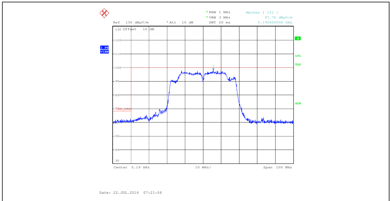
Plot 5.3.6.1.24. Band-Edge Rad Emissions, 802.11n HT40, HT4, Ch 38, 5190 MHz, SISO, Gain Control 27.5, Horiz, Chain # 2
