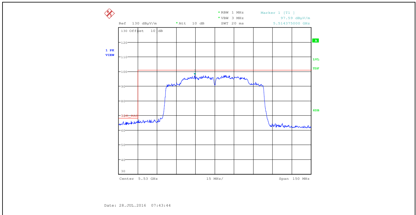
Plot 5.3.10.1.37. Band-Edge Rad Emissions, 802.11ac80, VHT6, Ch 106, 5530 MHz, SISO, Gain Control 23, Vert, Chain # 2
