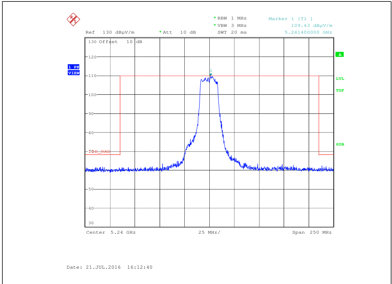
Plot 5.3.6.1.22. Band-Edge Rad Emissions, 802.11n HT20, HT4, Ch 48, 5240 MHz, MIMO, Gain Control 31, Vertical Chain # 1 & 2
