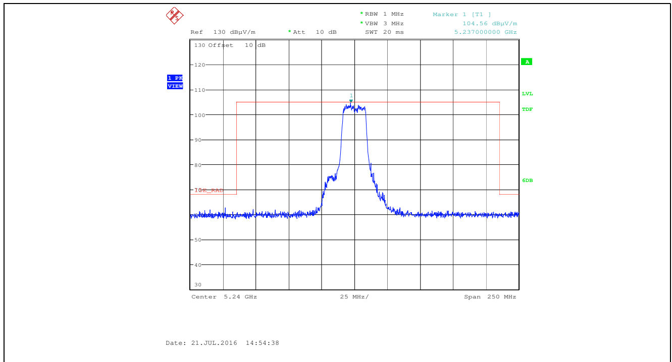
Plot 5.3.6.1.16. Band-Edge Rad Emissions, 802.11n HT20, HT4, Ch 48, 5240 MHz, SISO, Gain Control 31, Horiz, Chain # 2
