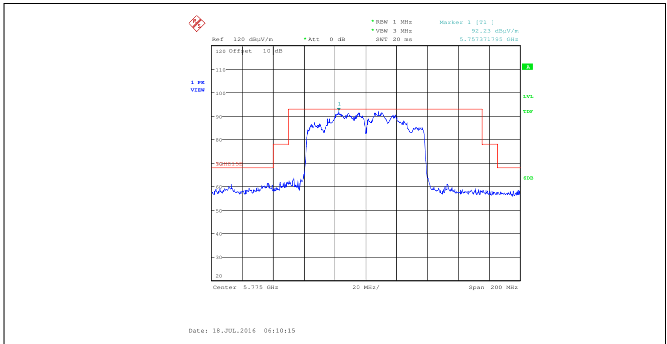
Plot 5.3.12.1.36. Band-Edge Rad Emissions, 802.11ac80, VHT6, Ch 155, 5775 MHz, SISO, Gain Control 28, Horiz, Chain # 2
