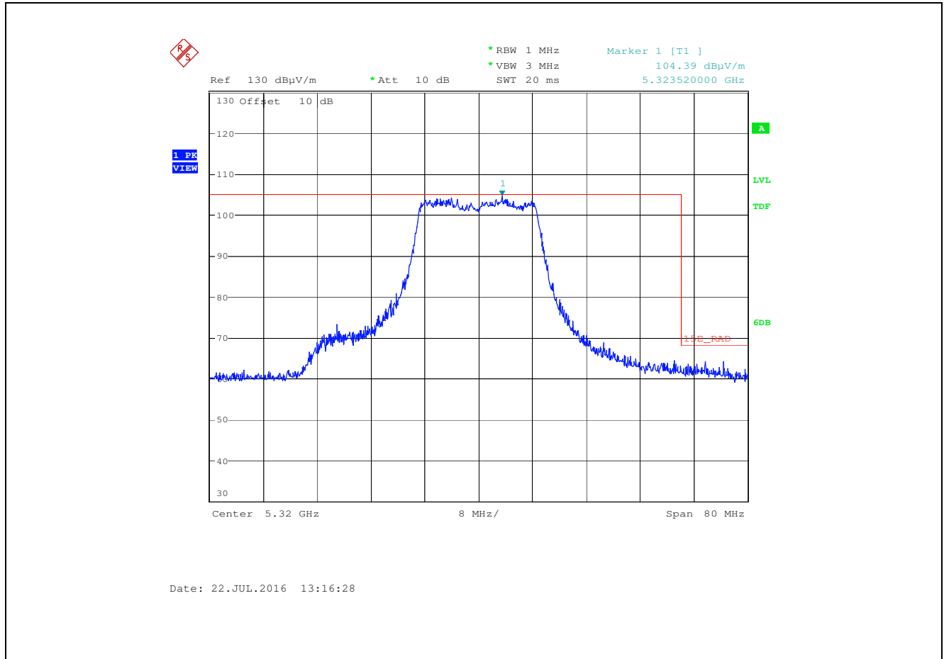
Plot 5.3.8.1.20. Band-Edge Rad Emissions, 802.11n HT20, HT4, Ch 64, 5320 MHz, MIMO, Gain Control 31, Horizontal Chain # 1 & 2
