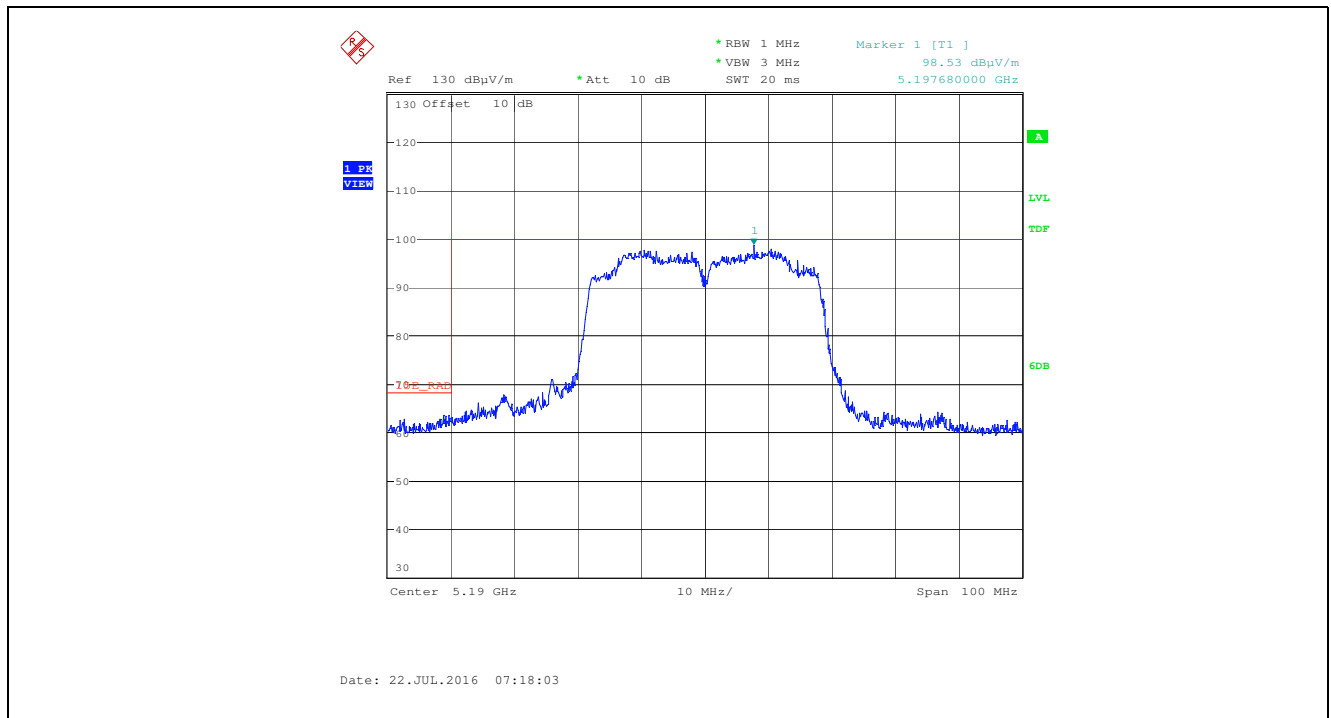
Plot 5.3.6.1.24. Band-Edge Rad Emissions, 802.11n HT40, HT4, Ch 38, 5190 MHz, SISO, Gain Control 27.5, Horiz, Chain # 2
