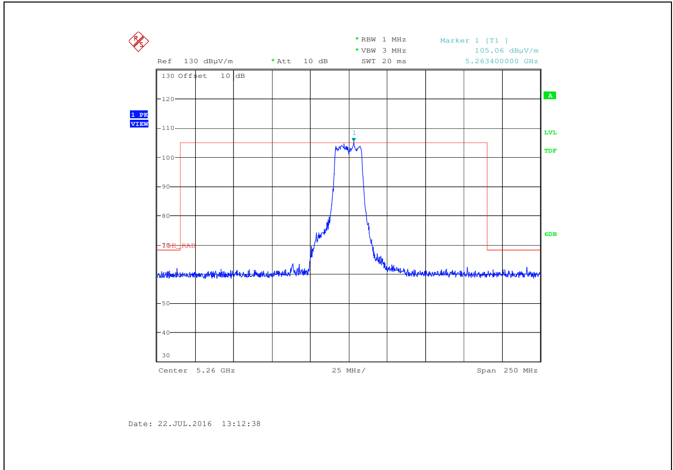
Plot 5.3.8.1.18. Band-Edge Rad Emissions, 802.11n HT20, HT4, Ch 52, 5260 MHz, MIMO, Gain Control 31, Horizontal Chain # 1 & 2
