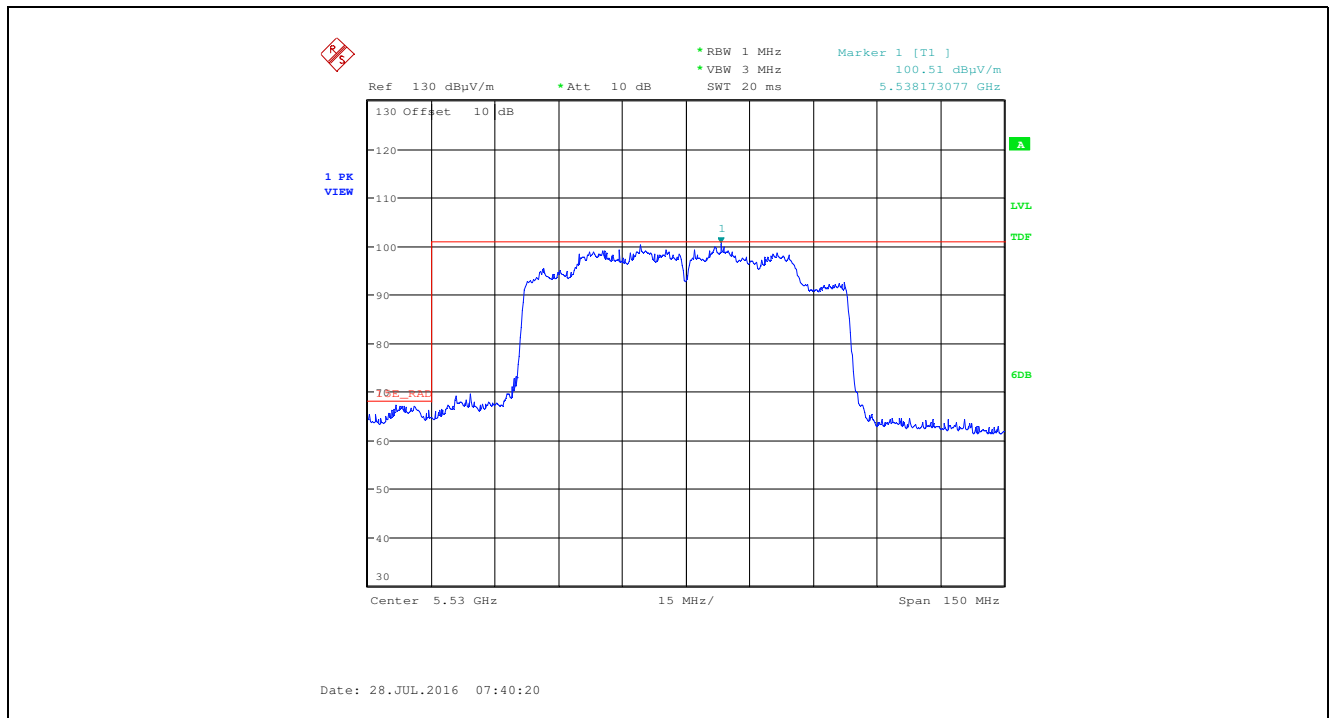
Plot 5.3.10.1.37. Band-Edge Rad Emissions, 802.11ac80, VHT6, Ch 106, 5530 MHz, SISO, Gain Control 23, Vert, Chain # 2
