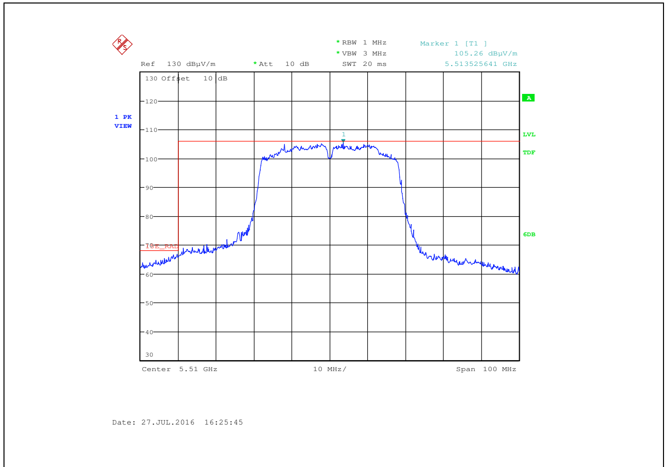
Plot 5.3.10.1.31. Band-Edge Rad Emissions, 802.11n HT40, HT4, Ch 102, 5510 MHz, MIMO, Gain Control 27, Vertical, Chain # 1 & 2
