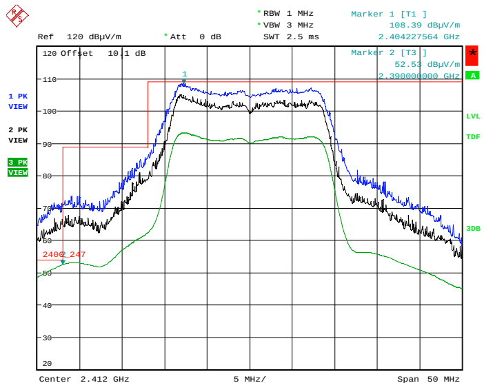
Plot 5.2.5.1.19. Band-Edge Rad Emissions, 802.11n20, HT4, Ch 1, 2412 MHz, SISO, Gain Control 21.5, Vertical, Chain # 1
