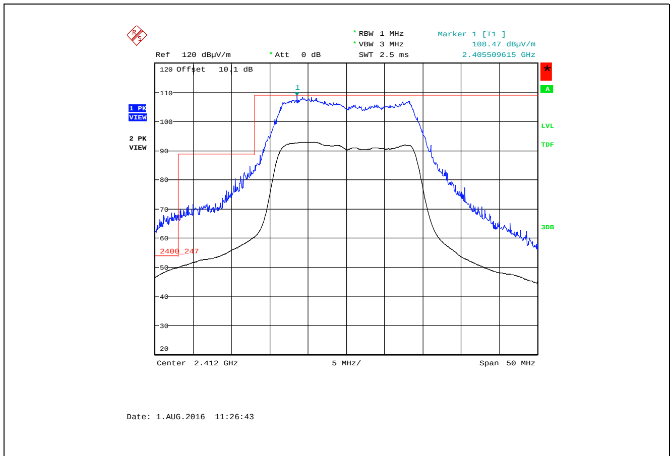
Plot 5.2.5.1.20. Band-Edge Rad Emissions, 802.11n20, HT4, Ch 1, 2412 MHz, SISO, Gain Control 21.5, Vertical, Chain # 2
