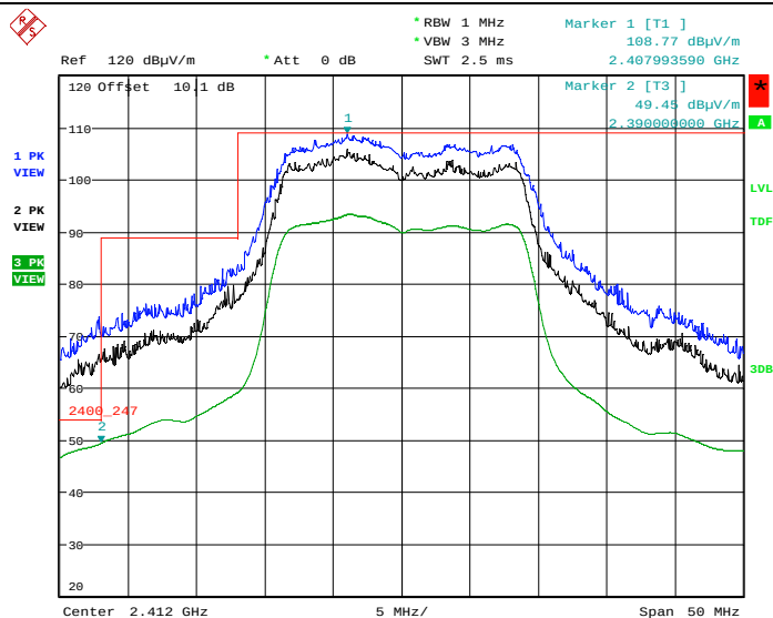
Plot 5.2.5.1.17. Band-Edge Rad Emissions, 802.11n20, HT4, Ch 1, 2412 MHz, SISO, Gain Control 21.5, Horiz, Chain # 1
