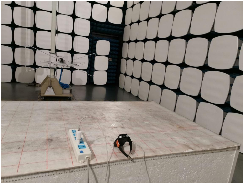
Radiated Emission (for Machine B) Below 1GHz
