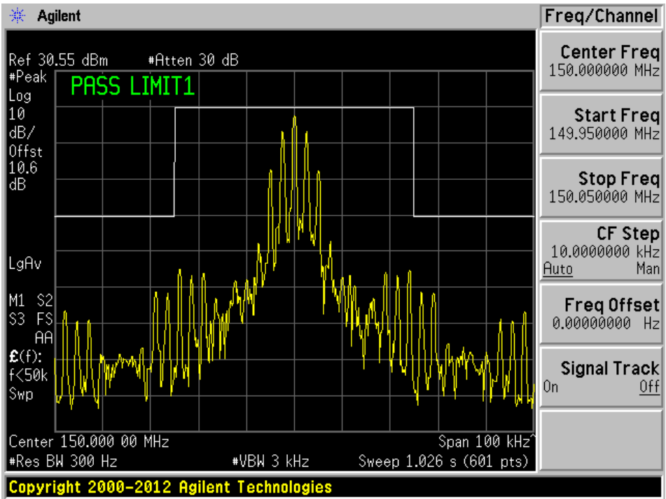
FM 150 MHz
