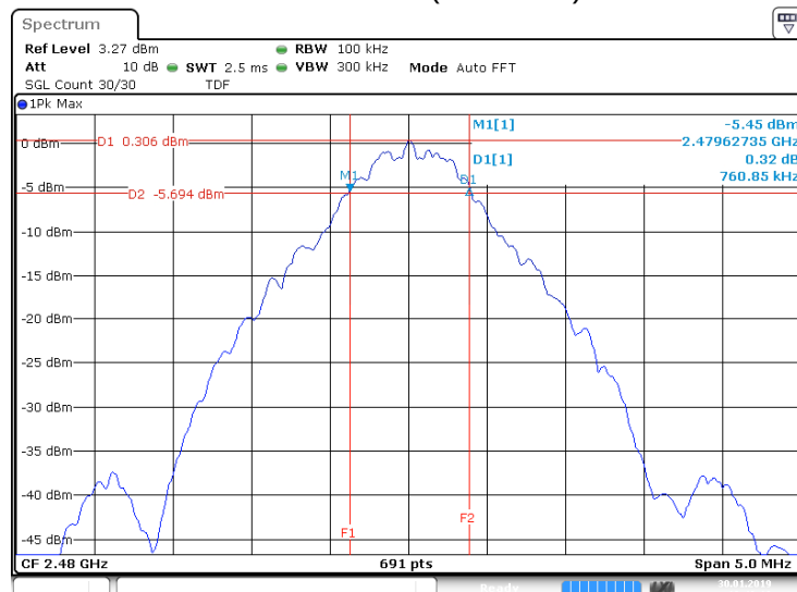
6 dB Bandwidth (Channel 39)
