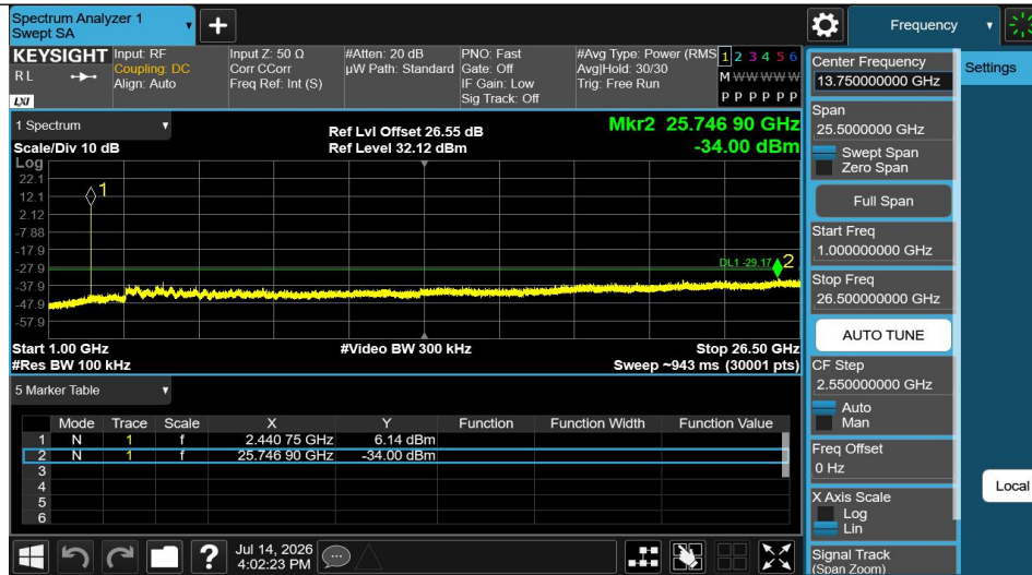
2DH5-Ant1-2441-1000~26500-PASS
