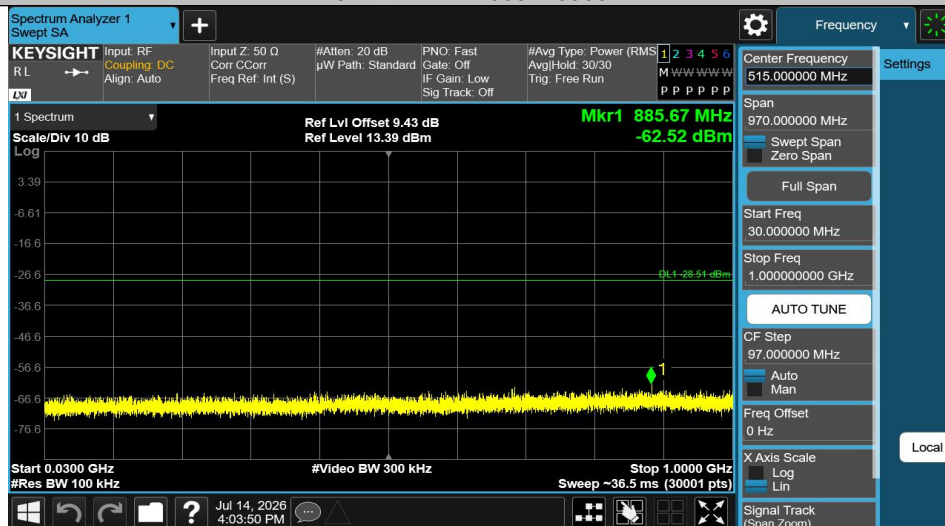
2DH5-Ant1-2480-30~1000-PASS
