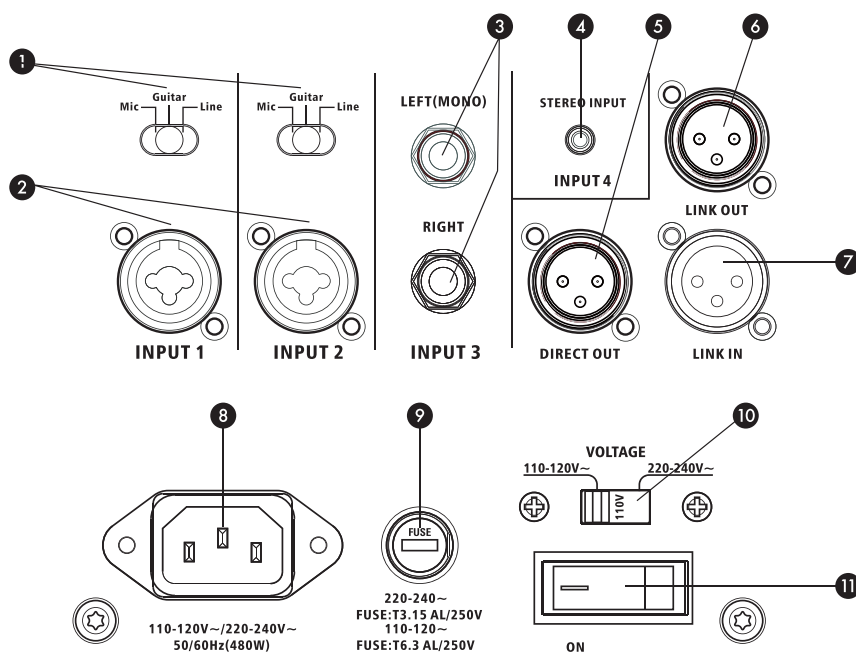
BACK PANEL
