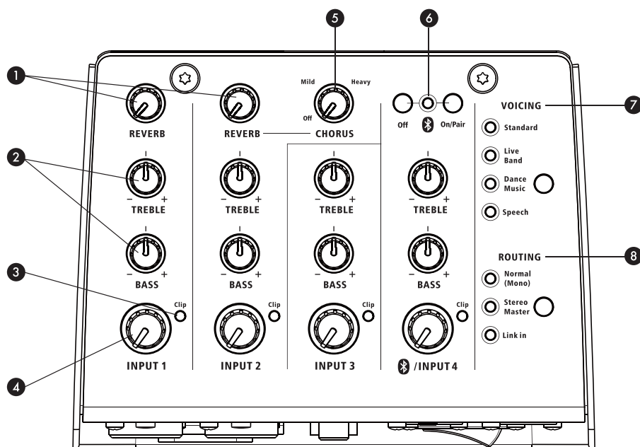
TOP PANEL
