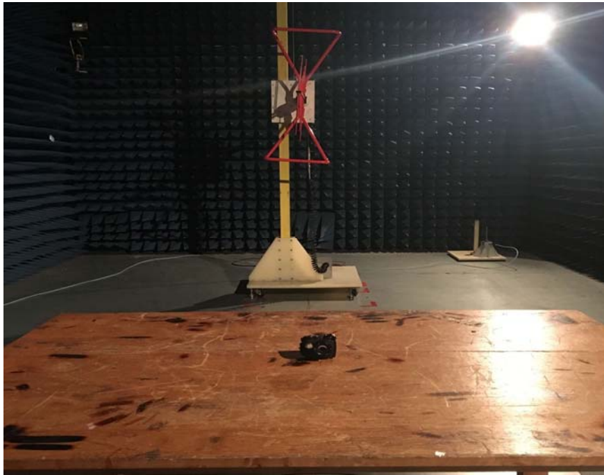
RE TEST SETUP
