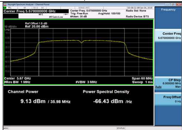
U-NII-2c,802.11n(HT40),5670MHz ,Ant1
