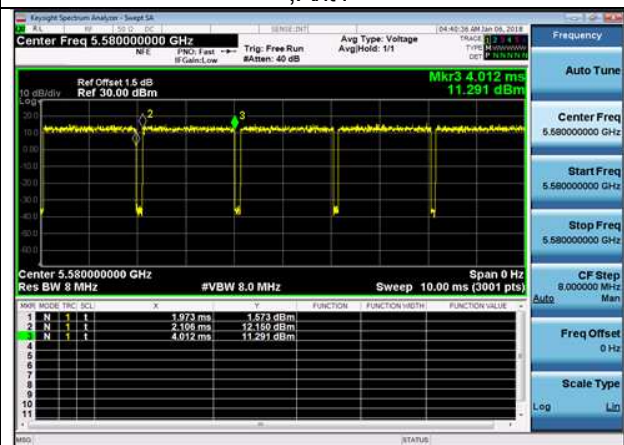
U-NII-2c,802.11n(HT20),5580MHz ,Ant1
