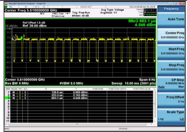
U-NII-2c,802.11ac(VHT80),5610MHz ,Ant1
