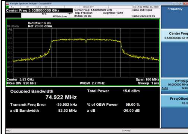
U-NII-2c,802.11ac(VHT80),5530MHz ,Ant1
