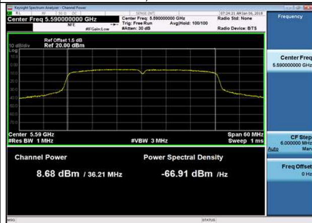
U-NII-2c,802.11n(HT40),5590MHz ,Ant1
