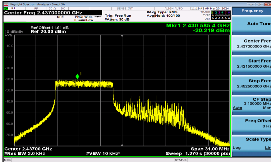
11AX20SISO-Ant1-2437-106Tone-PASS
