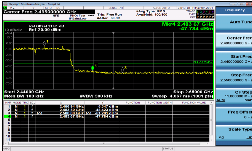
11AX40SISO-Ant1-2452-PASS
