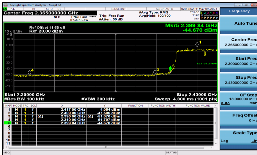
11AC40SISO-Ant1-2422-PASS
