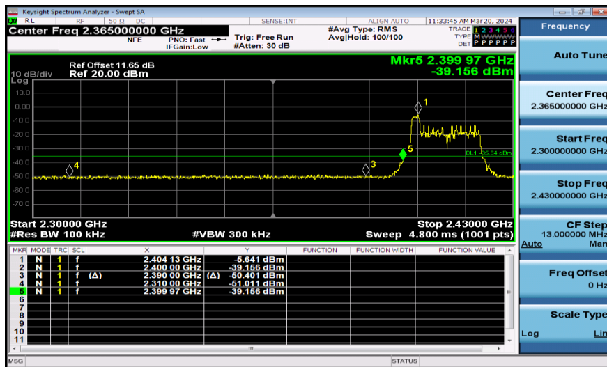
11AX20SISO-Ant1-2412-26Tone-PASS
