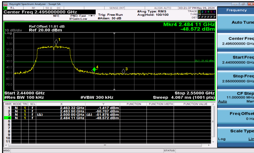
11AC20SISO-Ant1-2462-PASS
