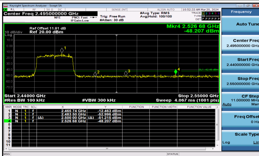
11AX20SISO-Ant1-2462-242Tone-PASS
