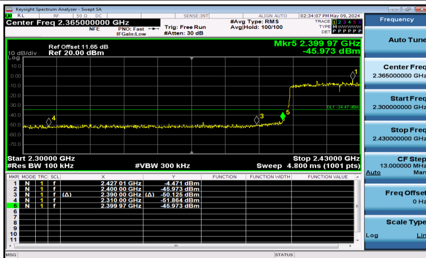
11AX40SISO-Ant1-2422-PASS
