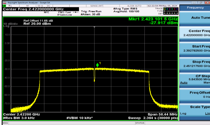
11AX40SISO-Ant1-2422-PASS
