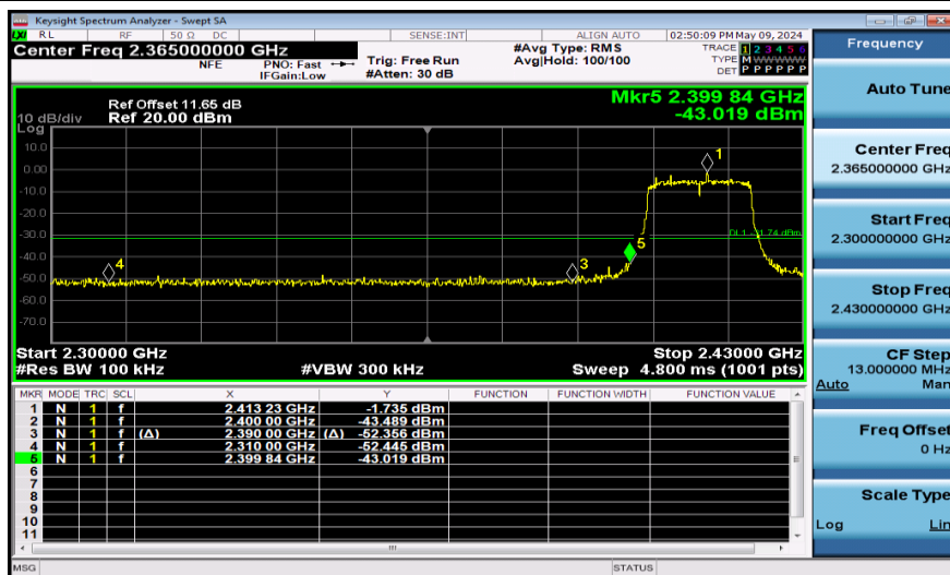
11AC20SISO-Ant1-2412-PASS
