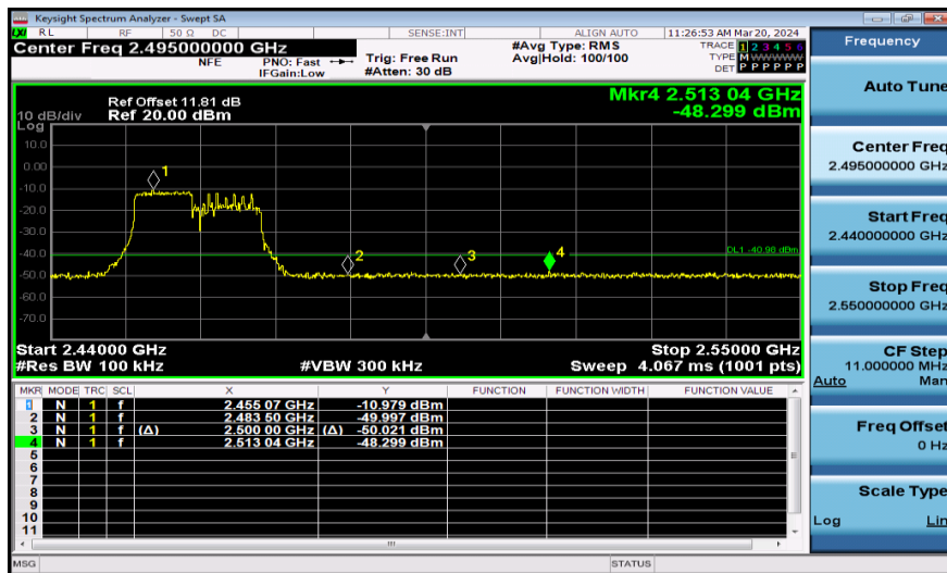
11AX20SISO-Ant1-2462-106Tone-PASS
