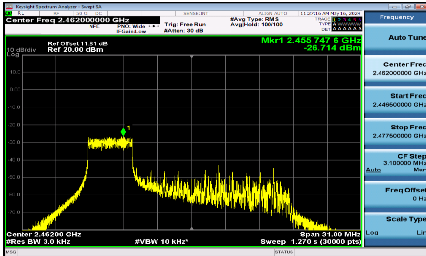
11AX20SISO-Ant1-2462-52Tone-PASS
