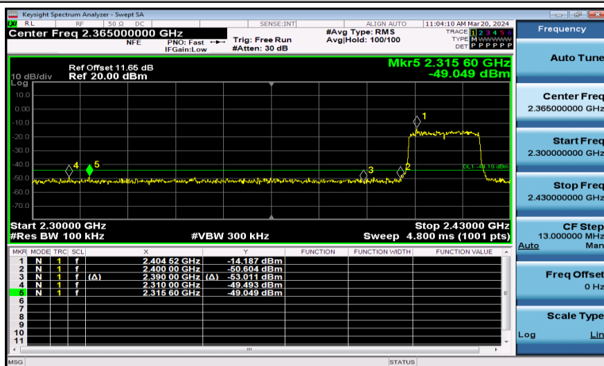
11AX20SISO-Ant1-2412-242Tone-PASS
