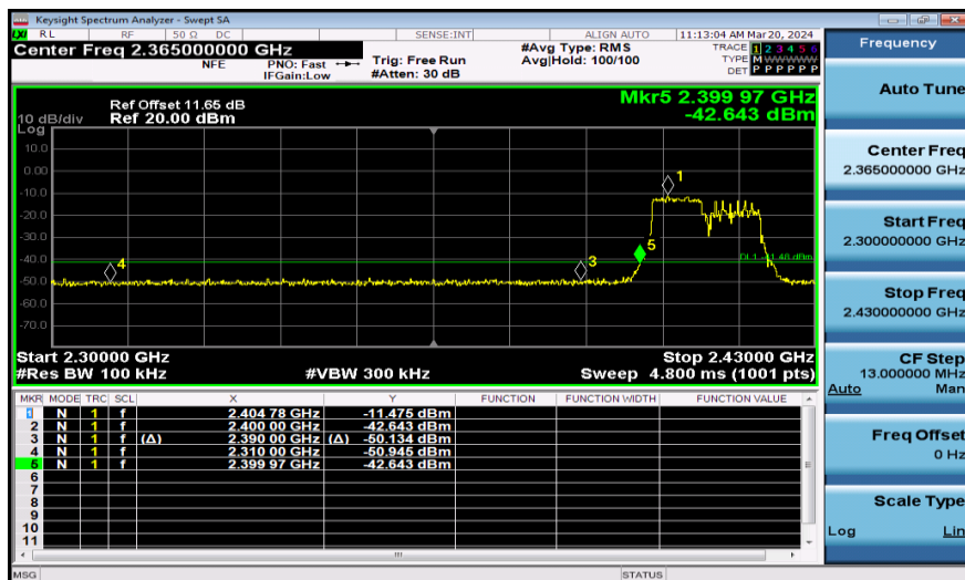
11AX20SISO-Ant1-2412-106Tone-PASS
