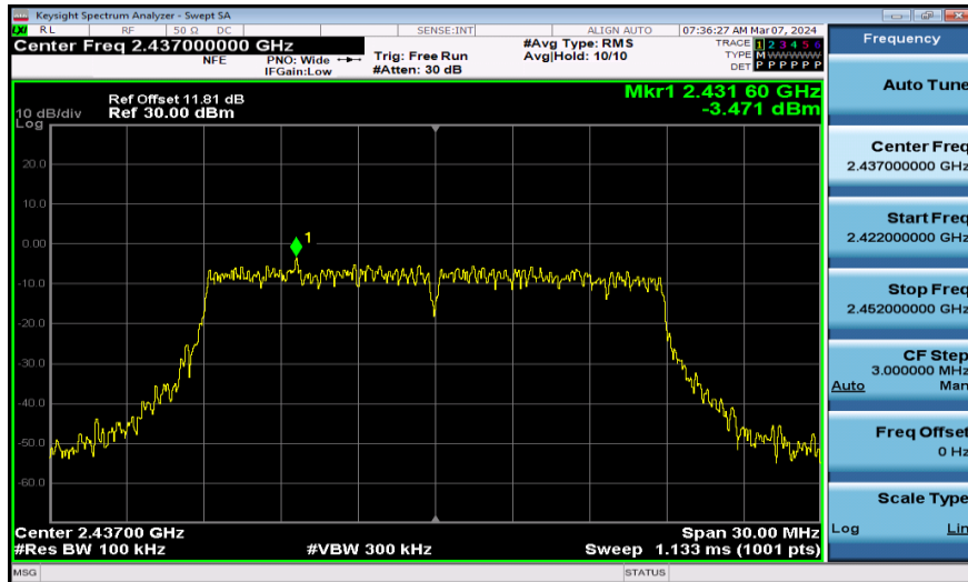
11N20SISO-Ant1-2437-0~Reference-PASS
