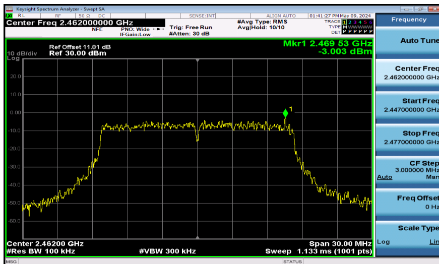
11G-Ant1-2462-0~Reference-PASS
