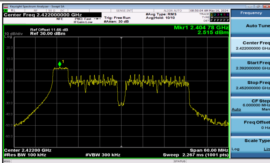
11AX40SISO-Ant1-2422-52Tone-0~Reference-PASS
