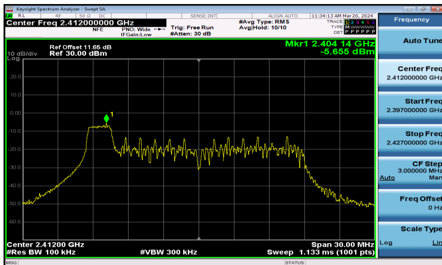
11AX20SISO-Ant1-2412-26Tone-0~Reference-PASS
