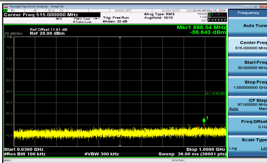
11AX20SISO-Ant1-2462-26Tone-30~1000-PASS
