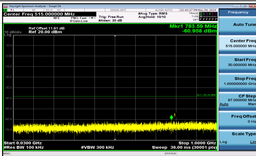
11AX40SISO-Ant1-2452-30~1000-PASS
