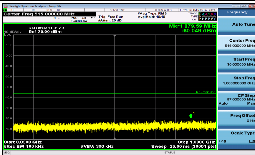
11AX20SISO-Ant1-2462-52Tone-30~1000-PASS
