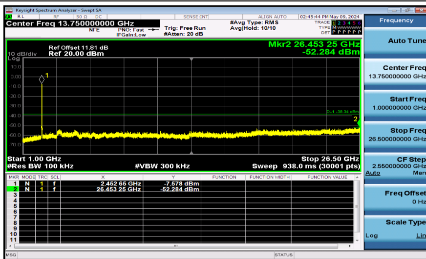
11AX40SISO-Ant1-2452-1000~26500-PASS
