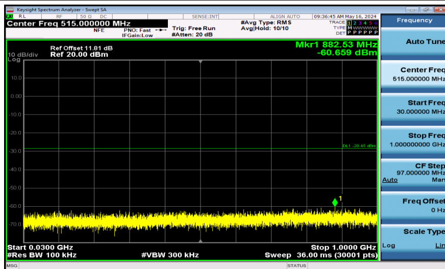
11AX40SISO-Ant1-2437-52Tone-30~1000-PASS
