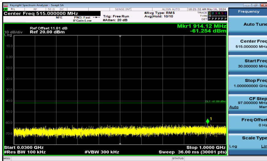
11AX40SISO-Ant1-2437-484Tone-30~1000-PASS
