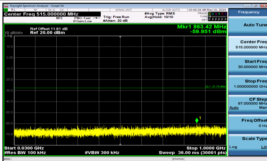
11AX40SISO-Ant1-2452-52Tone-30~1000-PASS
