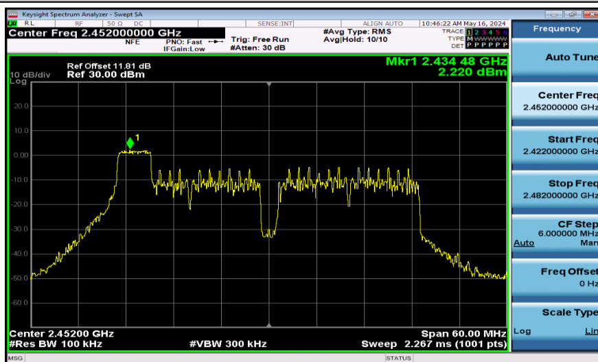
11AX40SISO-Ant1-2452-52Tone-0~Reference-PASS
