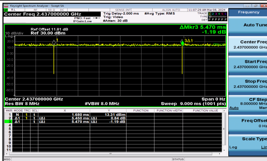
NTNV-11AX20SISO-Ant1-2437
