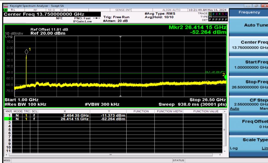
11AX40SISO-Ant1-2437-484Tone-1000~26500-PASS
