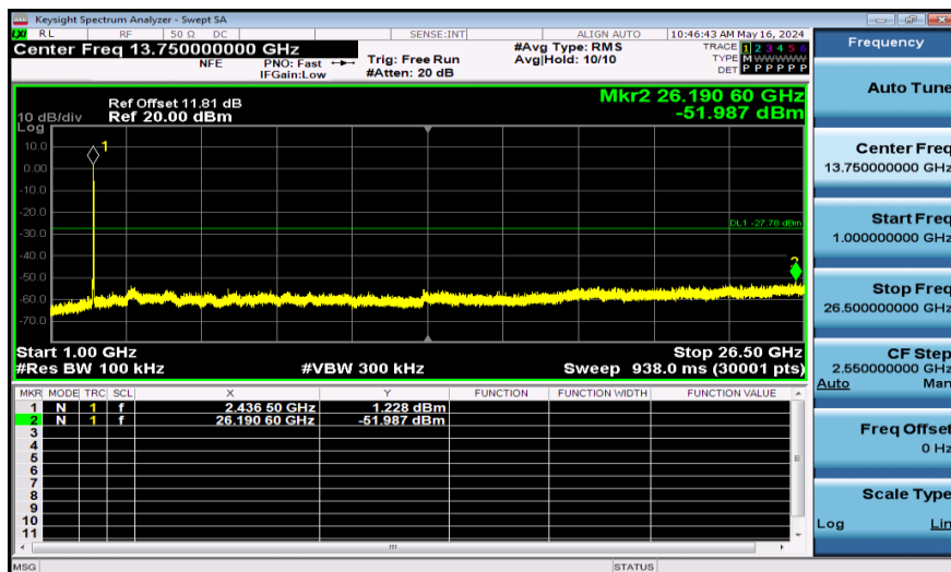
11AX40SISO-Ant1-2452-52Tone-1000~26500-PASS
