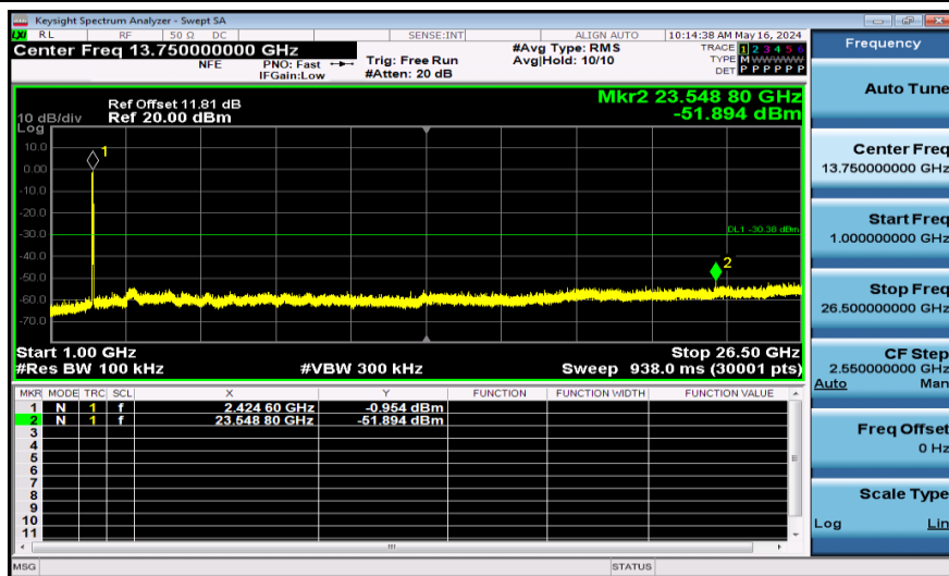
11AX40SISO-Ant1-2437-106Tone-1000~26500-PASS
