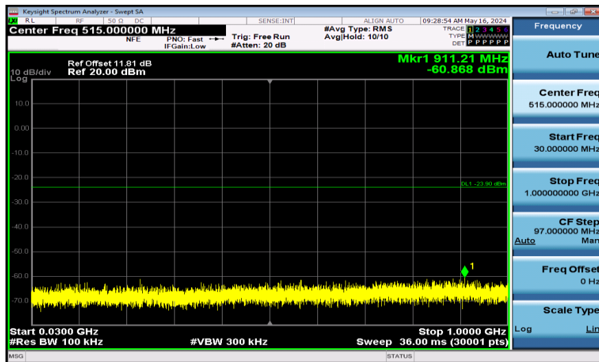
11AX40SISO-Ant1-2437-26Tone-30~1000-PASS
