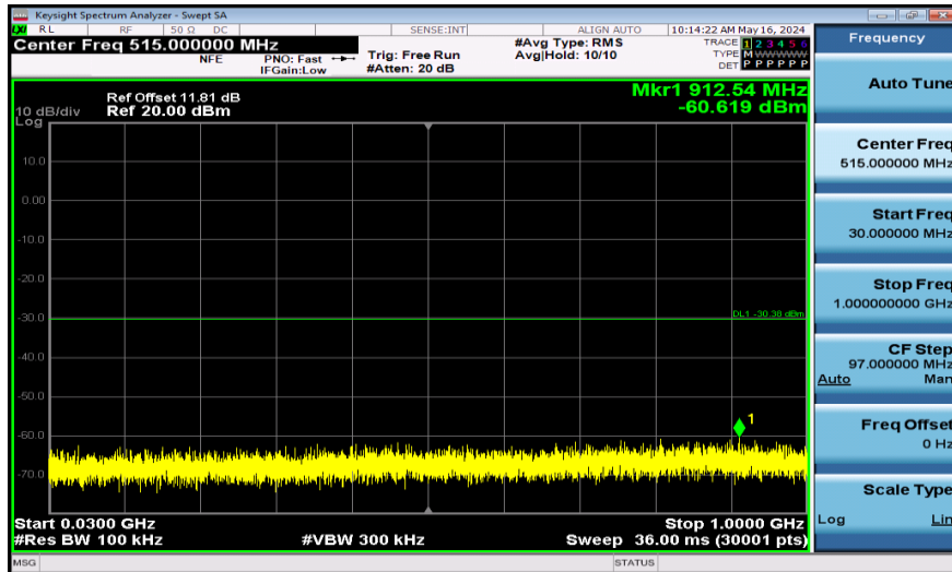
11AX40SISO-Ant1-2437-106Tone-30~1000-PASS
