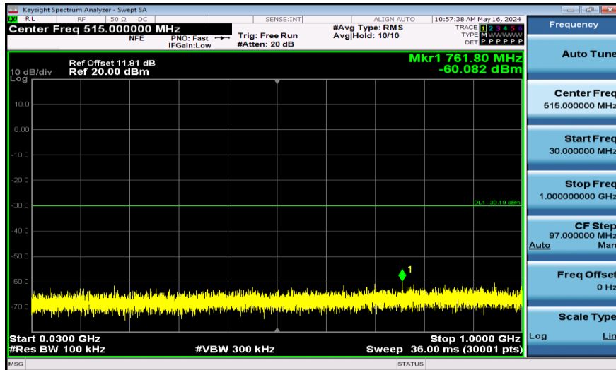
11AX40SISO-Ant1-2452-106Tone-30~1000-PASS
