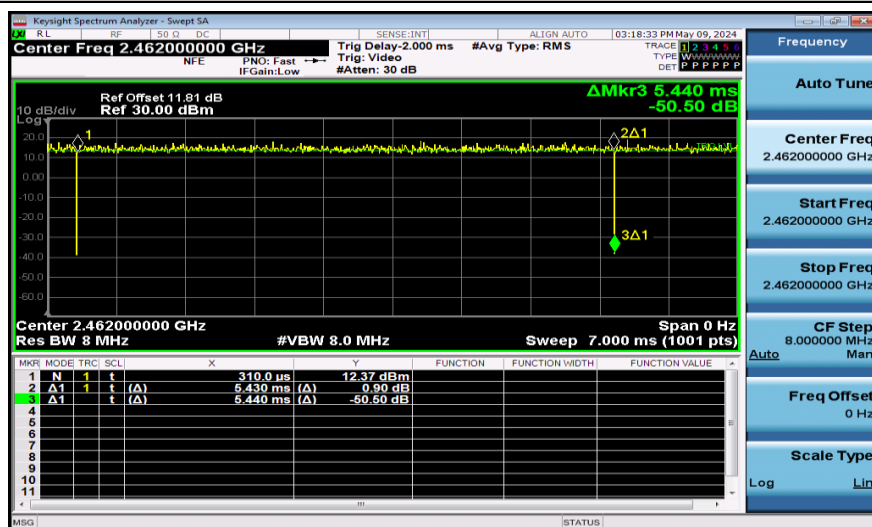
NTNV-11AC20SISO-Ant1-2462
