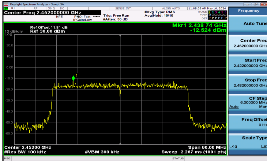
11AX40SISO-Ant1-2452-484Tone-0~Reference-PASS
