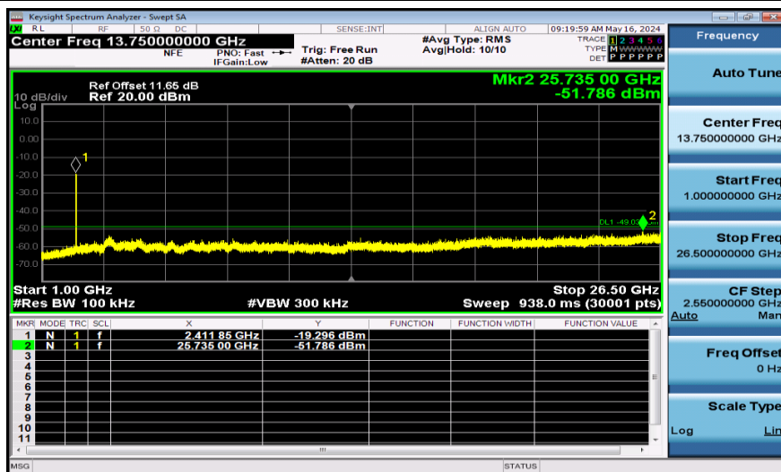
11AX40SISO-Ant1-2422-484Tone-1000~26500-PASS
