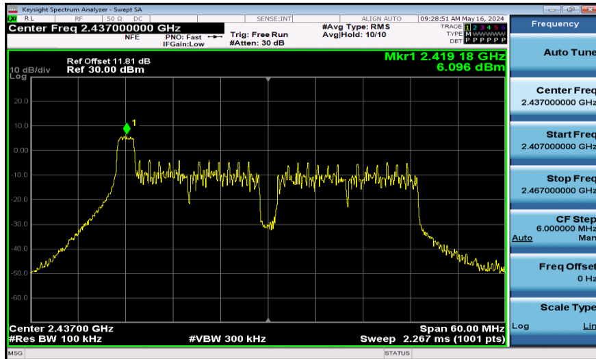
11AX40SISO-Ant1-2437-26Tone-0~Reference-PASS
