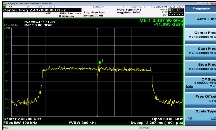
11AX40SISO-Ant1-2437-484Tone-0~Reference-PASS
