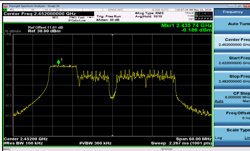
11AX40SISO-Ant1-2452-106Tone-0~Reference-PASS
