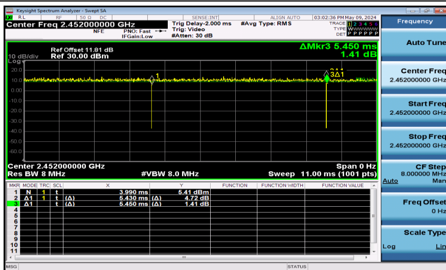
NTNV-11AC40SISO-Ant1-2452
