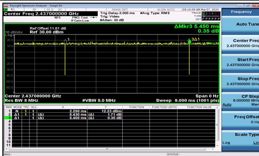
NTNV-11AC20SISO-Ant1-2437
