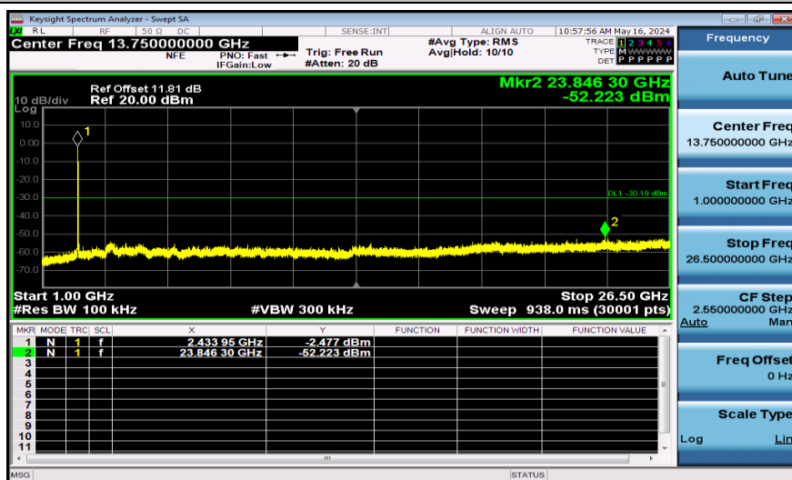
11AX40SISO-Ant1-2452-106Tone-1000~26500-PASS
