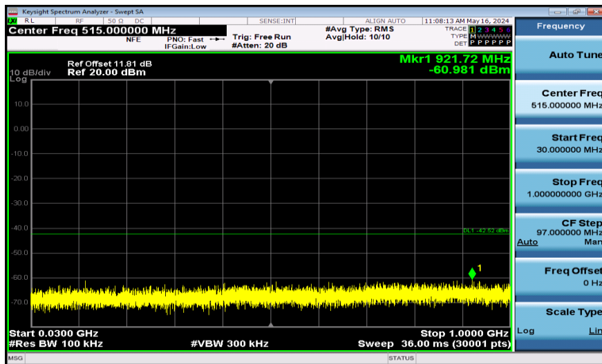
11AX40SISO-Ant1-2452-484Tone-30~1000-PASS
