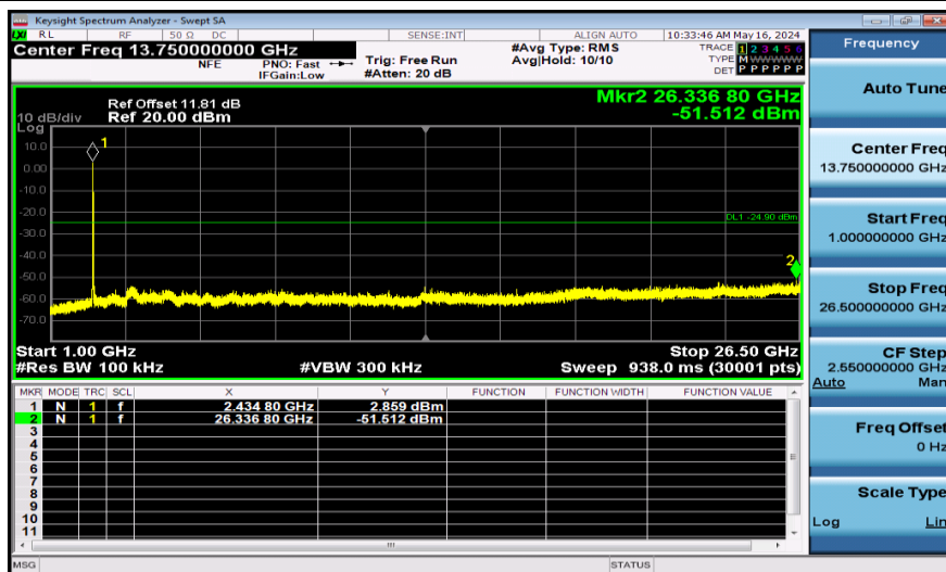
11AX40SISO-Ant1-2452-26Tone-1000~26500-PASS
