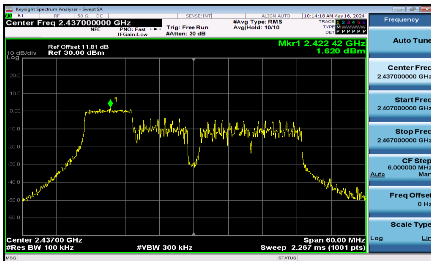
11AX40SISO-Ant1-2437-106Tone-0~Reference-PASS
