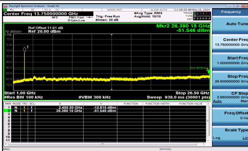
11AX40SISO-Ant1-2452-484Tone-1000~26500-PASS
