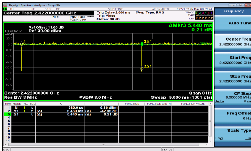
NTNV-11AC40SISO-Ant1-2422
