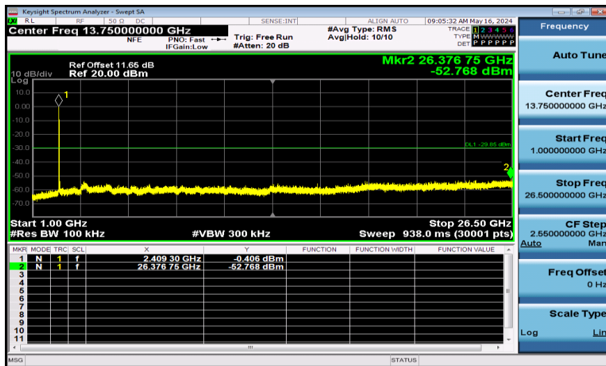
11AX40SISO-Ant1-2422-106Tone-1000~26500-PASS
