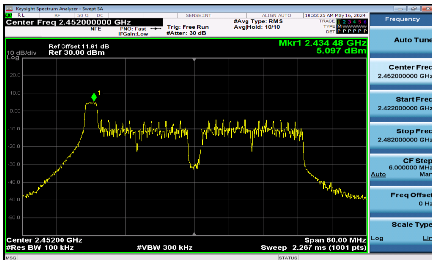
11AX40SISO-Ant1-2452-26Tone-0~Reference-PASS
