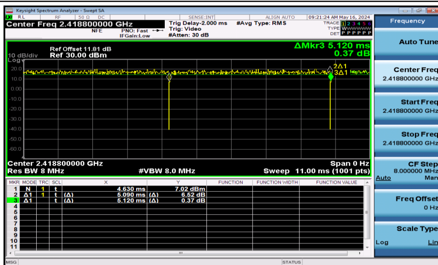
NTNV-11AX40SISO-Ant1-2437-26Tone
