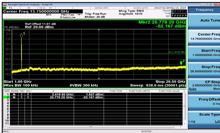
11AX40SISO-Ant1-2437-52Tone-1000~26500-PASS
