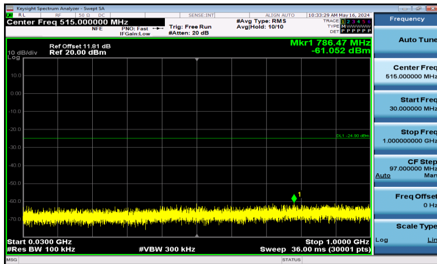
11AX40SISO-Ant1-2452-26Tone-30~1000-PASS
