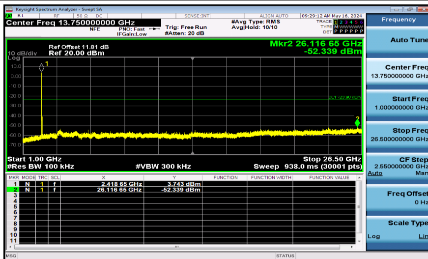
11AX40SISO-Ant1-2437-26Tone-1000~26500-PASS
