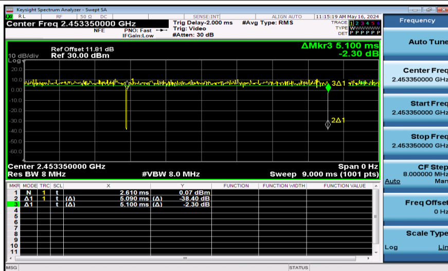
NTNV-11AX20SISO-Ant1-2462-26Tone
