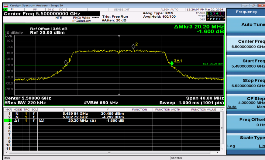
11AC20SISO-Ant1-5500
