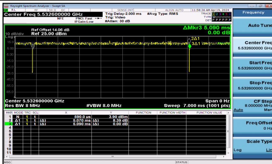
NTNV-11AX40SISO-Ant1-5550-52Tone
