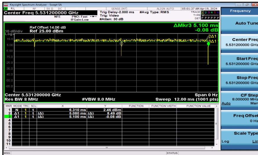
NTNV-11AX40SISO-Ant1-5550-26Tone
