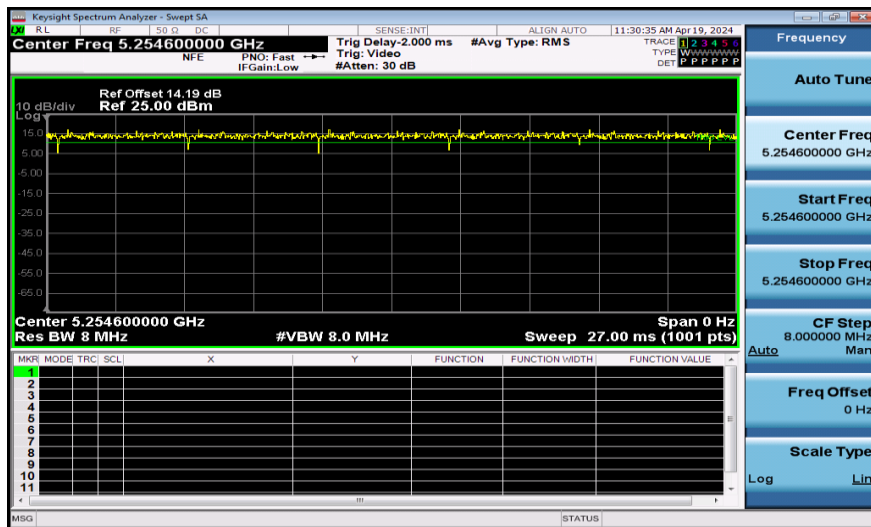
NTNV-11AX40SISO-Ant1-5270-52Tone
