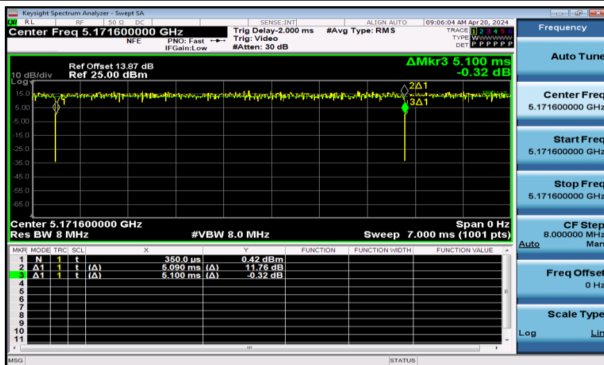
NTNV-11AX80SISO-Ant1-5210-26Tone
