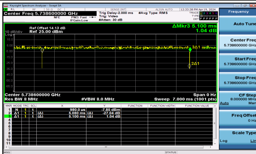
NTNV-11AX40SISO-Ant1-5755-52Tone
