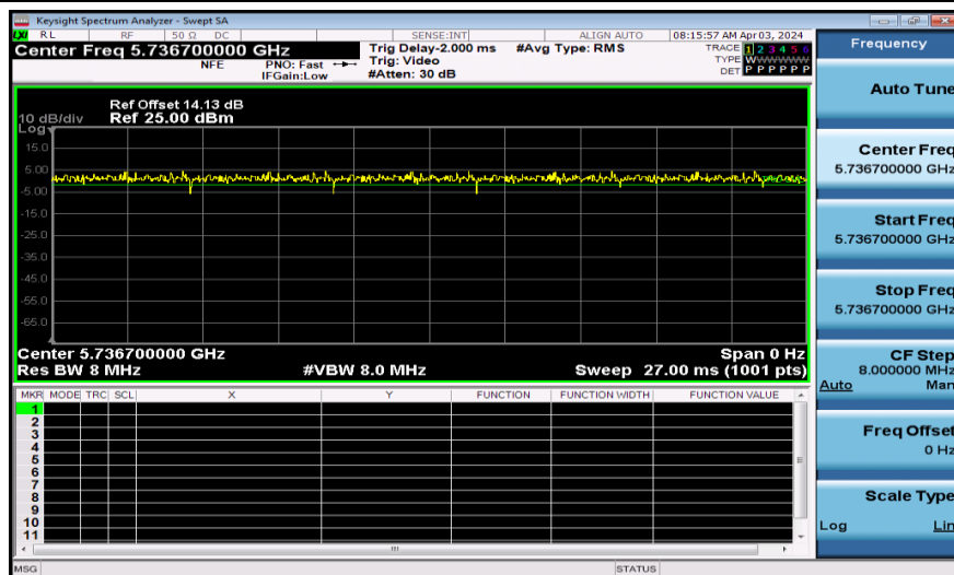
NTNV-11AX20SISO-Ant1-5745-26Tone
