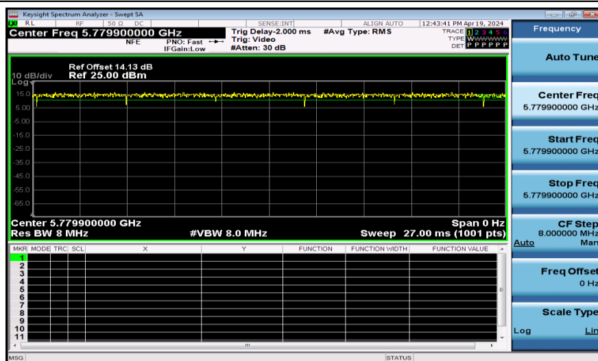
NTNV-11AX40SISO-Ant1-5795-52Tone
