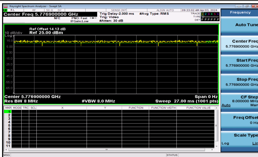
NTNV-11AX20SISO-Ant1-5785-26Tone
