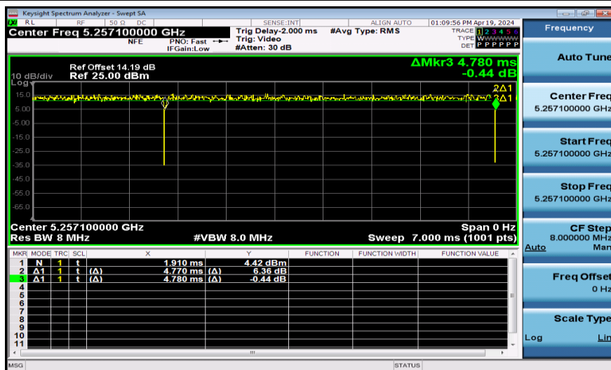
NTNV-11AX40SISO-Ant1-5270-106Tone
