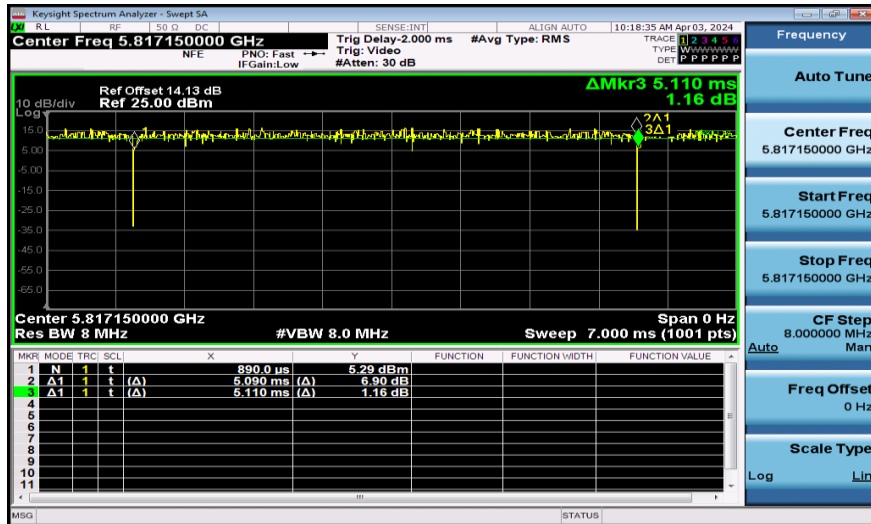
NTNV-11AX20SISO-Ant1-5825-26Tone
