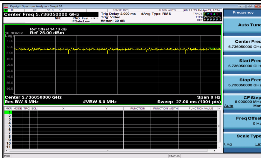
NTNV-11AX20SISO-Ant1-5745-52Tone
