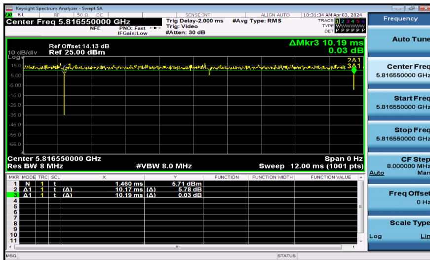
NTNV-11AX20SISO-Ant1-5825-52Tone
