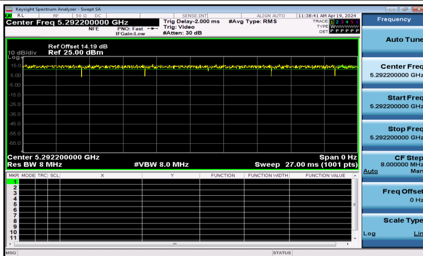
NTNV-11AX40SISO-Ant1-5310-52Tone
