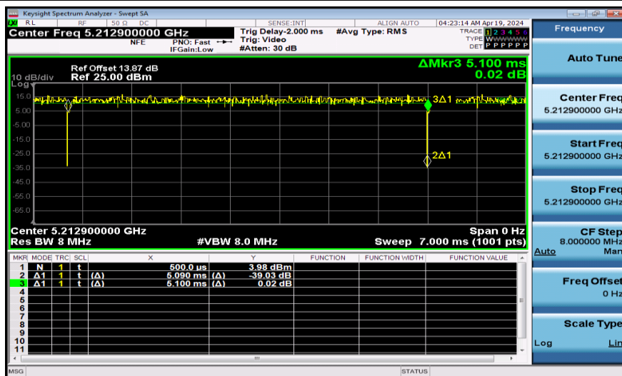
NTNV-11AX40SISO-Ant1-5230-26Tone
