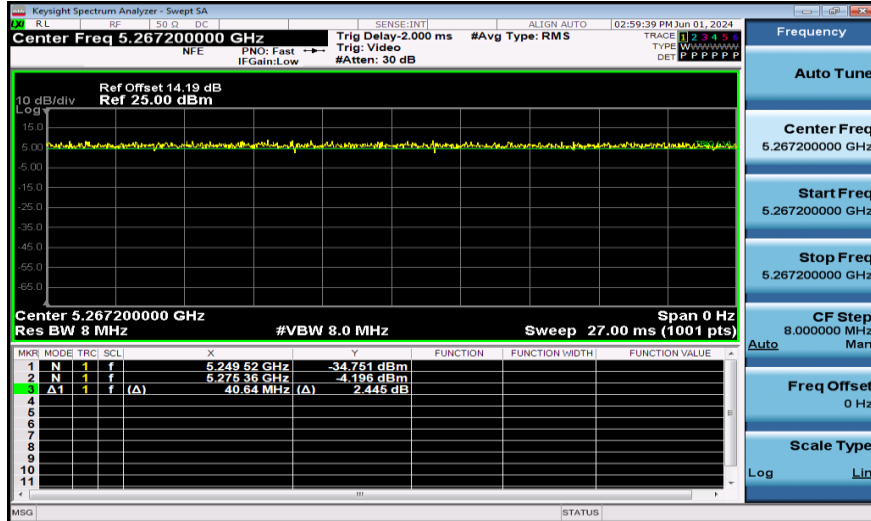
NTNV-11AX40SISO-Ant1-5270-484Tone
