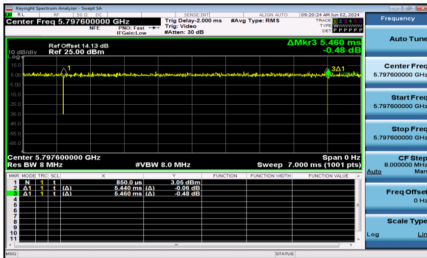
NTNV-11AX40SISO-Ant1-5795-484Tone
