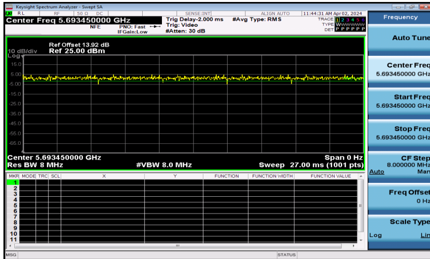
NTNV-11AX20SISO-Ant1-5700-52Tone
