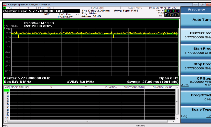
NTNV-11AX40SISO-Ant1-5795-26Tone
