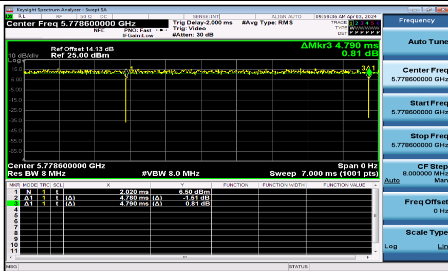
NTNV-11AX20SISO-Ant1-5785-106Tone
