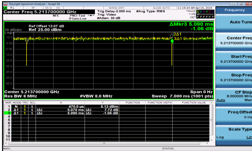
NTNV-11AX40SISO-Ant1-5230-52Tone
