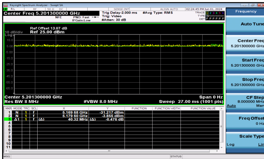
NTNV-11AX40SISO-Ant1-5190-484Tone
