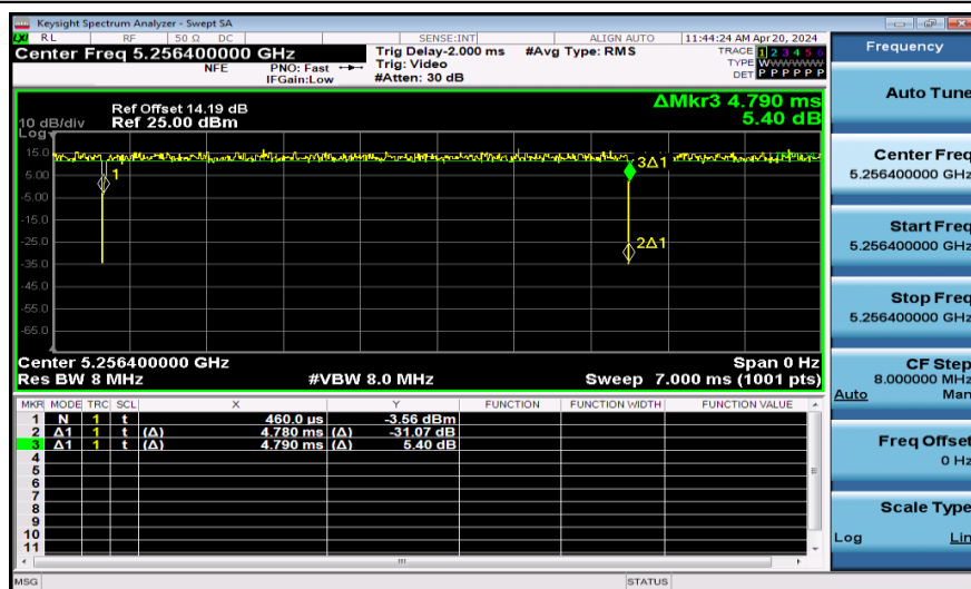
NTNV-11AX80SISO-Ant1-5290-106Tone
