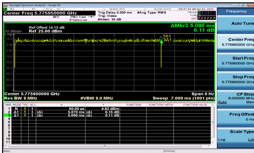
NTNV-11AX20SISO-Ant1-5785-52Tone
