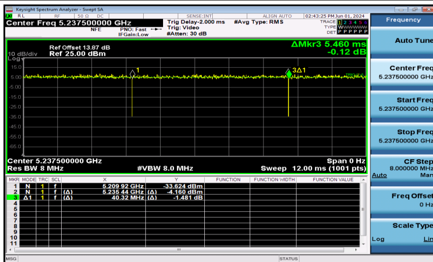
NTNV-11AX40SISO-Ant1-5230-484Tone
