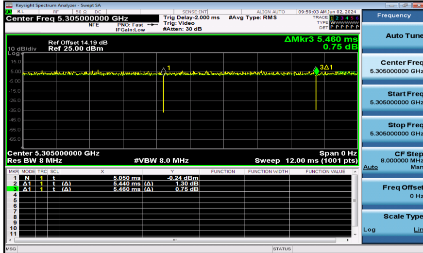
NTNV-11AX80SISO-Ant1-5290-484Tone
