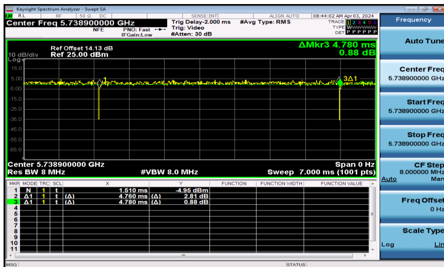
NTNV-11AX20SISO-Ant1-5745-106Tone
