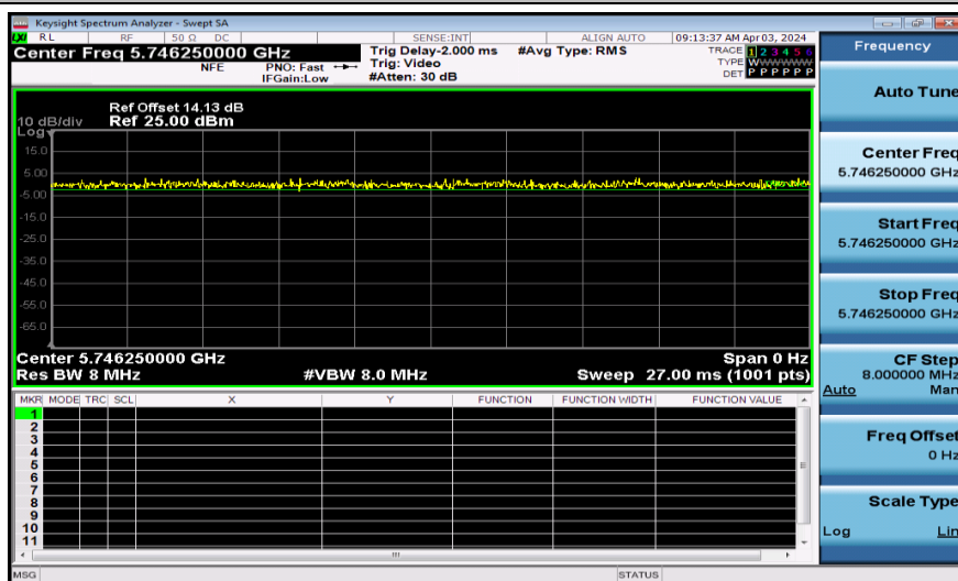
NTNV-11AX20SISO-Ant1-5745-242Tone
