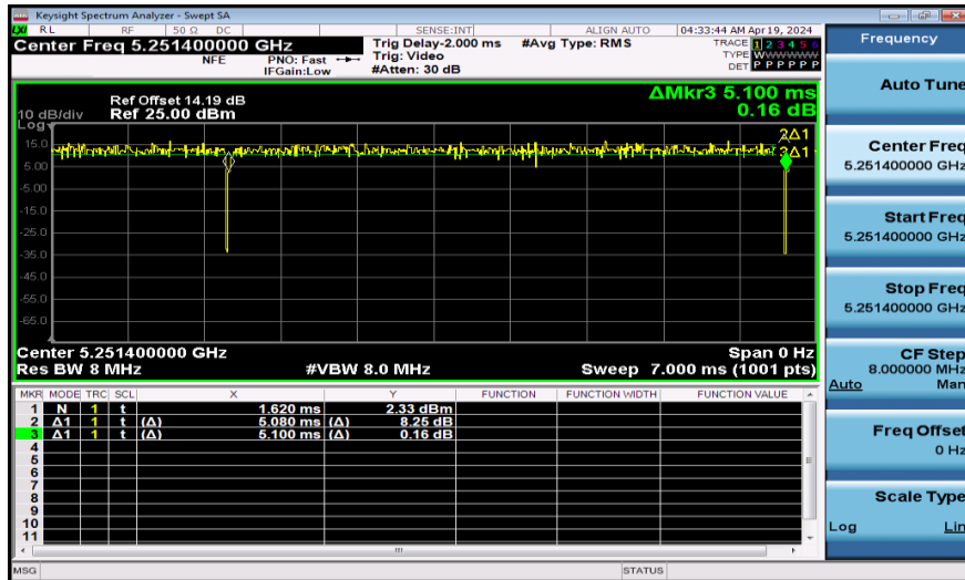
NTNV-11AX40SISO-Ant1-5270-26Tone
