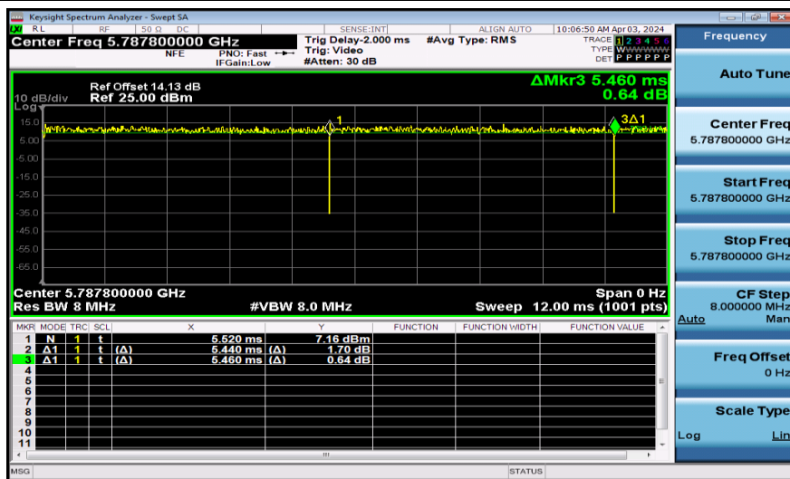
NTNV-11AX20SISO-Ant1-5785-242Tone
