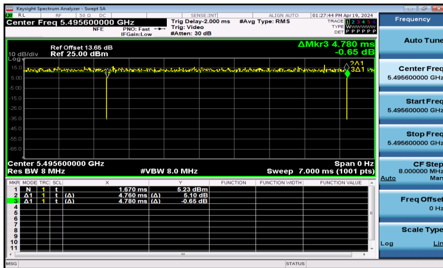
NTNV-11AX40SISO-Ant1-5510-106Tone
