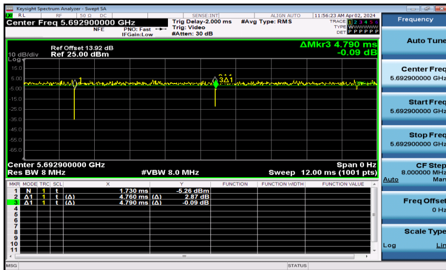
NTNV-11AX20SISO-Ant1-5700-106Tone
