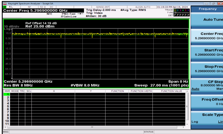
NTNV-11AX40SISO-Ant1-5310-106Tone
