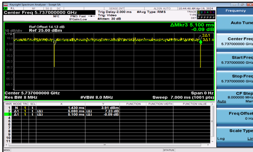
NTNV-11AX40SISO-Ant1-5755-26Tone
