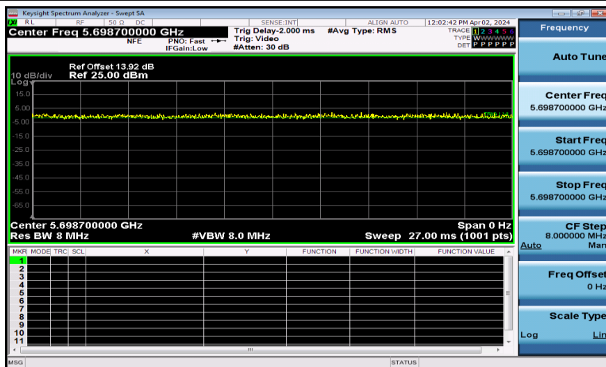
NTNV-11AX20SISO-Ant1-5700-242Tone
