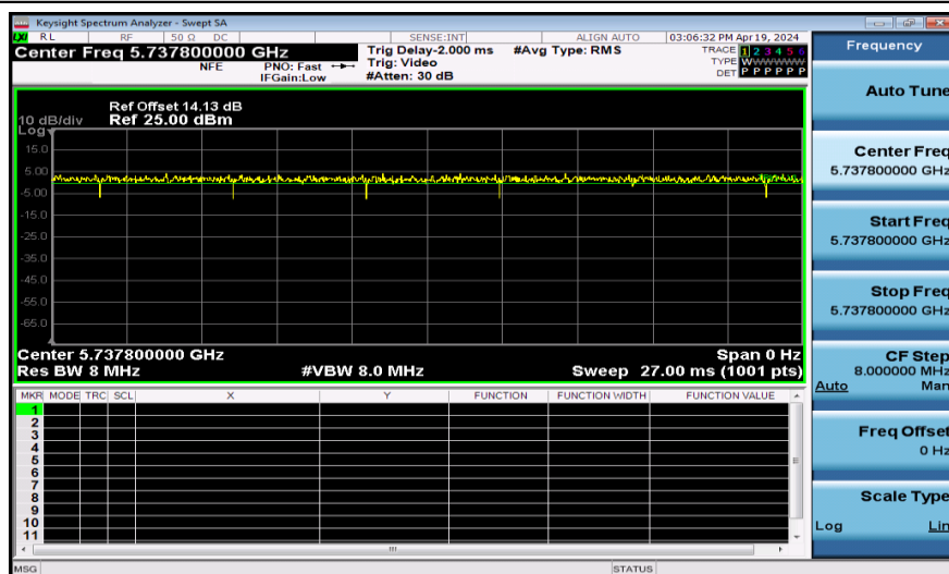
NTNV-11AX40SISO-Ant1-5755-106Tone
