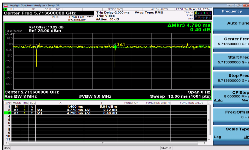
NTNV-11AX20SISO-Ant1-5720-106Tone
