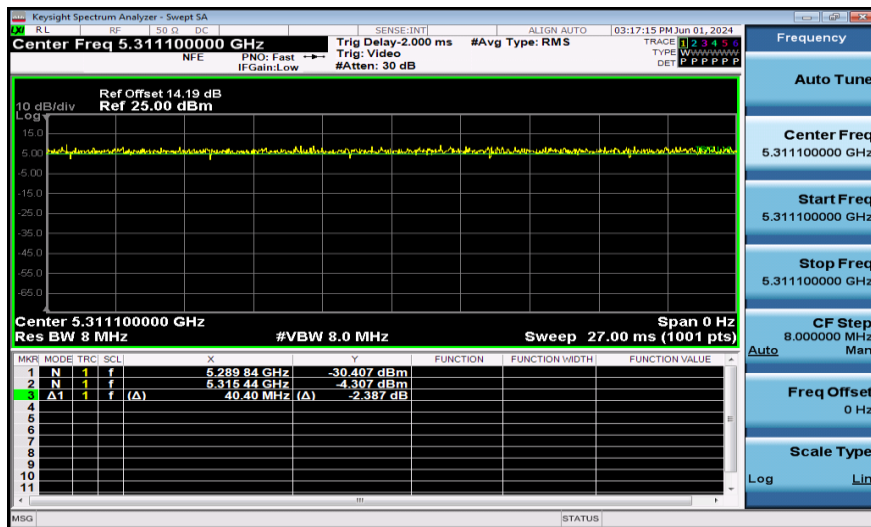
NTNV-11AX40SISO-Ant1-5310-484Tone
