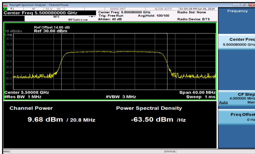
11AX20SISO-Ant1-5500-PASS
