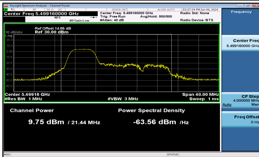
11AX20SISO-Ant1-5500-52Tone-PASS
