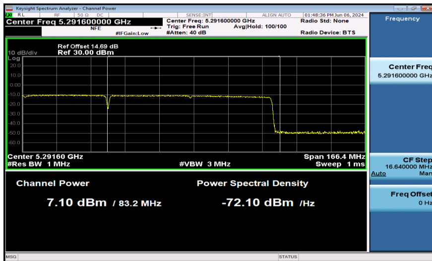
11AX160SISO-Ant1-5250_UNII-2A-PASS
