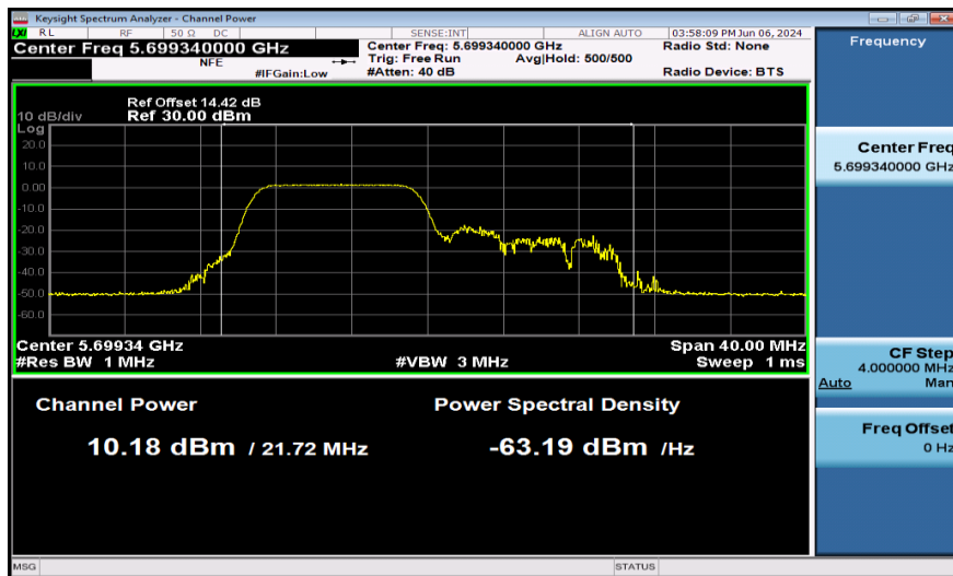
11AX20SISO-Ant1-5700-106Tone-PASS
