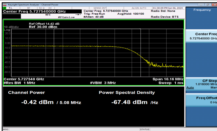
11AX40SISO-Ant1-5710_UNII-3-PASS
