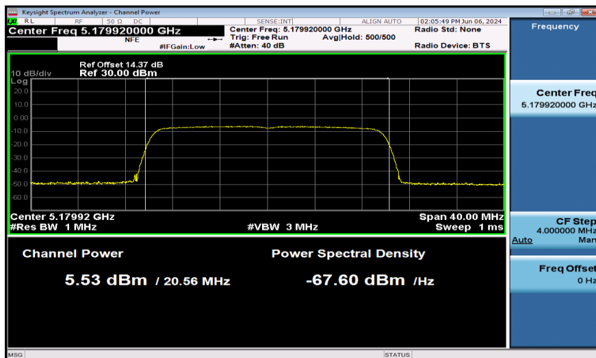
11AX20SISO-Ant1-5180-242Tone-PASS
