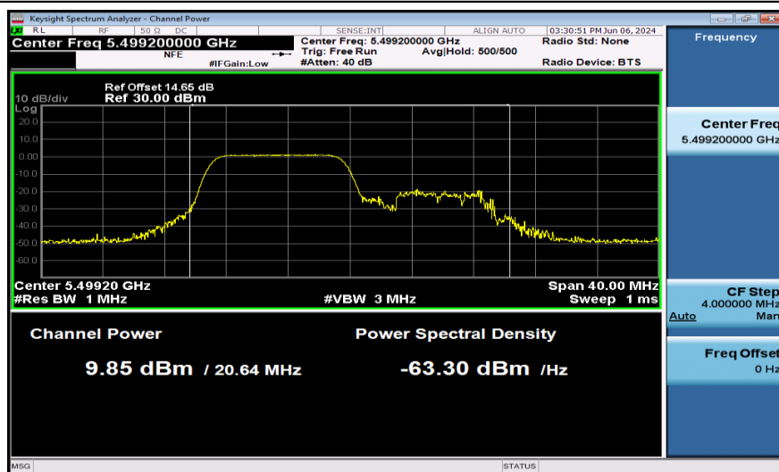
11AX20SISO-Ant1-5500-106Tone-PASS
