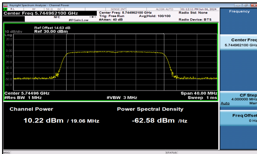
11AX20SISO-Ant1-5745-PASS
