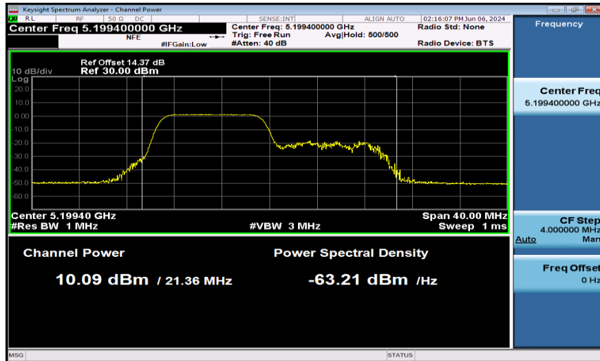
11AX20SISO-Ant1-5200-106Tone-PASS
