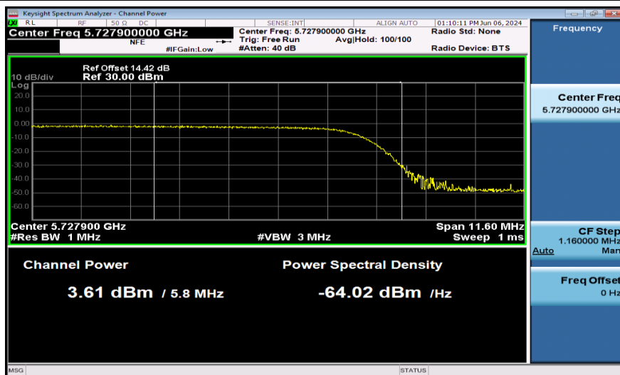
11AX20SISO-Ant1-5720_UNII-3-PASS
