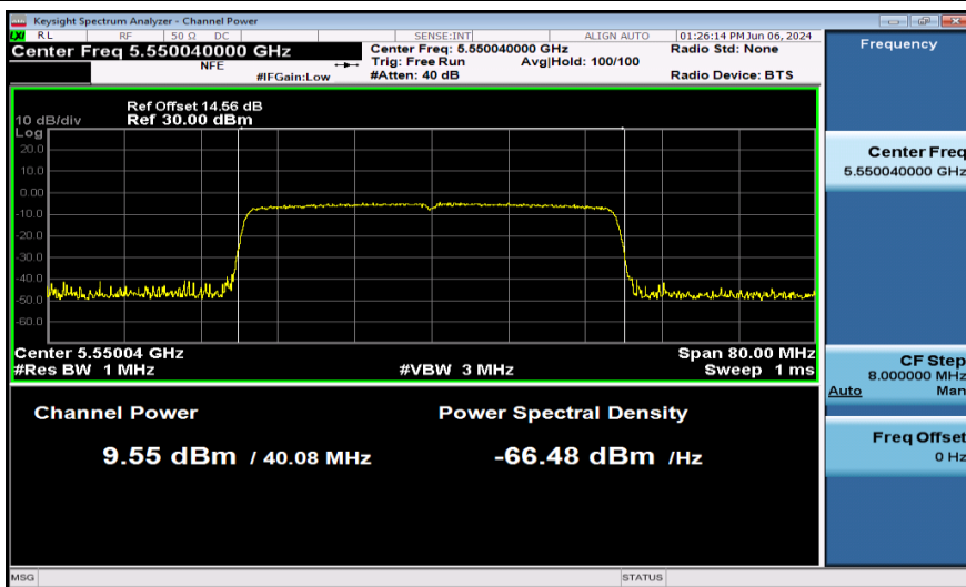
11AX40SISO-Ant1-5550-PASS
