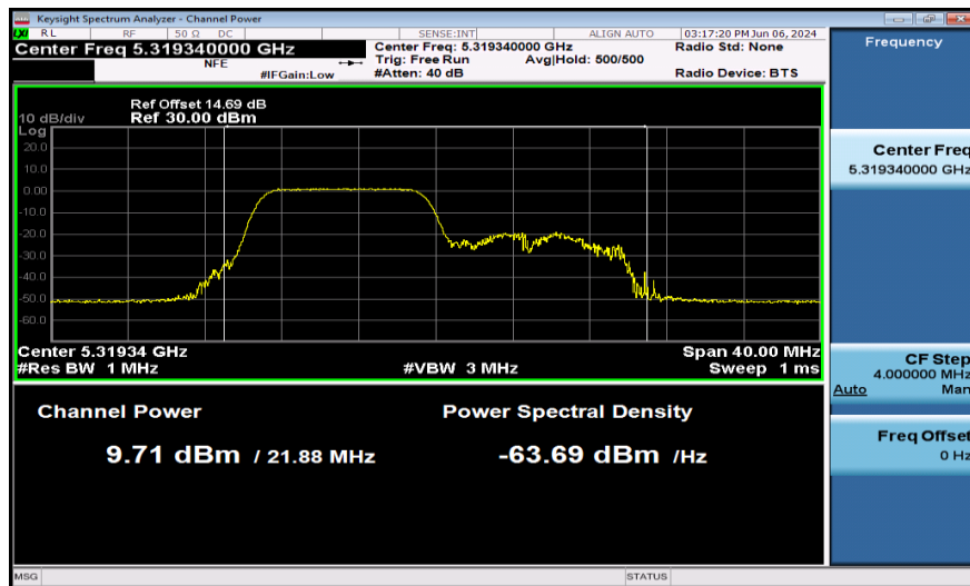
11AX20SISO-Ant1-5320-106Tone-PASS
