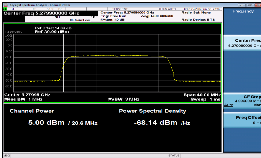
11AX20SISO-Ant1-5280-242Tone-PASS
