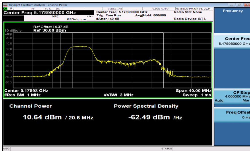
11AX20SISO-Ant1-5180-52Tone-PASS
