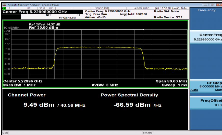
11AX40SISO-Ant1-5230-PASS
