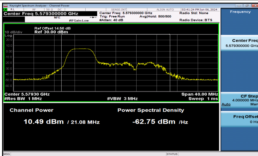
11AX20SISO-Ant1-5580-52Tone-PASS
