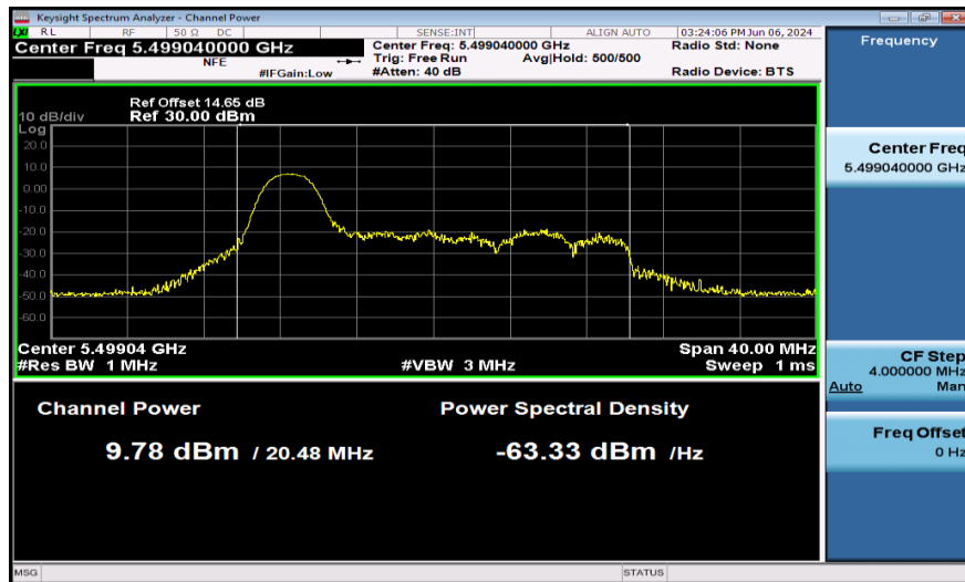
11AX20SISO-Ant1-5500-26Tone-PASS
