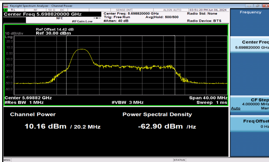
11AX20SISO-Ant1-5700-26Tone-PASS
