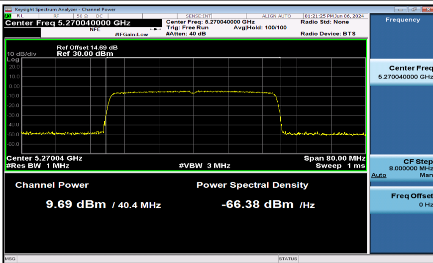
11AX40SISO-Ant1-5270-PASS
