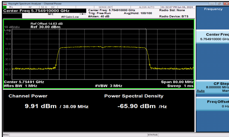
11AX40SISO-Ant1-5755-PASS
