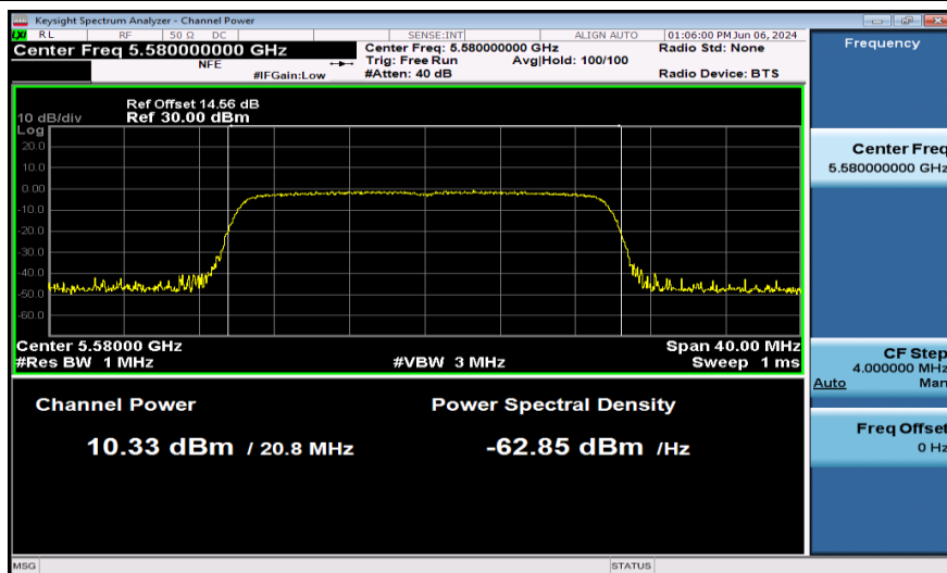
11AX20SISO-Ant1-5580-PASS
