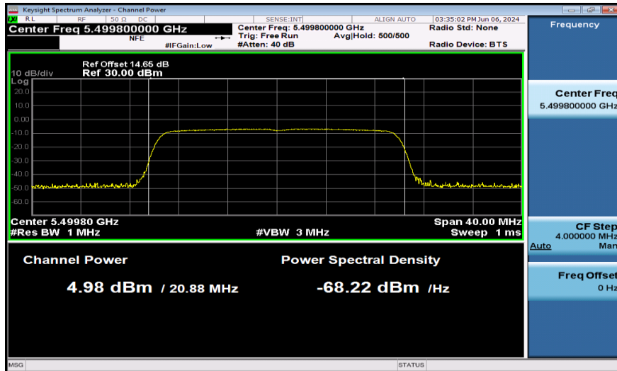
11AX20SISO-Ant1-5500-242Tone-PASS
