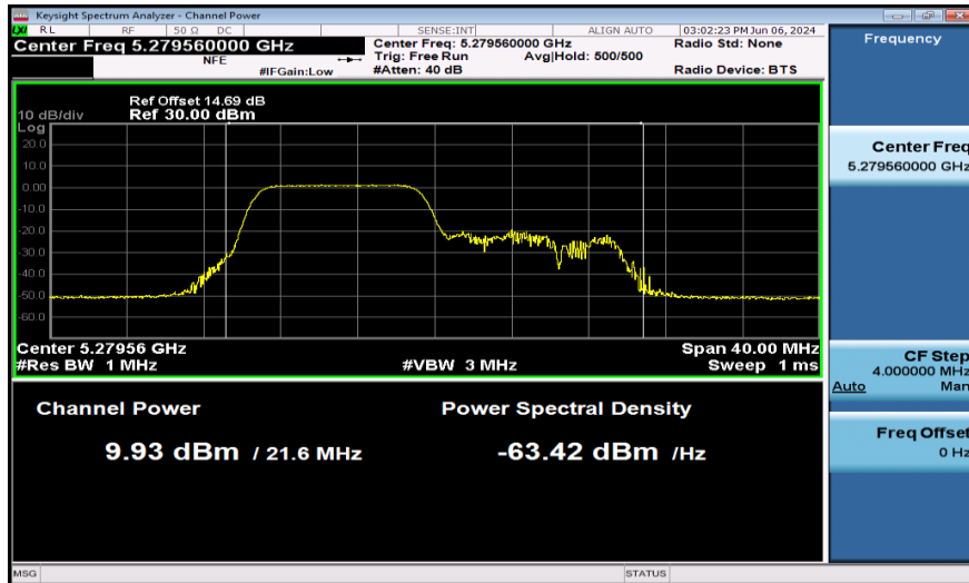
11AX20SISO-Ant1-5280-106Tone-PASS
