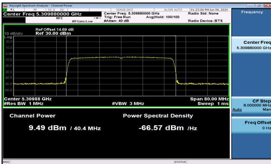
11AX40SISO-Ant1-5310-PASS
