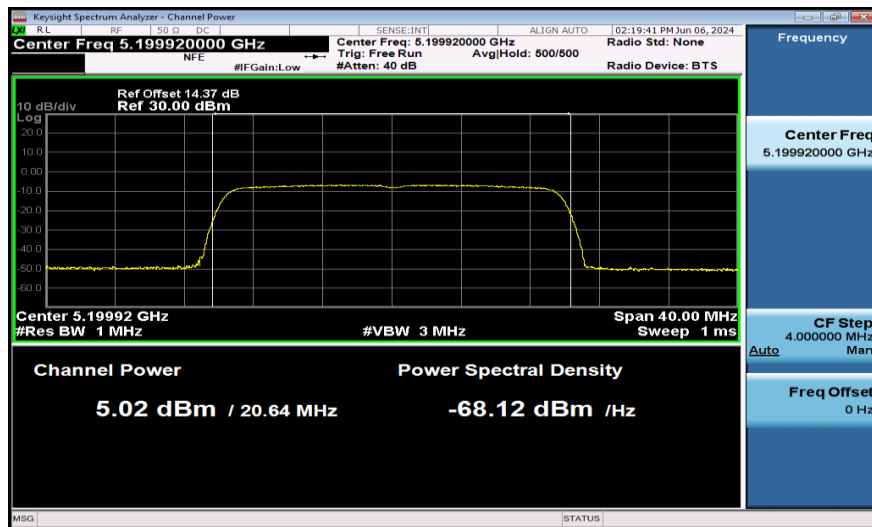
11AX20SISO-Ant1-5200-242Tone-PASS
