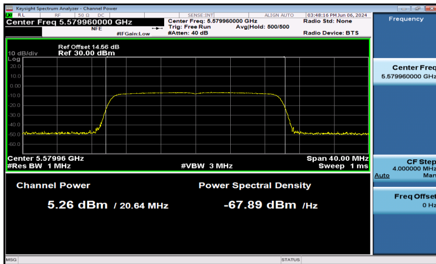
11AX20SISO-Ant1-5580-242Tone-PASS
