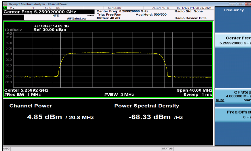
11AX20SISO-Ant1-5260-242Tone-PASS
