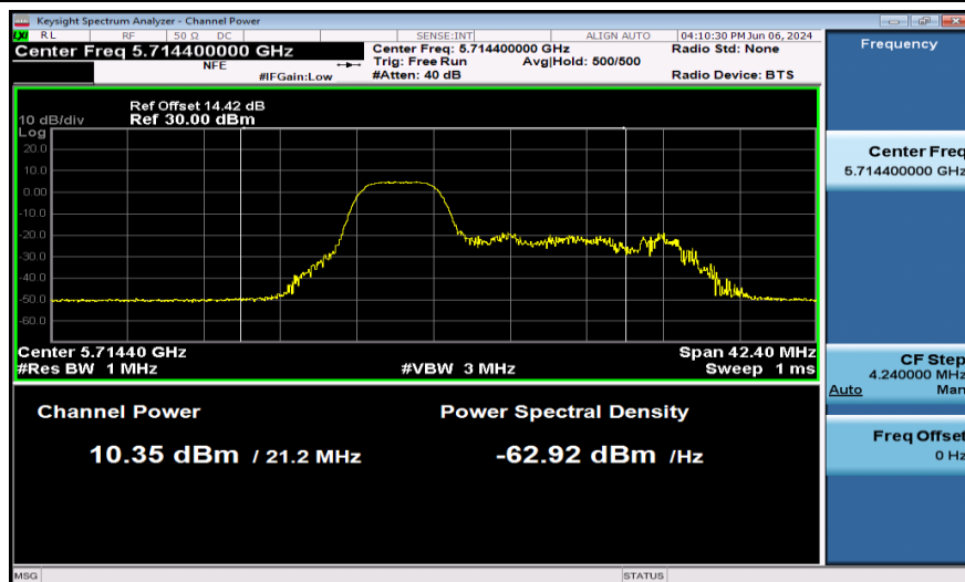
11AX20SISO-Ant1-5720_UNII-2C-52Tone-PASS
