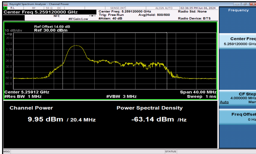
11AX20SISO-Ant1-5260-26Tone-PASS
