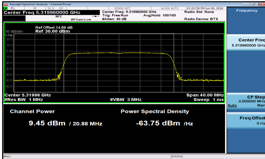
11AX20SISO-Ant1-5320-PASS
