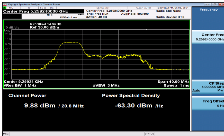
11AX20SISO-Ant1-5260-52Tone-PASS
