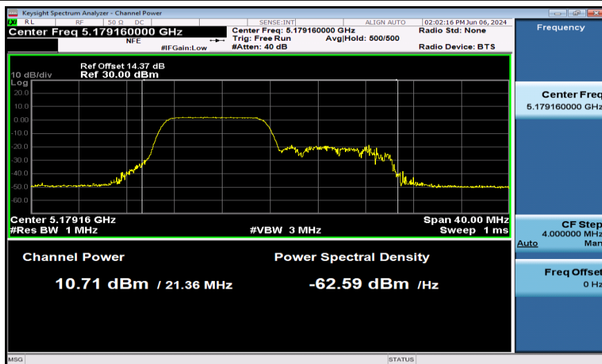
11AX20SISO-Ant1-5180-106Tone-PASS
