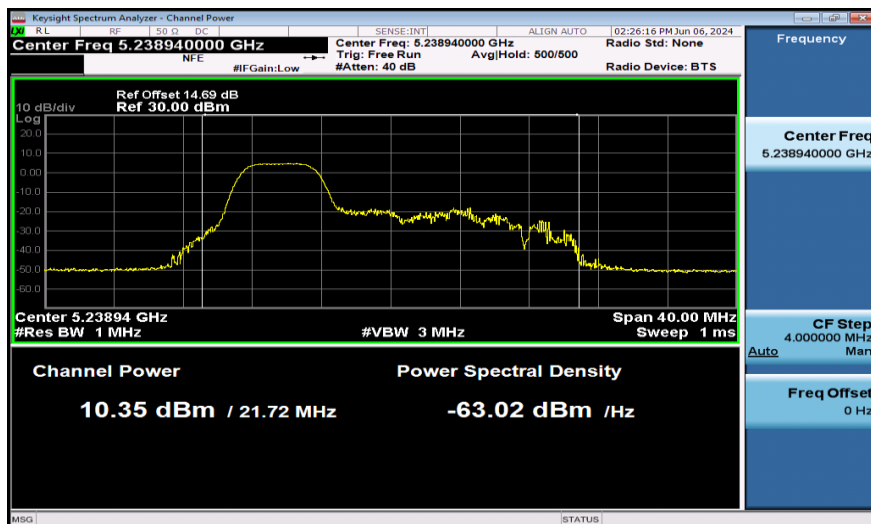
11AX20SISO-Ant1-5240-52Tone-PASS
