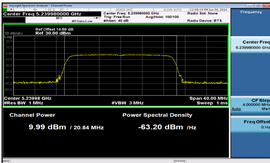
11AX20SISO-Ant1-5240-PASS
