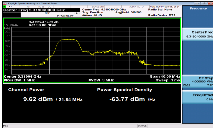
11AX20SISO-Ant1-5320-52Tone-PASS
