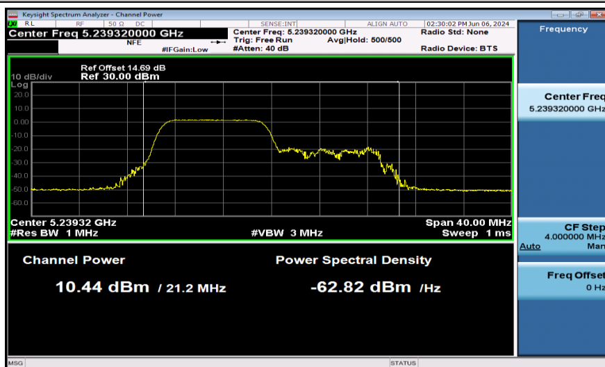
11AX20SISO-Ant1-5240-106Tone-PASS
