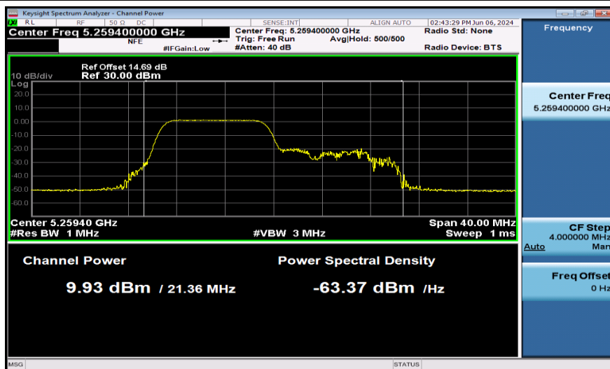
11AX20SISO-Ant1-5260-106Tone-PASS
