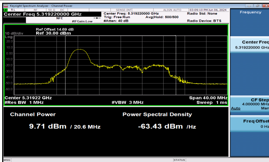
11AX20SISO-Ant1-5320-26Tone-PASS
