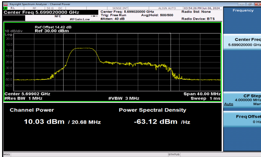
11AX20SISO-Ant1-5700-52Tone-PASS
