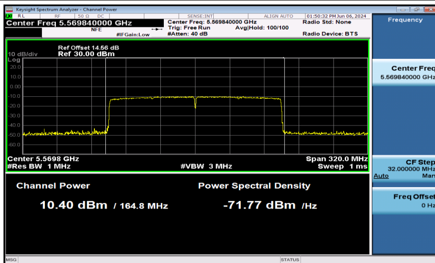
11AX160SISO-Ant1-5570-PASS
