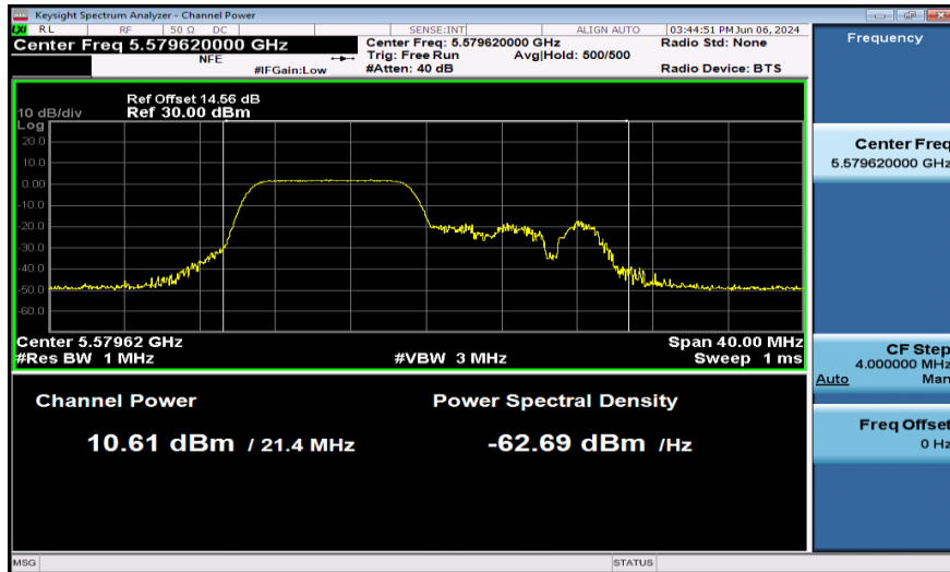
11AX20SISO-Ant1-5580-106Tone-PASS
