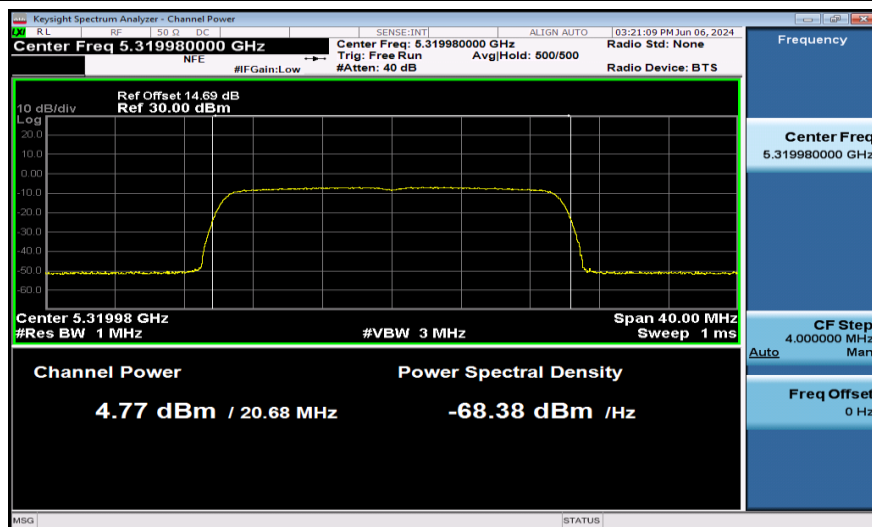
11AX20SISO-Ant1-5320-242Tone-PASS
