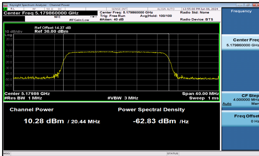
11AX20SISO-Ant1-5180-PASS
