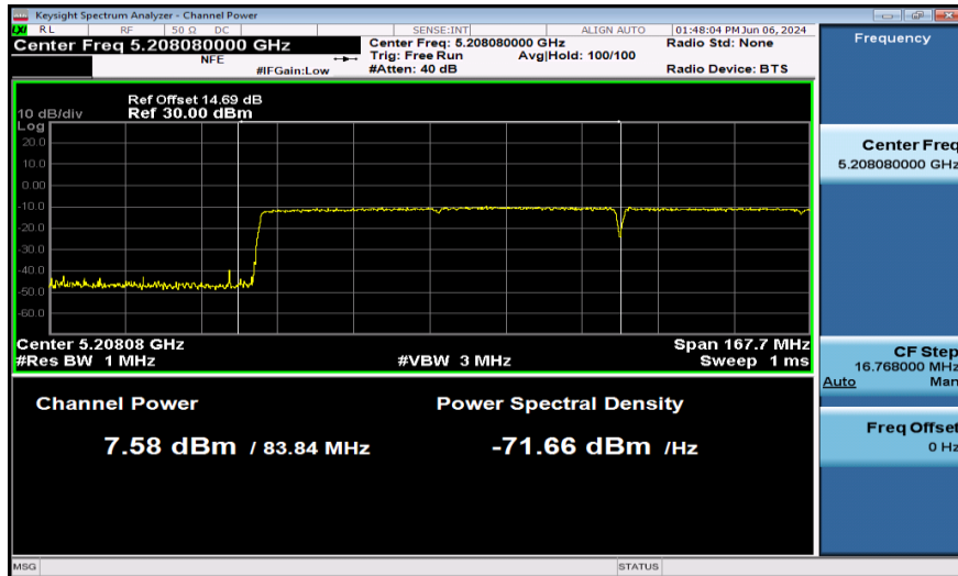
11AX160SISO-Ant1-5250_UNII-1-PASS
