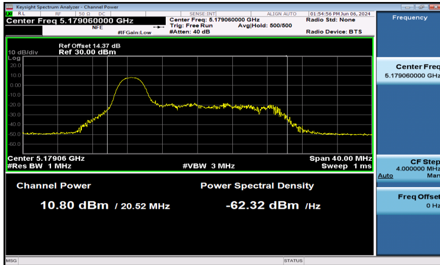
11AX20SISO-Ant1-5180-26Tone-PASS
