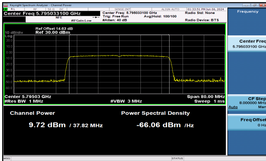
11AX40SISO-Ant1-5795-PASS
