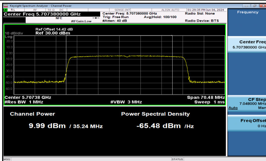
11AX40SISO-Ant1-5710_PASS
