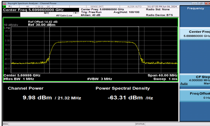
11AX20SISO-Ant1-5700-PASS
