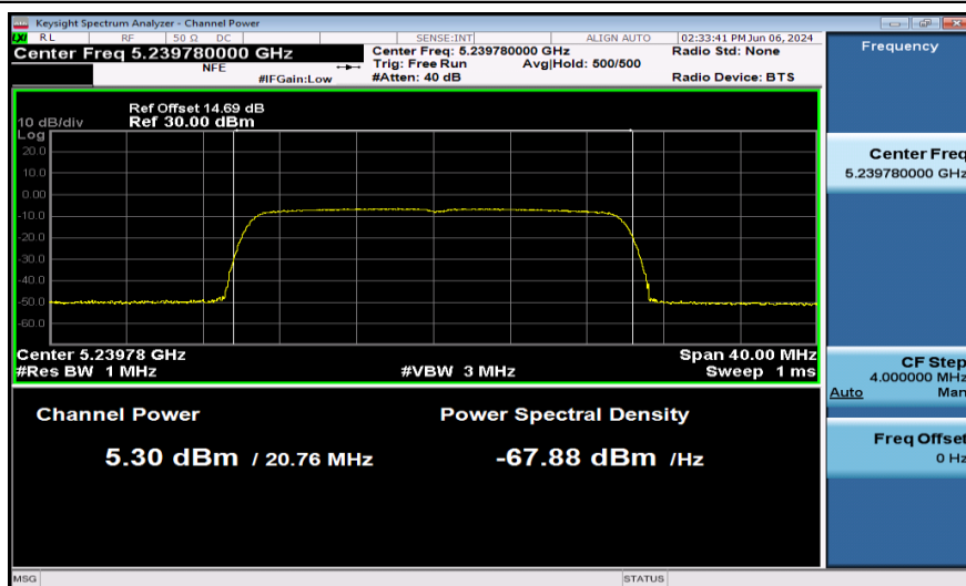
11AX20SISO-Ant1-5240-242Tone-PASS
