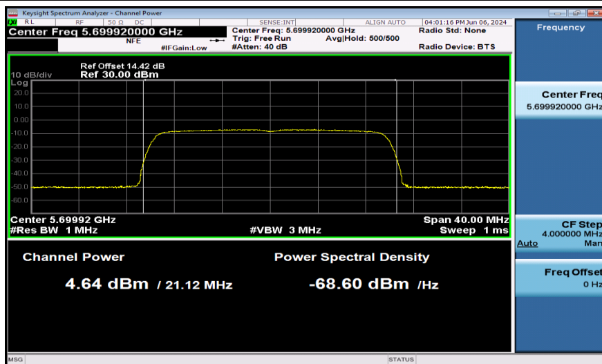
11AX20SISO-Ant1-5700-242Tone-PASS
