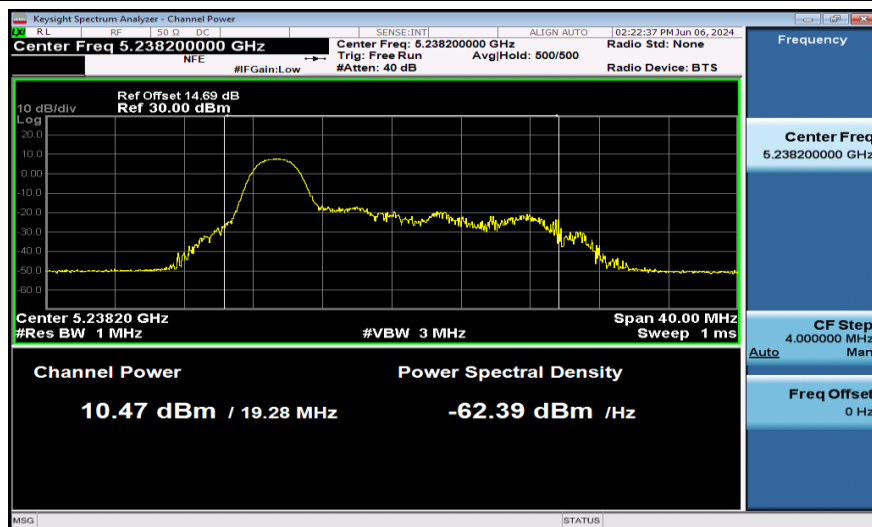
11AX20SISO-Ant1-5240-26Tone-PASS
