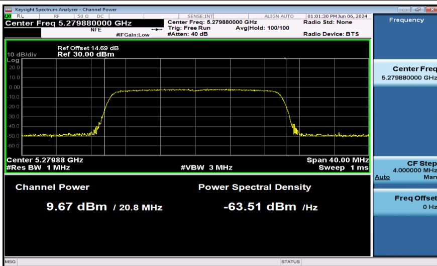
11AX20SISO-Ant1-5280-PASS
