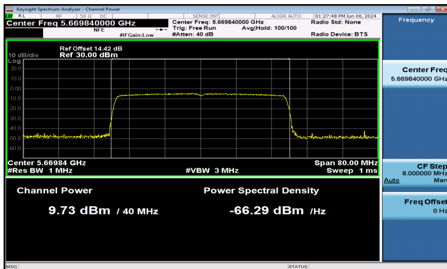
11AX40SISO-Ant1-5670-PASS
