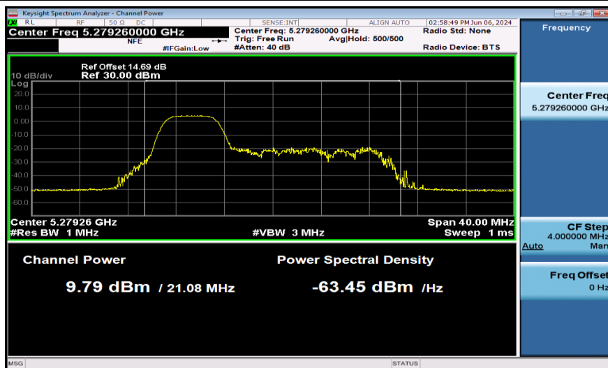
11AX20SISO-Ant1-5280-52Tone-PASS
