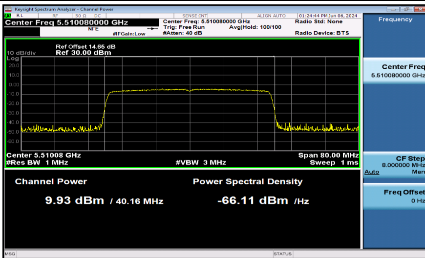
11AX40SISO-Ant1-5510-PASS
