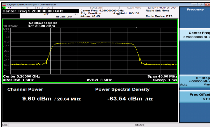
11AX20SISO-Ant1-5260-PASS
