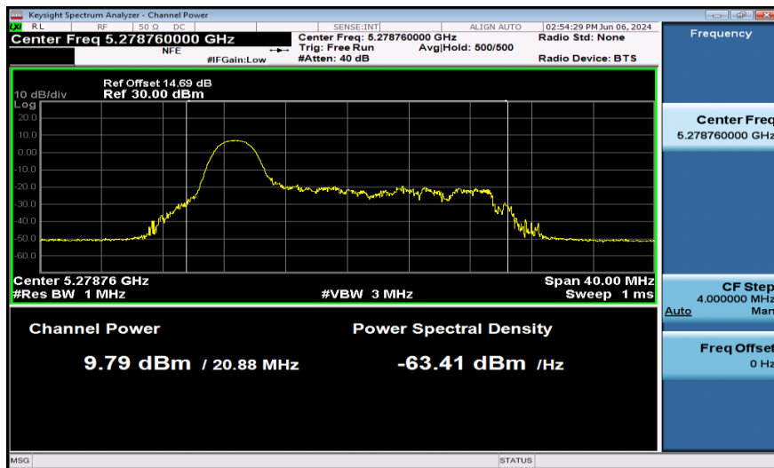
11AX20SISO-Ant1-5280-26Tone-PASS
