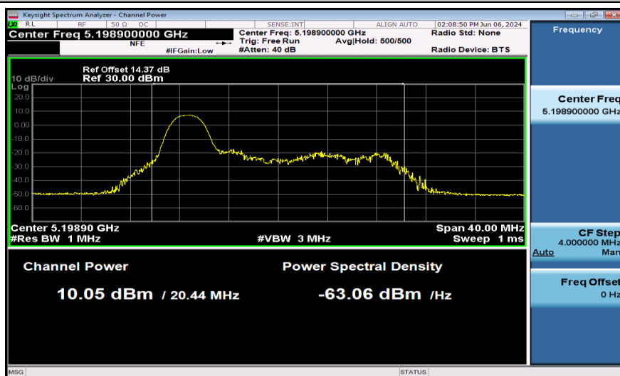
11AX20SISO-Ant1-5200-26Tone-PASS
