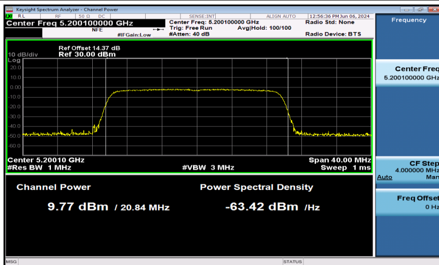
11AX20SISO-Ant1-5200-PASS
