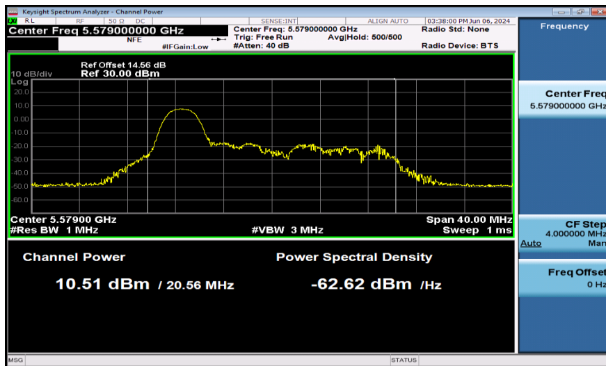
11AX20SISO-Ant1-5580-26Tone-PASS
