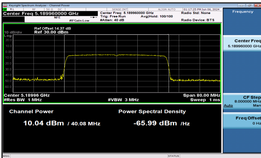
11AX40SISO-Ant1-5190-PASS
