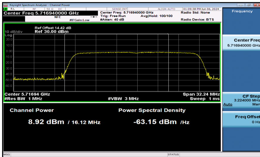
11AX20SISO-Ant1-5720_UNII-2C-PASS
