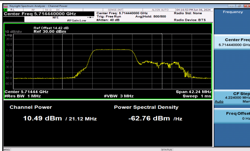
11AX20SISO-Ant1-5720_UNII-2C-106Tone-PASS
