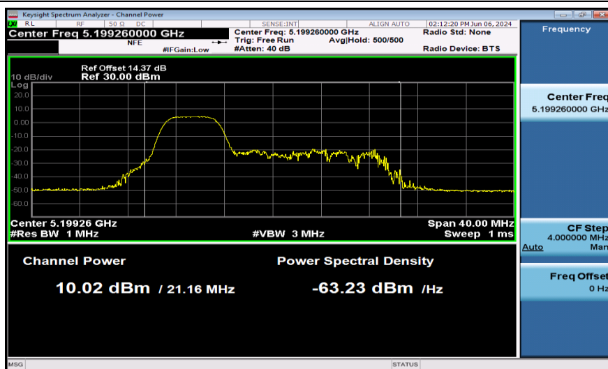
11AX20SISO-Ant1-5200-52Tone-PASS
