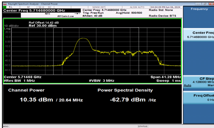
11AX20SISO-Ant1-5720_UNII-2C-26Tone-PASS
