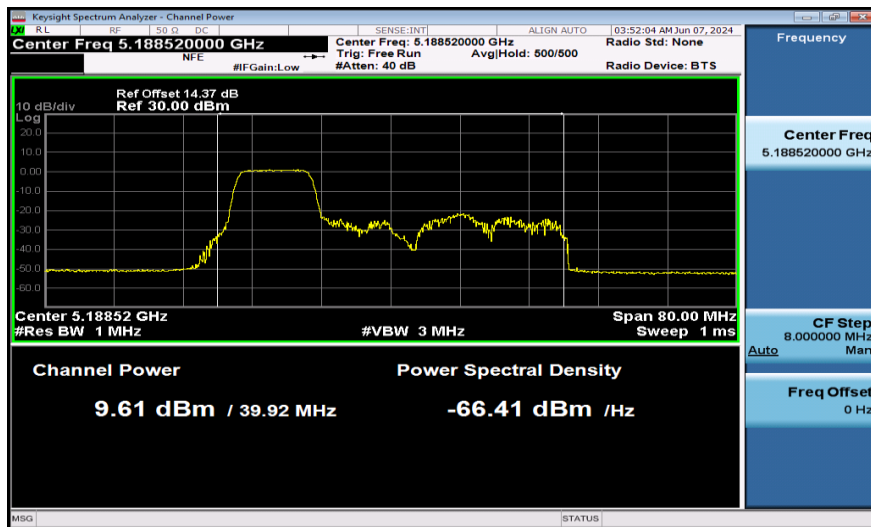
11AX40SISO-Ant1-5190-106Tone-PASS
