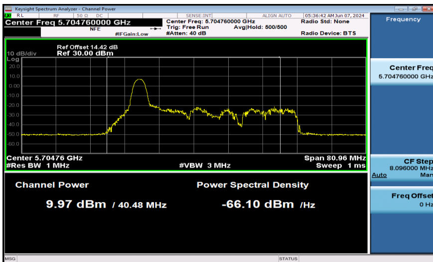
11AX40SISO-Ant1-5710_UNII-2C-26Tone-PASS
