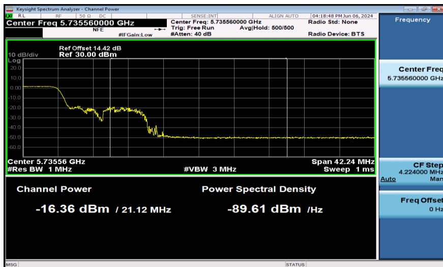
11AX20SISO-Ant1-5720_UNII-3-106Tone-PASS
