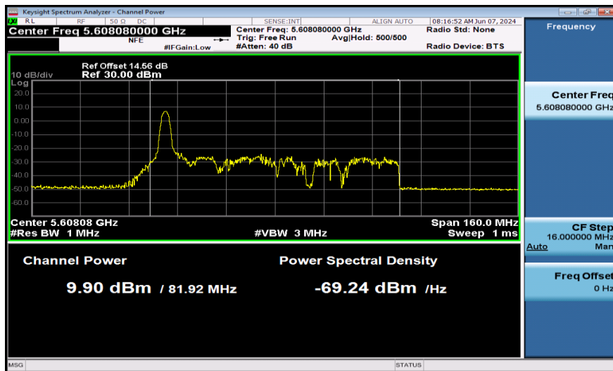
11AX80SISO-Ant1-5610-26Tone-PASS
