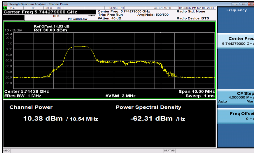
11AX20SISO-Ant1-5745-52Tone-PASS
