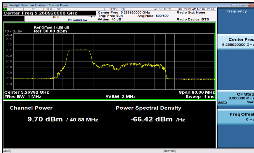
11AX40SISO-Ant1-5270-106Tone-PASS
