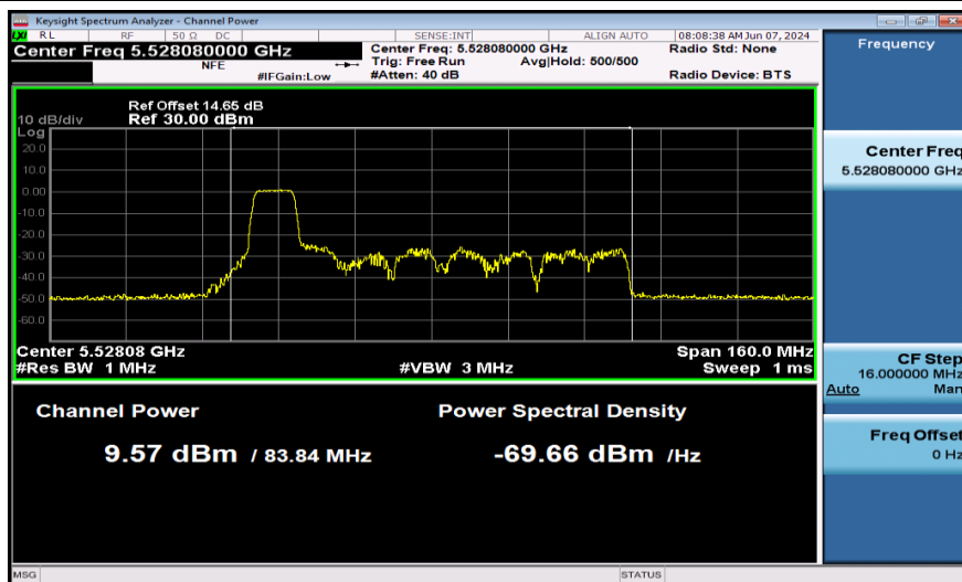
11AX80SISO-Ant1-5530-106Tone-PASS
