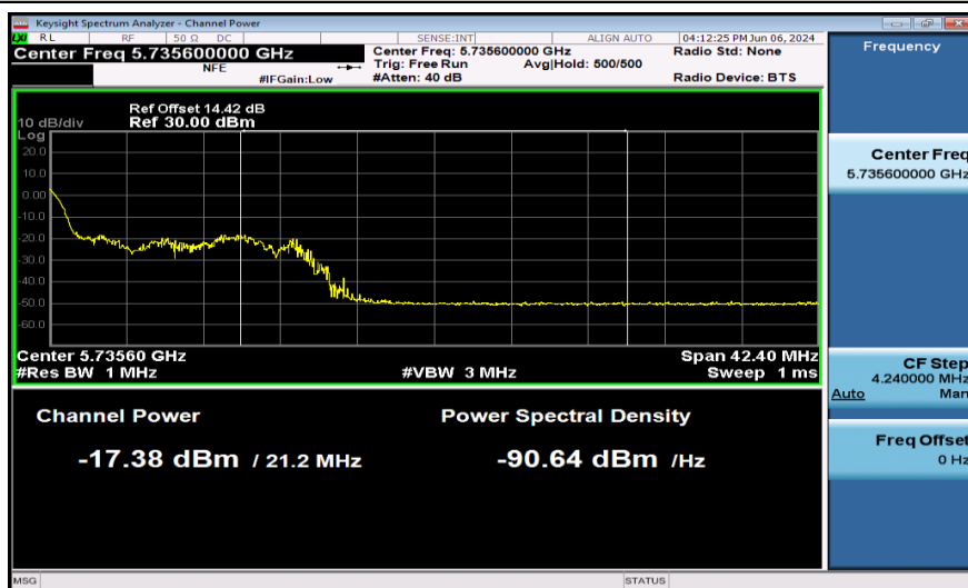
11AX20SISO-Ant1-5720_UNII-3-52Tone-PASS
