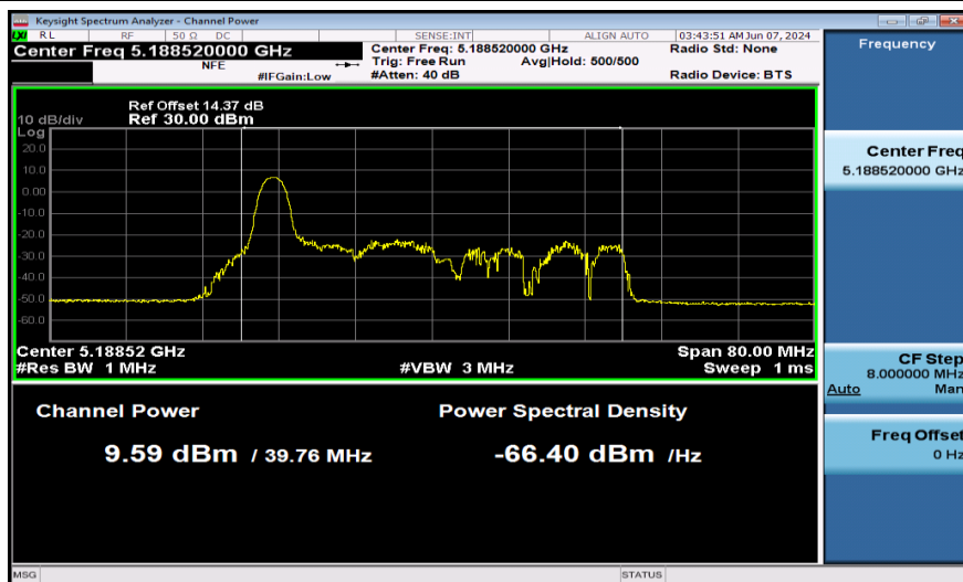
11AX40SISO-Ant1-5190-26Tone-PASS
