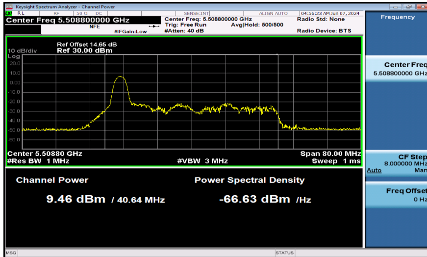
11AX40SISO-Ant1-5510-26Tone-PASS
