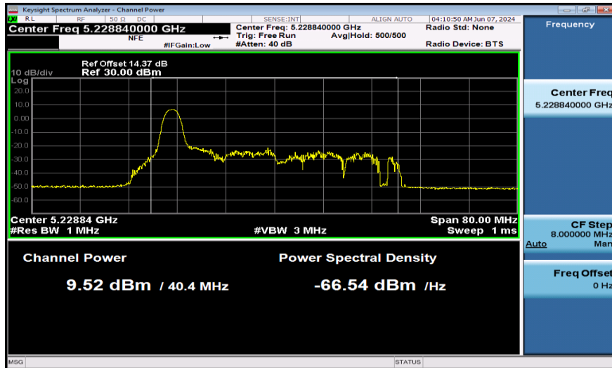
11AX40SISO-Ant1-5230-26Tone-PASS
