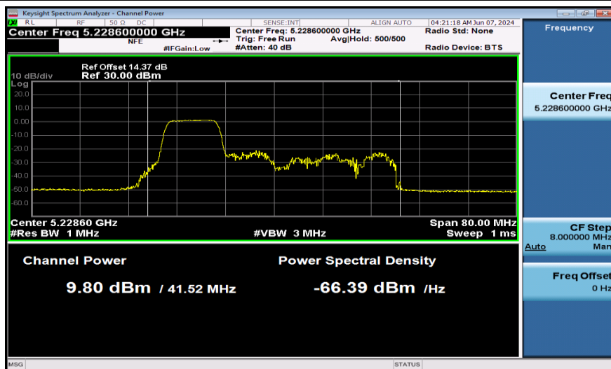
11AX40SISO-Ant1-5230-106Tone-PASS
