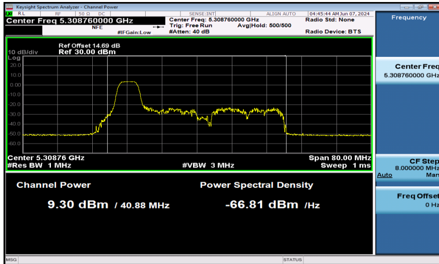
11AX40SISO-Ant1-5310-52Tone-PASS
