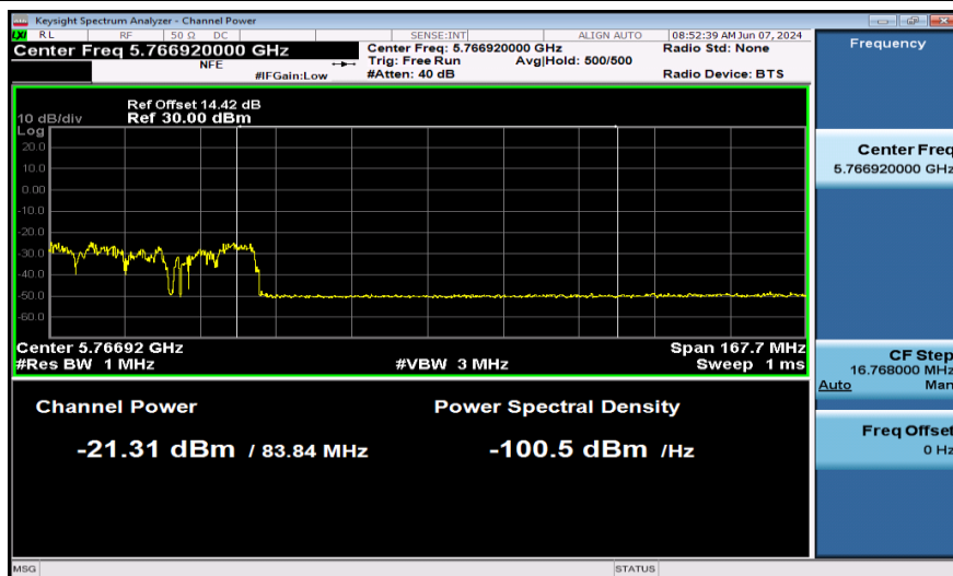
11AX80SISO-Ant1-5690_UNII-3-106Tone-PASS
