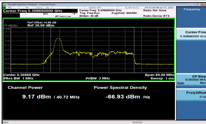
11AX40SISO-Ant1-5310-26Tone-PASS
