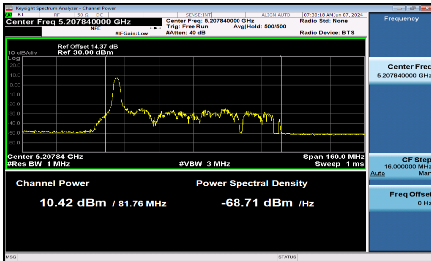
11AX80SISO-Ant1-5210-26Tone-PASS
