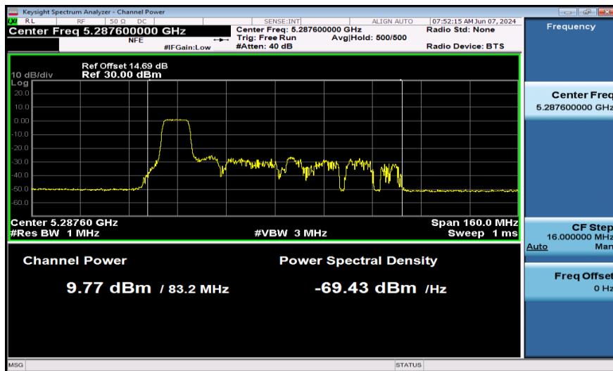
11AX80SISO-Ant1-5290-106Tone-PASS
