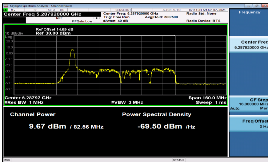
11AX80SISO-Ant1-5290-26Tone-PASS
