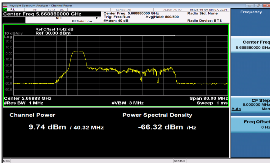
11AX40SISO-Ant1-5670-52Tone-PASS
