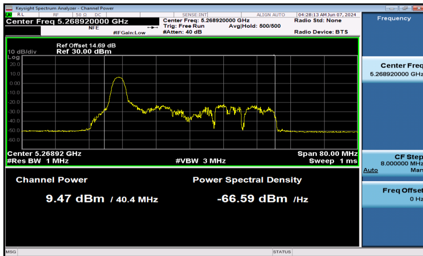
11AX40SISO-Ant1-5270-26Tone-PASS
