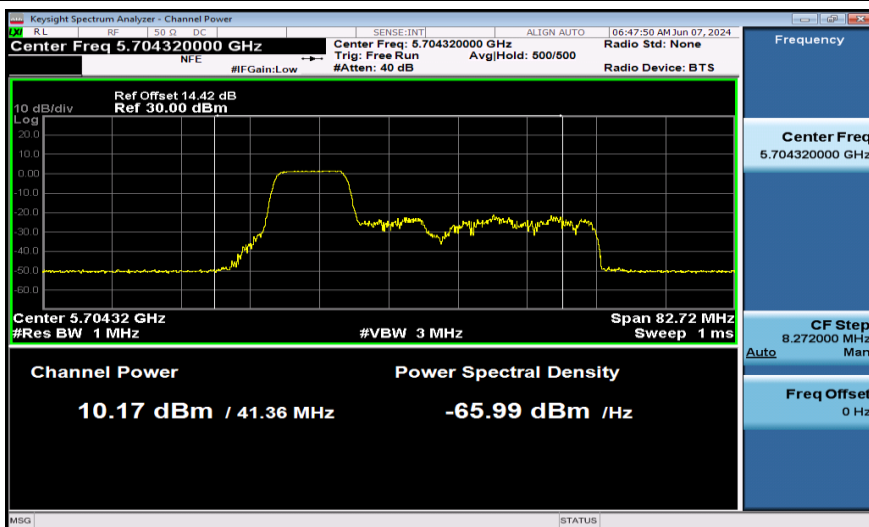
11AX40SISO-Ant1-5710_UNII-2C-106Tone-PASS
