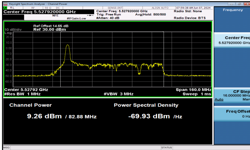
11AX80SISO-Ant1-5530-26Tone-PASS
