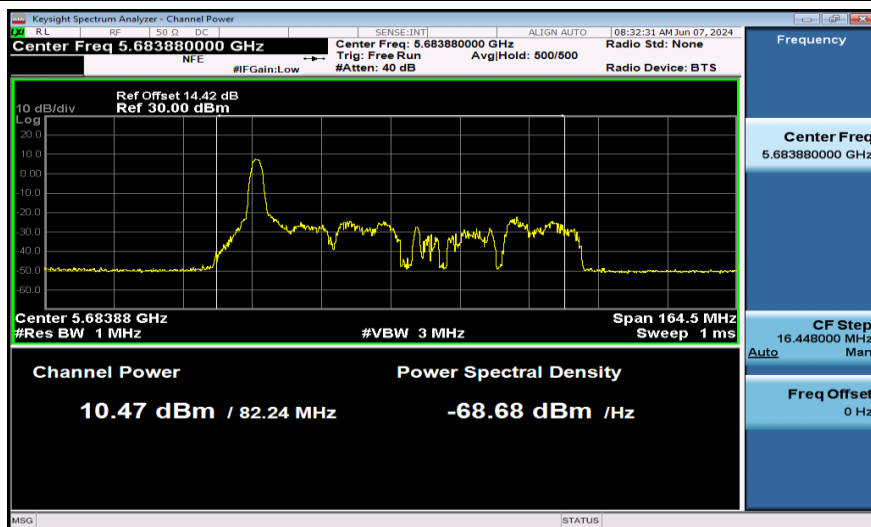
11AX80SISO-Ant1-5690_UNII-2C-26Tone-PASS
