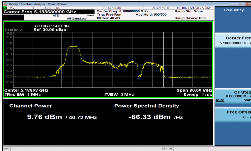
11AX40SISO-Ant1-5190-52Tone-PASS
