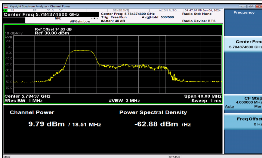
11AX20SISO-Ant1-5785-52Tone-PASS
