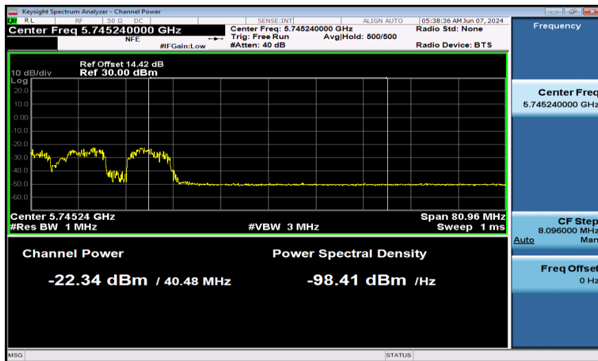
11AX40SISO-Ant1-5710_UNII-3-26Tone-PASS
