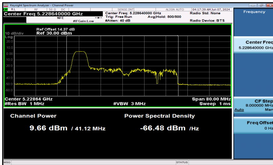
11AX40SISO-Ant1-5230-52Tone-PASS
