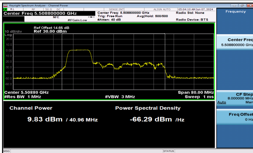
11AX40SISO-Ant1-5510-106Tone-PASS
