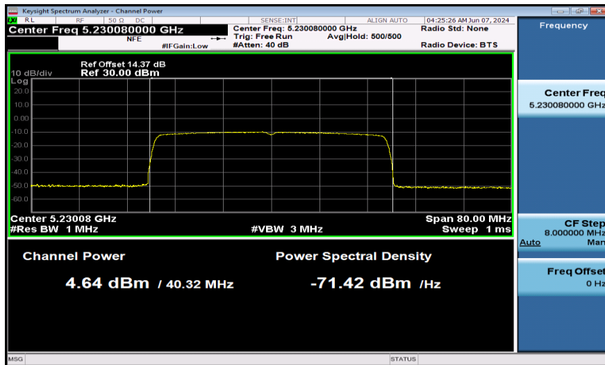
11AX40SISO-Ant1-5230-484Tone-PASS
