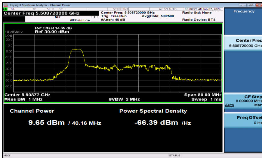
11AX40SISO-Ant1-5510-52Tone-PASS
