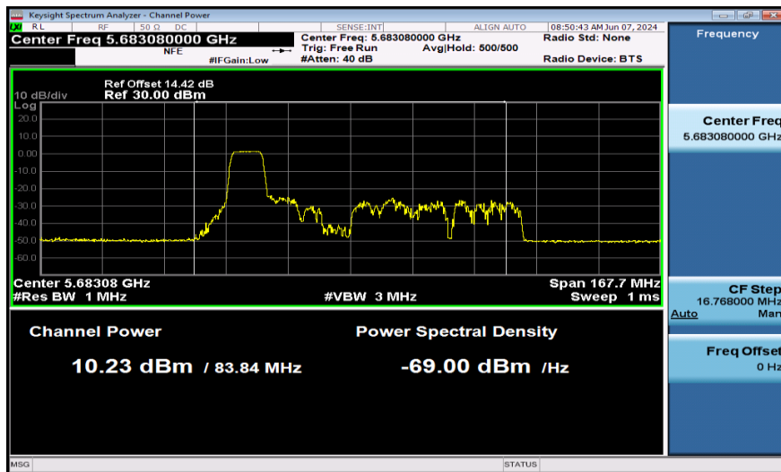
11AX80SISO-Ant1-5690_UNII-2C-106Tone-PASS
