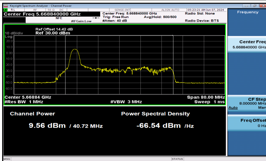
11AX40SISO-Ant1-5670-26Tone-PASS
