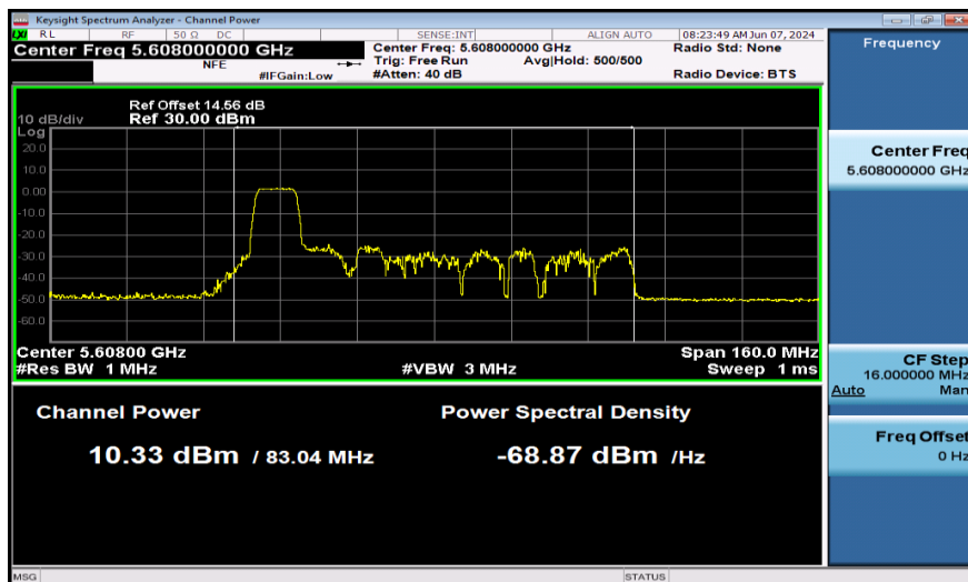
11AX80SISO-Ant1-5610-106Tone-PASS
