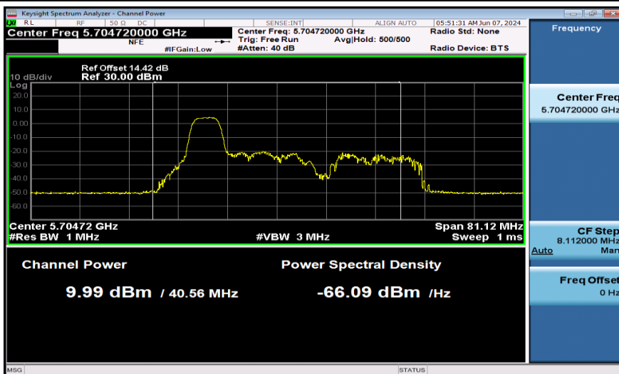
11AX40SISO-Ant1-5710_UNII-2C-52Tone-PASS
