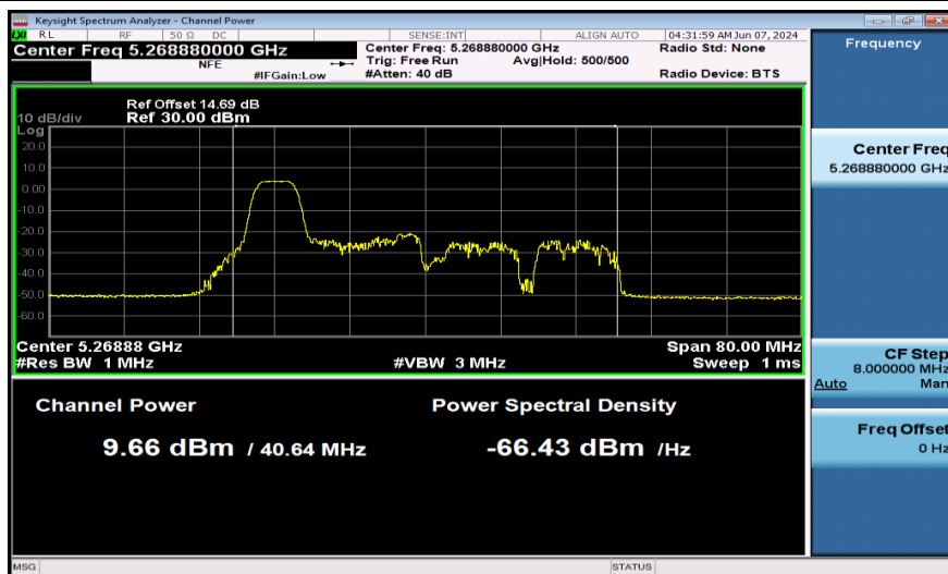
11AX40SISO-Ant1-5270-52Tone-PASS
