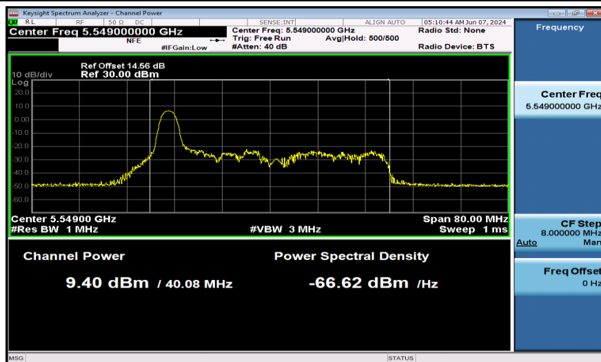
11AX40SISO-Ant1-5550-26Tone-PASS
