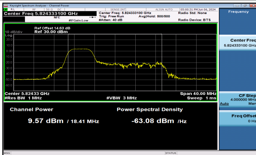
11AX20SISO-Ant1-5825-52Tone-PASS
