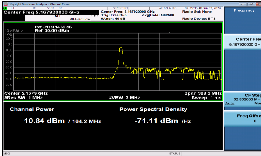
11AX160SISO-Ant1-5250_UNII-1-52Tone-PASS
