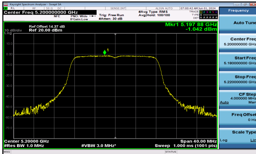
11A-Ant1-5200-PASS
