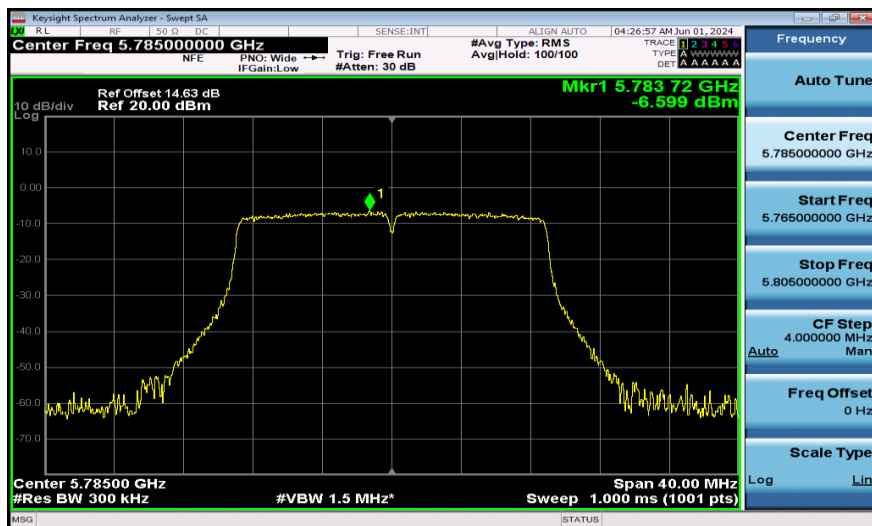
11AC20SISO-Ant1-5785-PASS
