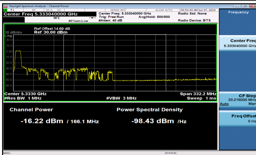
11AX160SISO-Ant1-5250_UNII-2A-106Tone-PASS
