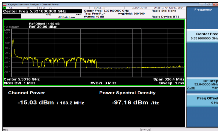
11AX160SISO-Ant1-5250_UNII-2A-26Tone-PASS
