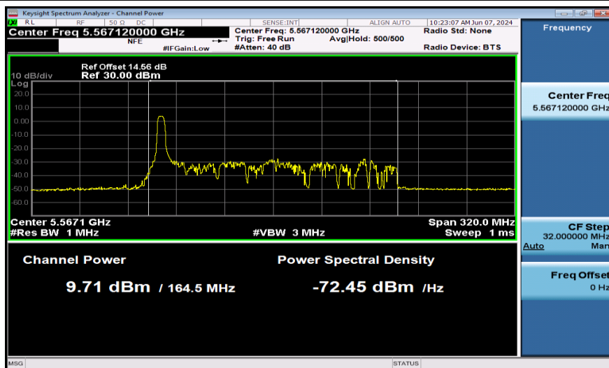
11AX160SISO-Ant1-5570-52Tone-PASS
