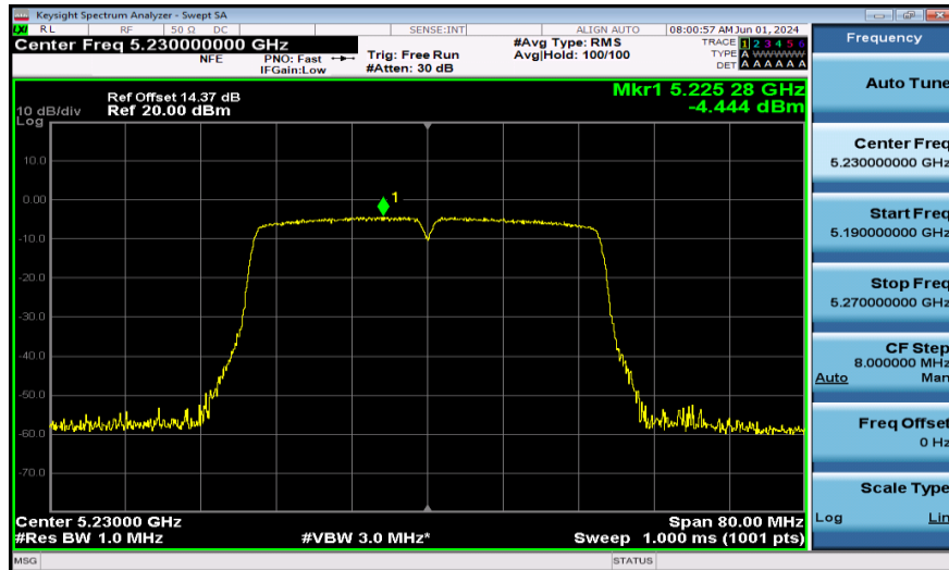
11AC40SISO-Ant1-5230-PASS
