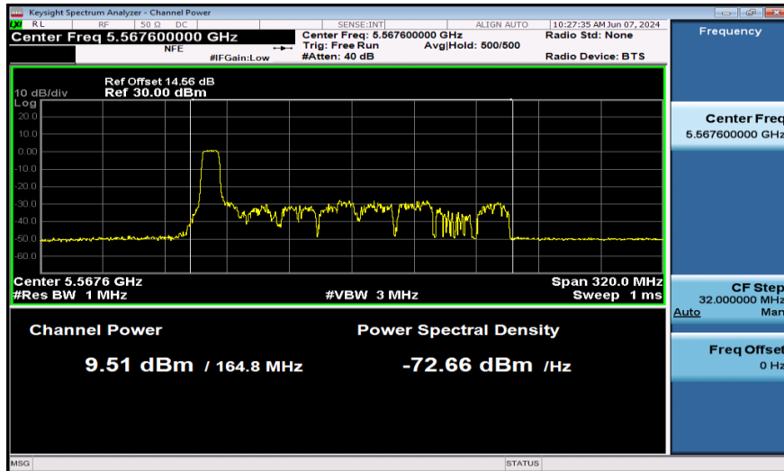
11AX160SISO-Ant1-5570-106Tone-PASS
