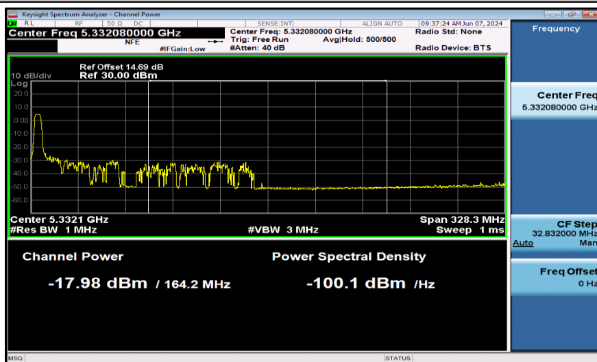
11AX160SISO-Ant1-5250_UNII-2A-52Tone-PASS
