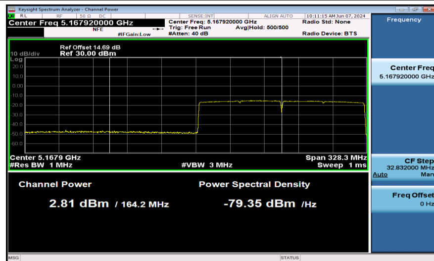
11AX160SISO-Ant1-5250_UNII-1-2*996Tone-PASS
