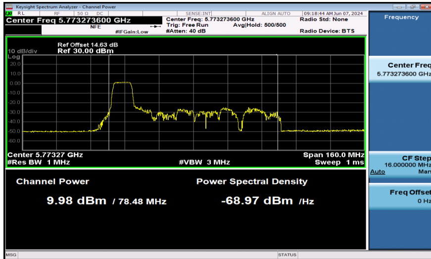
11AX80SISO-Ant1-5775-106Tone-PASS
