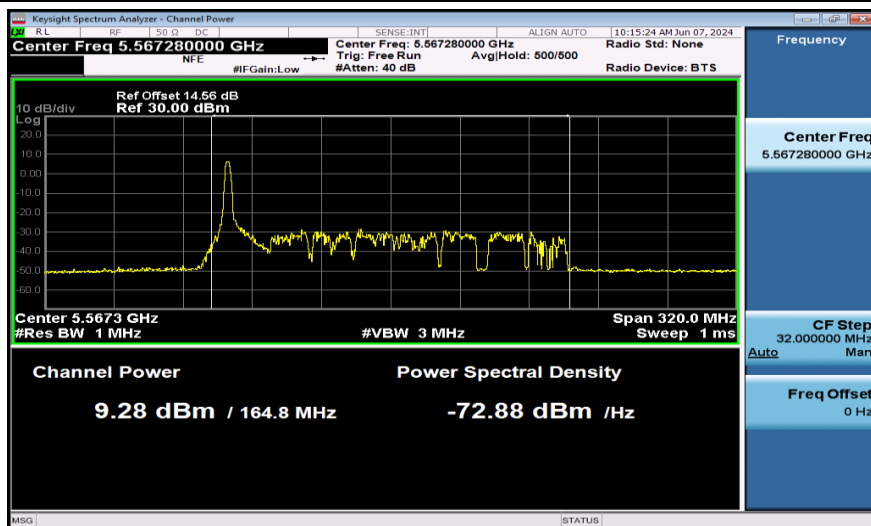
11AX160SISO-Ant1-5570-26Tone-PASS
