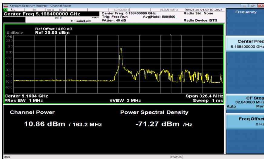
11AX160SISO-Ant1-5250_UNII-1-26Tone-PASS
