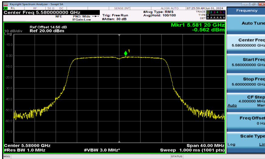
11N20SISO-Ant1-5580-PASS
