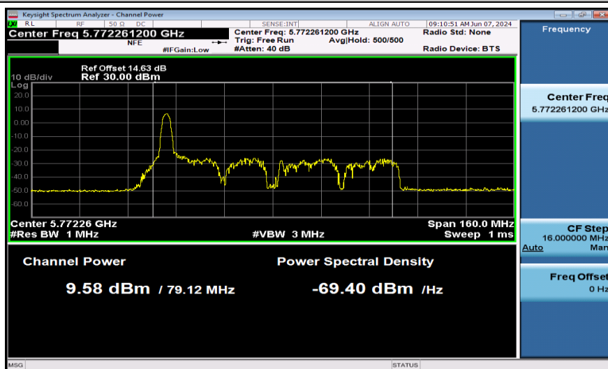
11AX80SISO-Ant1-5775-26Tone-PASS
