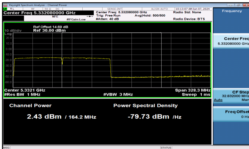
11AX160SISO-Ant1-5250_UNII-2A-2*996Tone-PASS
