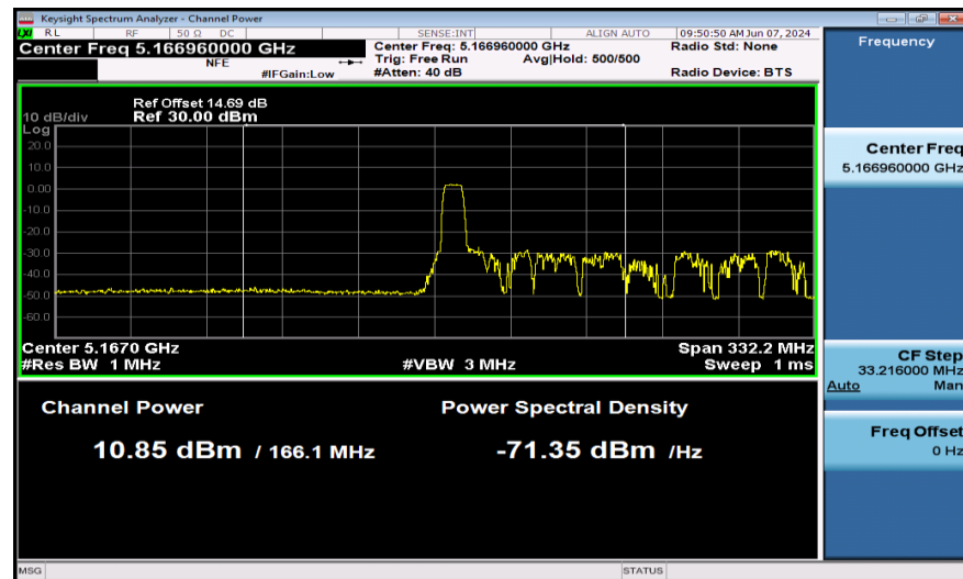
11AX160SISO-Ant1-5250_UNII-1-106Tone-PASS
