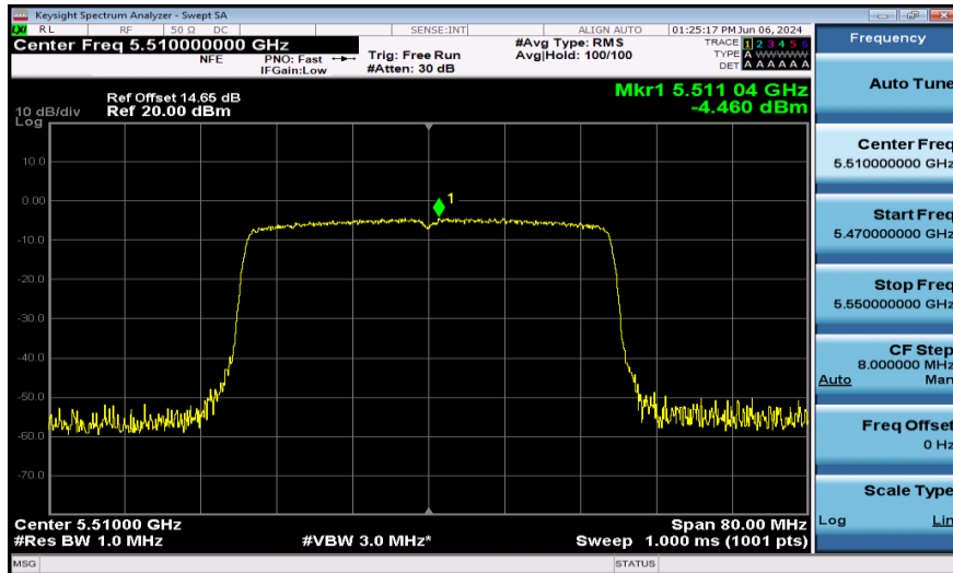
11AX40SISO-Ant1-5510-PASS
