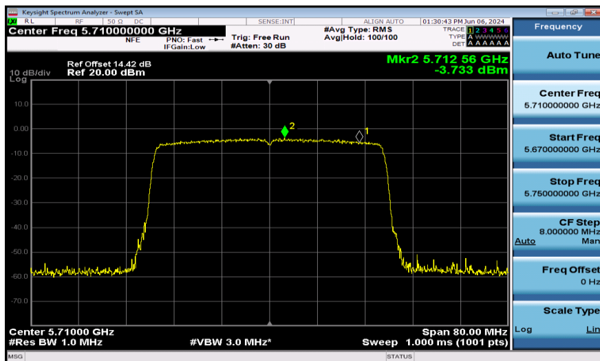
11AX40SISO-Ant1-5710_UNII-2C-PASS
