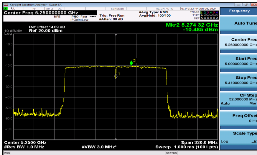
11AX160SISO-Ant1-5250_UNII-2A-PASS
