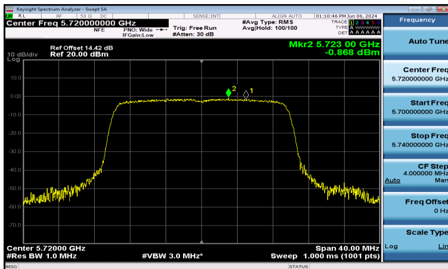
11AX20SISO-Ant1-5720_UNII-2C-PASS
