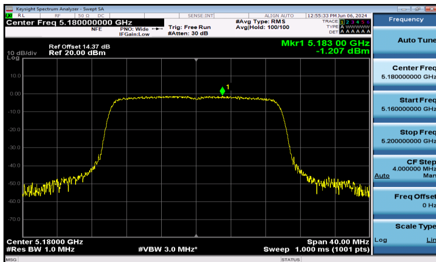
11AX20SISO-Ant1-5180-PASS
