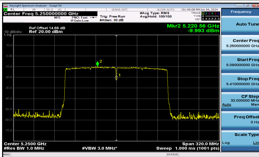
11AX160SISO-Ant1-5250_UNII-1-PASS
