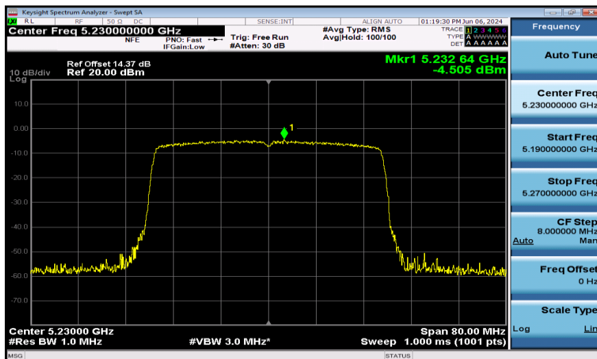
11AX40SISO-Ant1-5230-PASS
