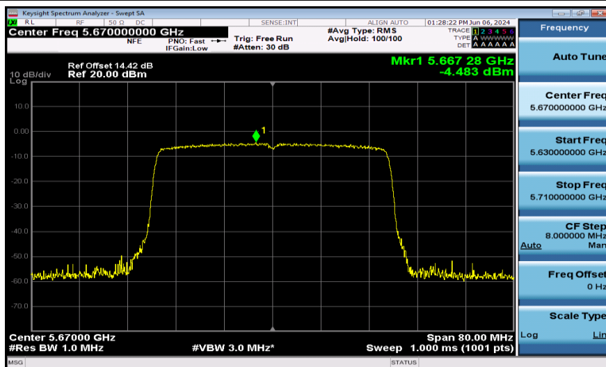
11AX40SISO-Ant1-5670-PASS
