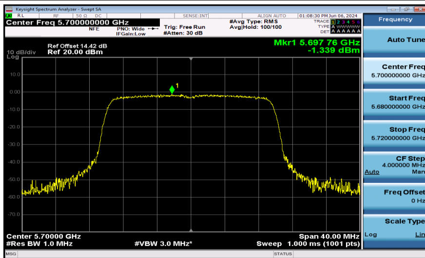
11AX20SISO-Ant1-5700-PASS
