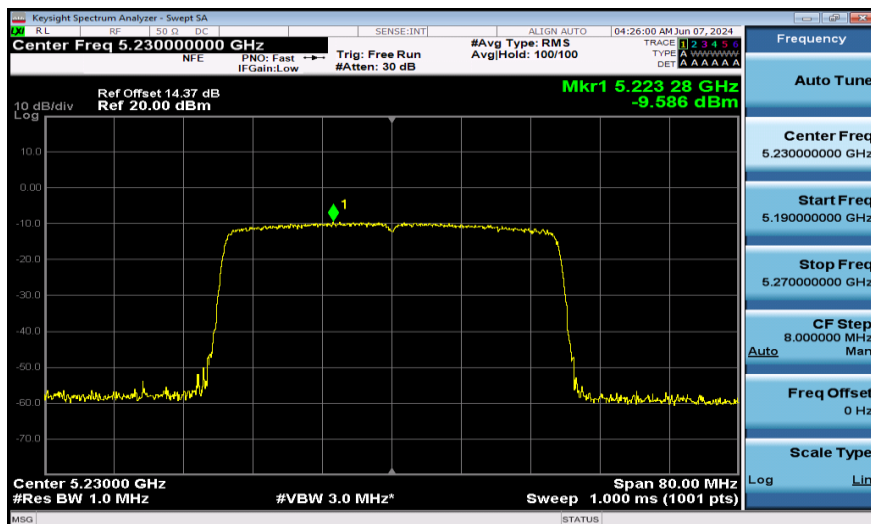
11AX40SISO-Ant1-5230-484Tone-PASS
