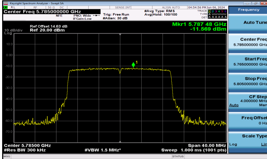
11AX20SISO-Ant1-5785-242Tone-PASS
