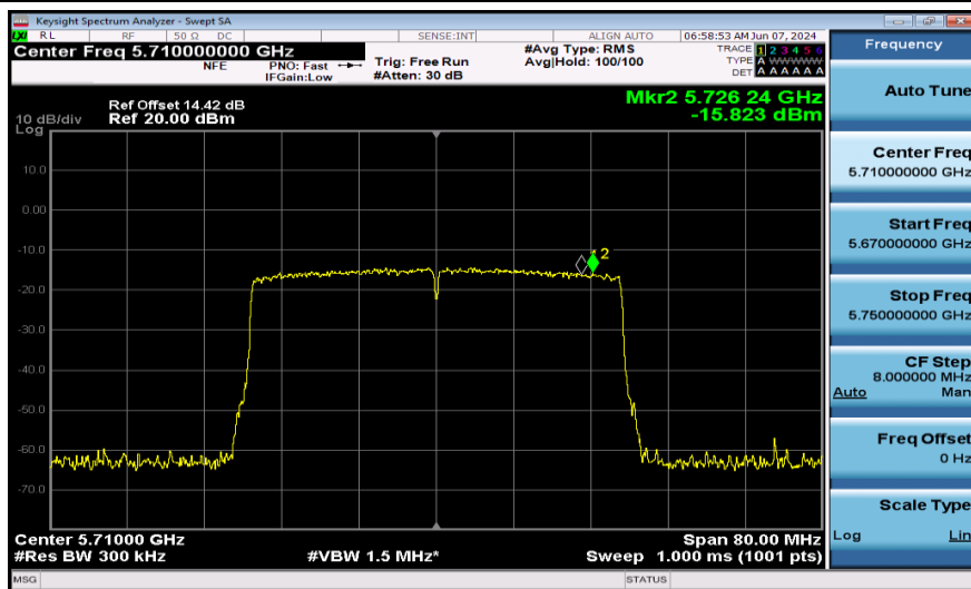
11AX40SISO-Ant1-5710_UNII-3-484Tone-PASS
