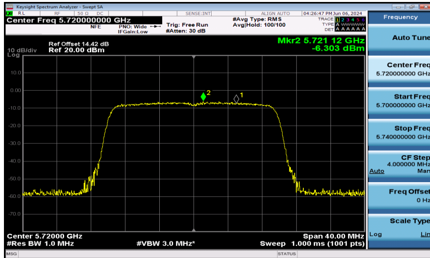
11AX20SISO-Ant1-5720_UNII-2C-242Tone-PASS
