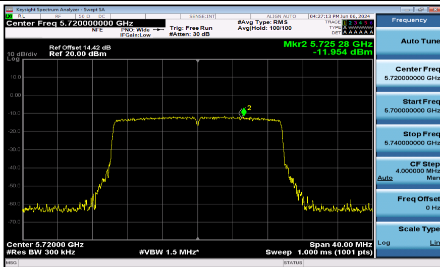
11AX20SISO-Ant1-5720_UNII-3-242Tone-PASS
