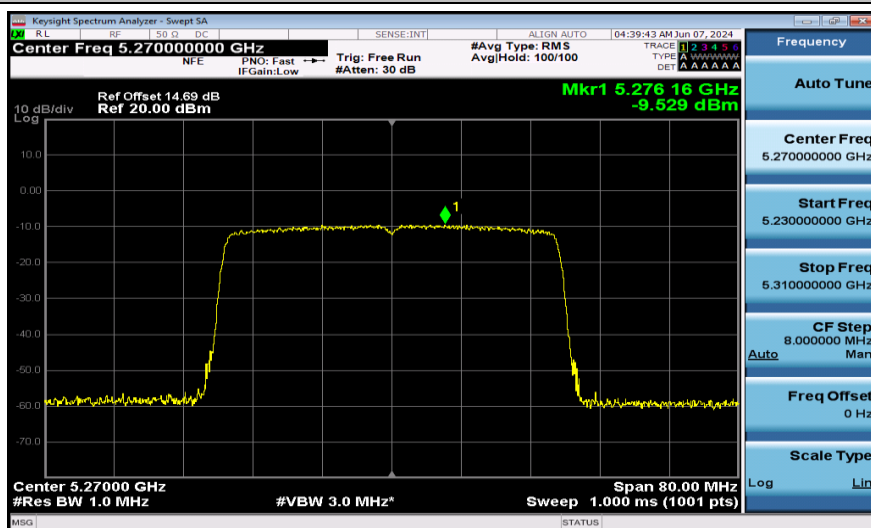
11AX40SISO-Ant1-5270-484Tone-PASS
