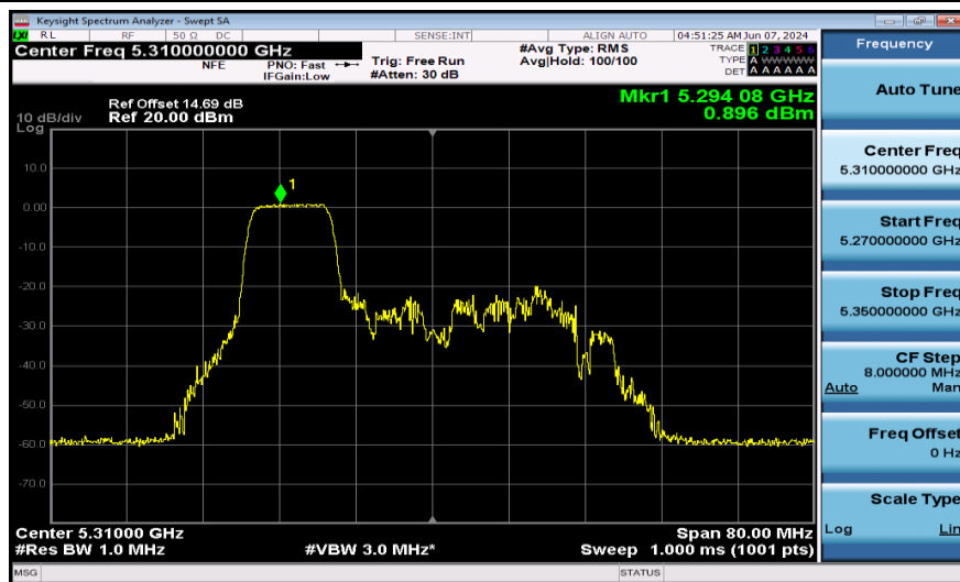
11AX40SISO-Ant1-5310-106Tone-PASS
