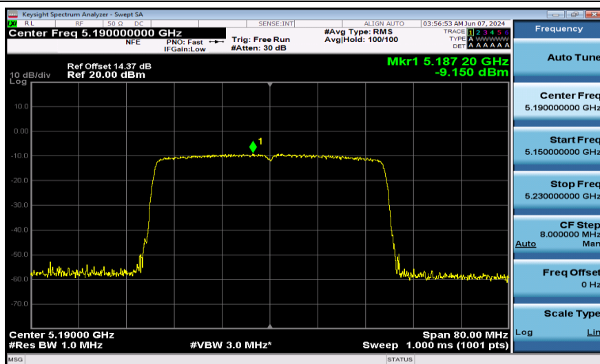
11AX40SISO-Ant1-5190-484Tone-PASS
