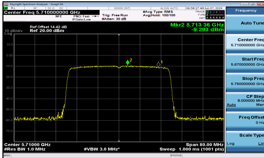
11AX40SISO-Ant1-5710_UNII-2C-484Tone-PASS
