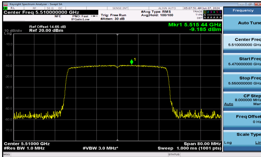
11AX40SISO-Ant1-5510-484Tone-PASS
