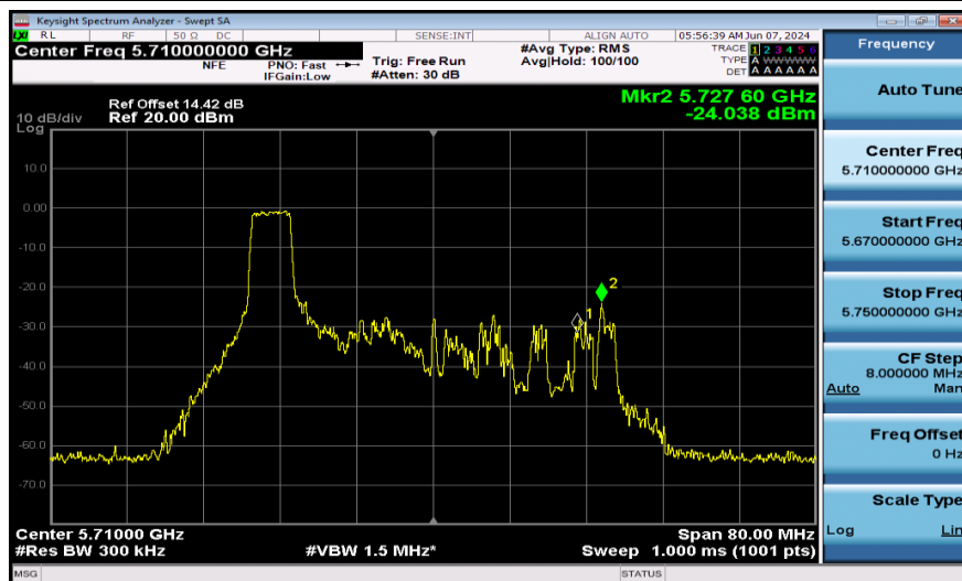
11AX40SISO-Ant1-5710_UNII-3-52Tone-PASS
