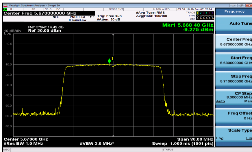
11AX40SISO-Ant1-5670-484Tone-PASS
