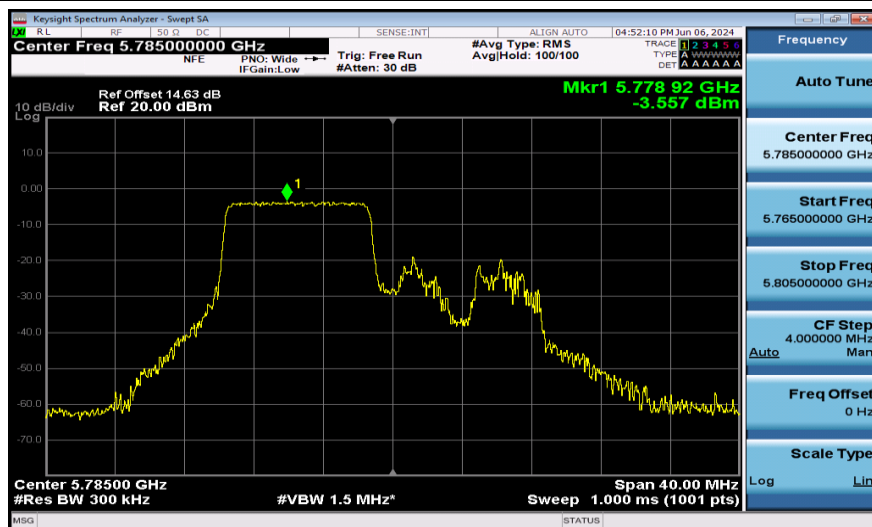
11AX20SISO-Ant1-5785-106Tone-PASS
