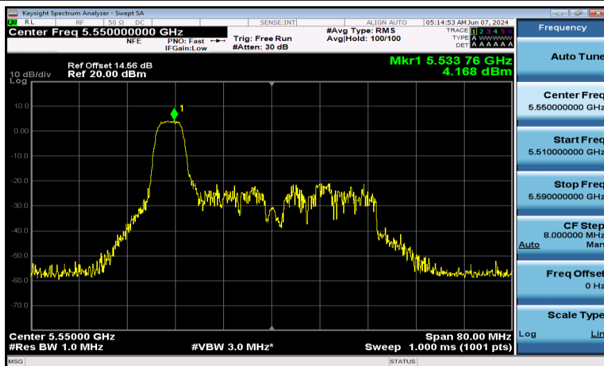
11AX40SISO-Ant1-5550-52Tone-PASS
