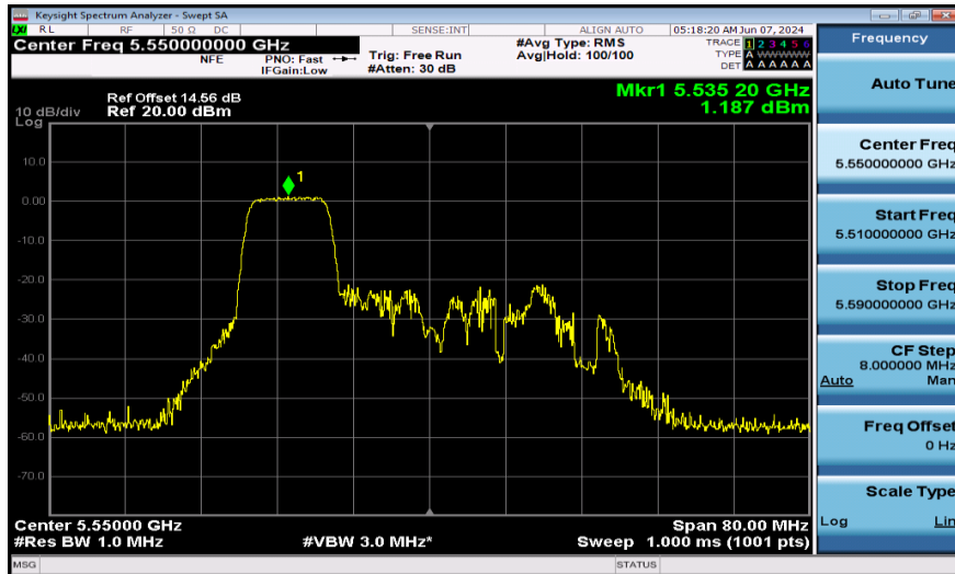
11AX40SISO-Ant1-5550-106Tone-PASS
