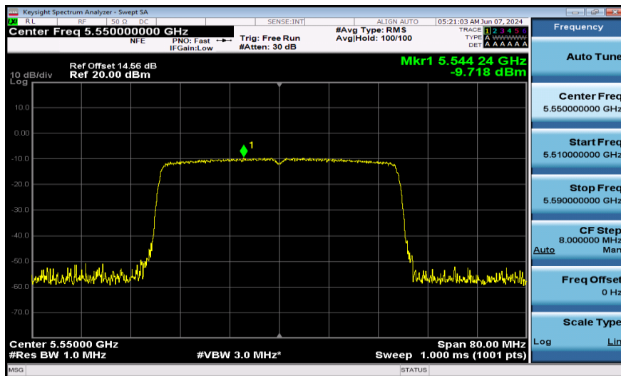
11AX40SISO-Ant1-5550-484Tone-PASS
