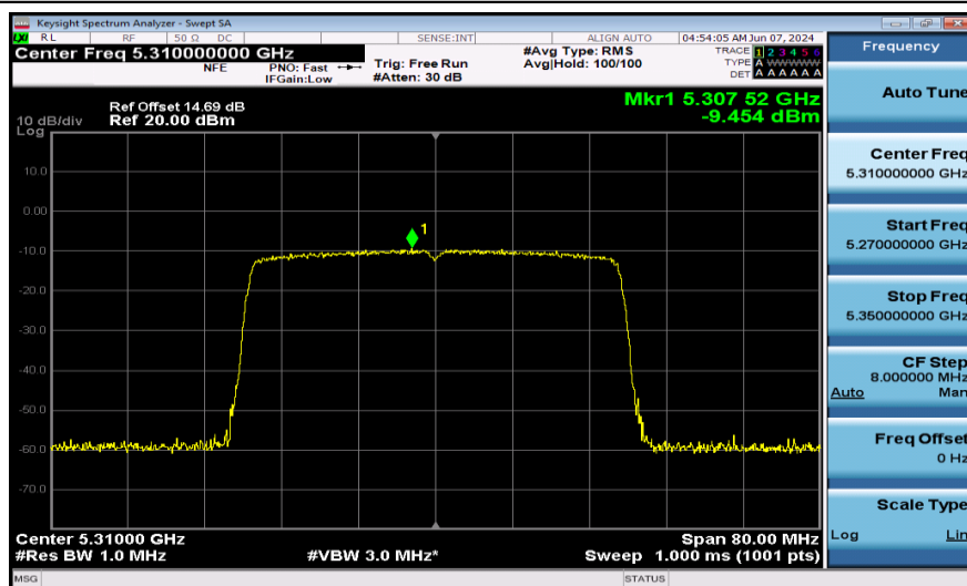
11AX40SISO-Ant1-5310-484Tone-PASS
