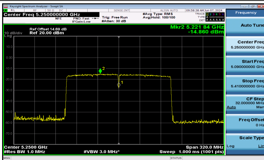
11AX160SISO-Ant1-5250_UNII-1-2*996Tone-PASS
