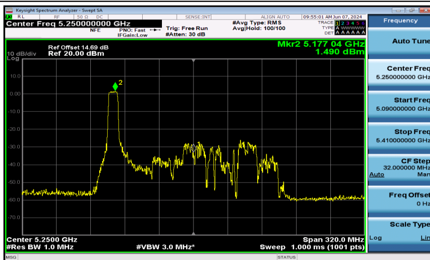
11AX160SISO-Ant1-5250_UNII-1-106Tone-PASS
