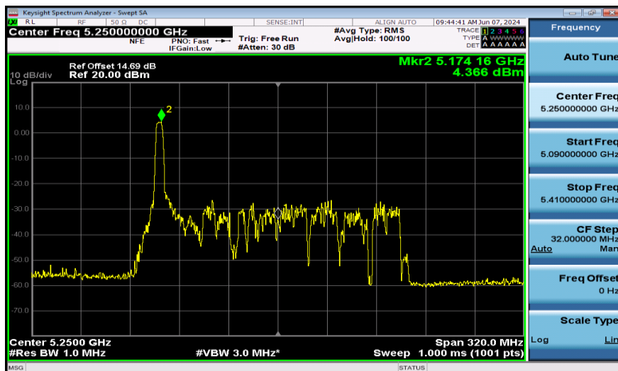
11AX160SISO-Ant1-5250_UNII-1-52Tone-PASS
