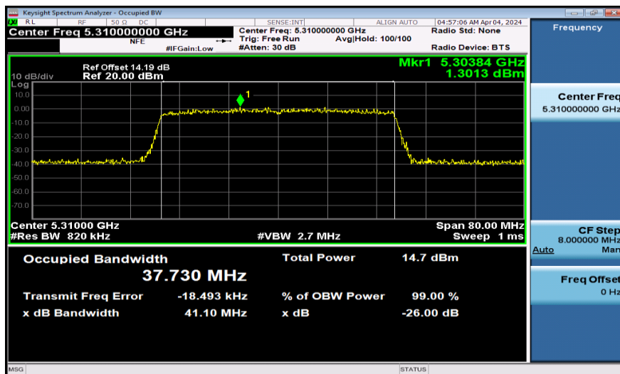
11AX40SISO-Ant1-5310
