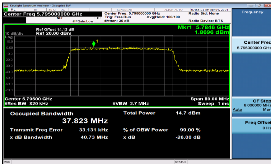
11AX40SISO-Ant1-5795
