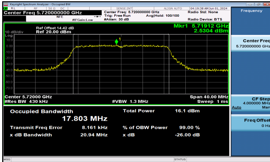
11AC20SISO-Ant1-5720
