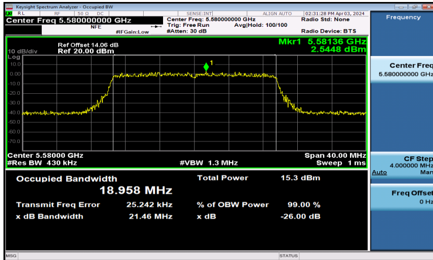
11AX20SISO-Ant1-5580
