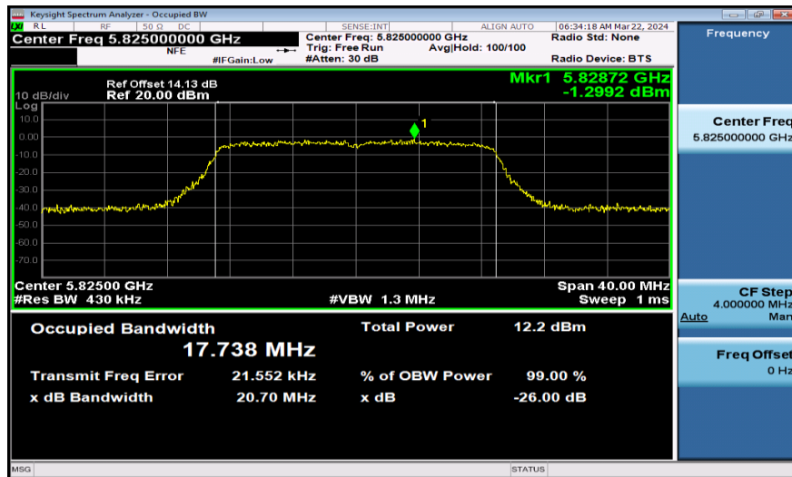
11AC20SISO-Ant1-5825
