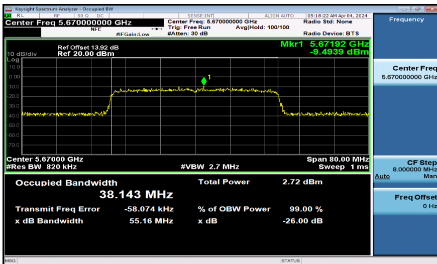
11AX40SISO-Ant1-5670
