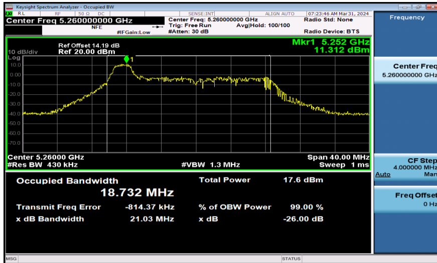
11AX20SISO-Ant1-5260-26Tone
