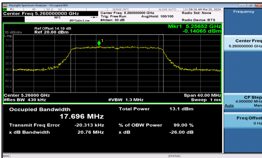
11AC20SISO-Ant1-5260
