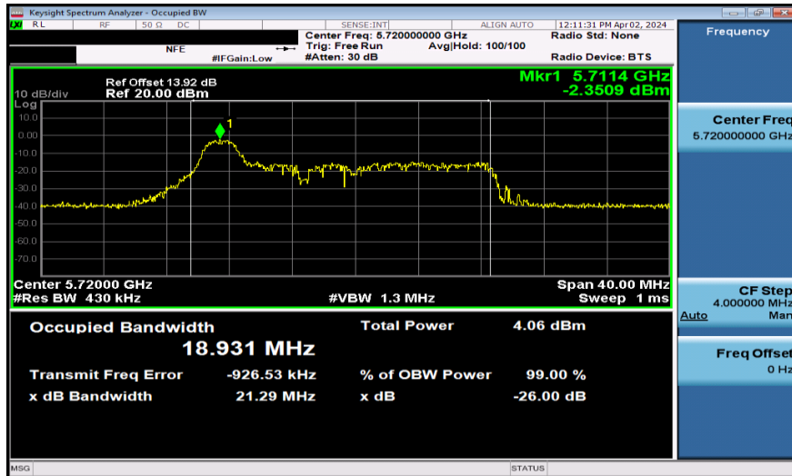
11AX20SISO-Ant1-5720-26Tone
