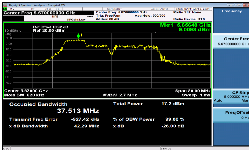
11AX40SISO-Ant1-5670-106Tone
