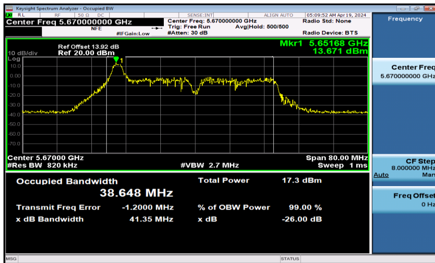
11AX40SISO-Ant1-5670-26Tone
