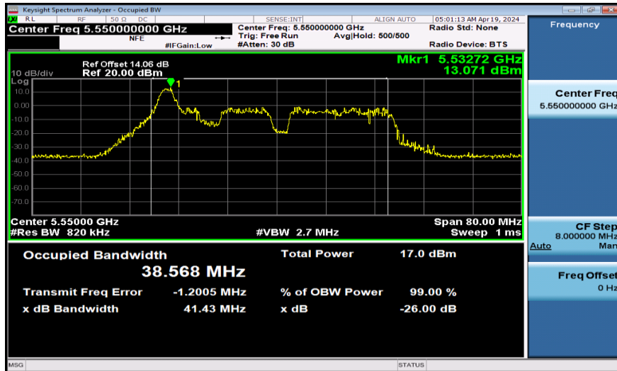
11AX40SISO-Ant1-5550-26Tone
