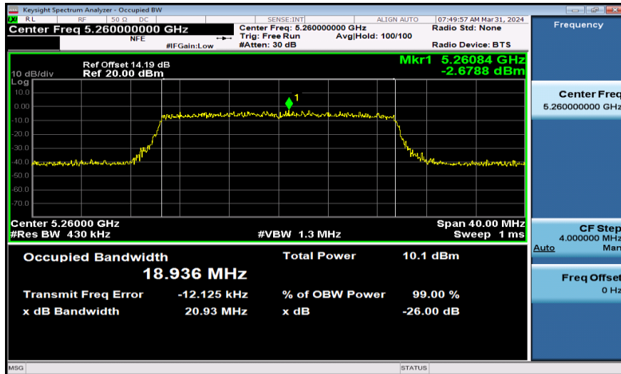
11AX20SISO-Ant1-5260-242Tone
