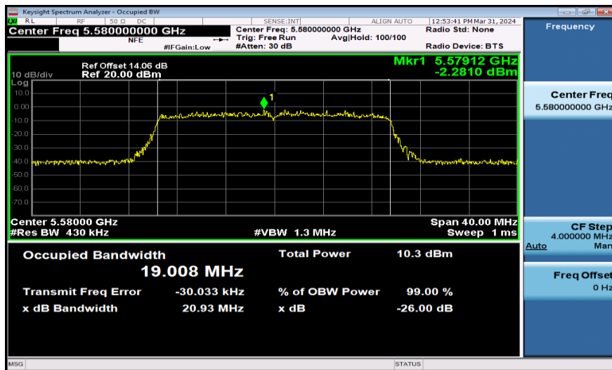
11AX20SISO-Ant1-5580-242Tone
