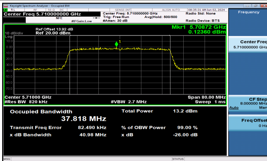
11AX40SISO-Ant1-5710-484Tone
