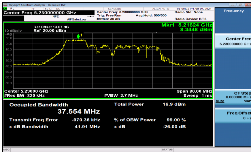
11AX40SISO-Ant1-5230-106Tone-RU53
