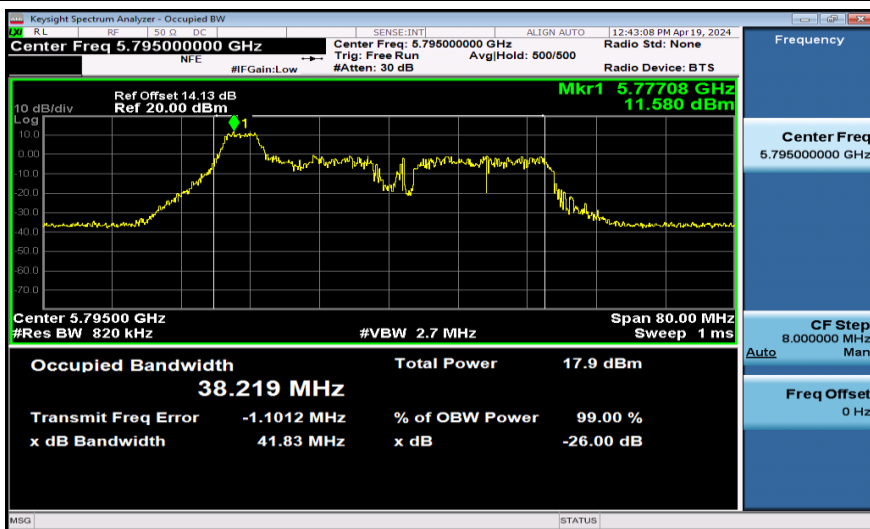
11AX40SISO-Ant1-5795-52Tone
