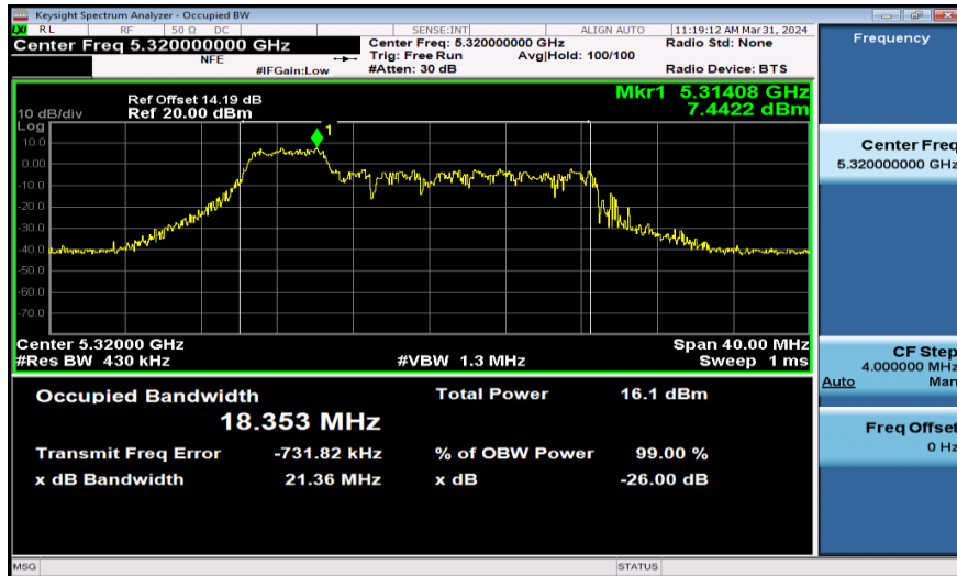
11AX20SISO-Ant1-5320-52Tone
