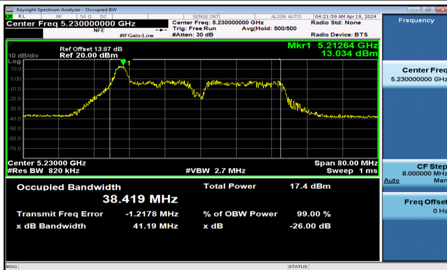
11AX40SISO-Ant1-5230-26Tone-RU0
