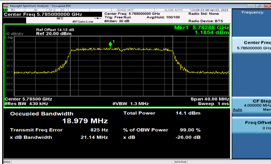
11AX20SISO-Ant1-5785-242Tone
