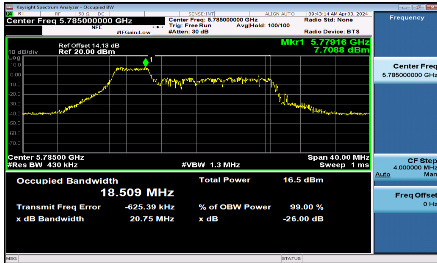
11AX20SISO-Ant1-5785-52Tone
