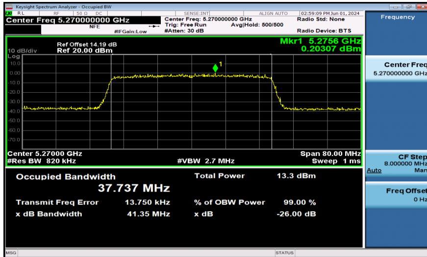
11AX40SISO-Ant1-5270-484Tone-RU61
