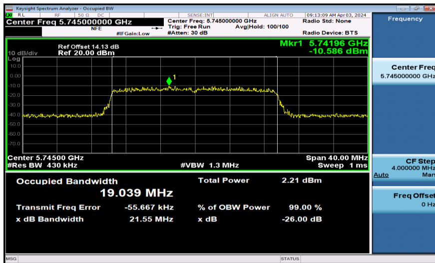
11AX20SISO-Ant1-5745-242Tone
