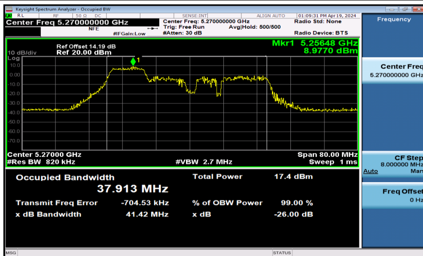
11AX40SISO-Ant1-5270-106Tone-RU53
