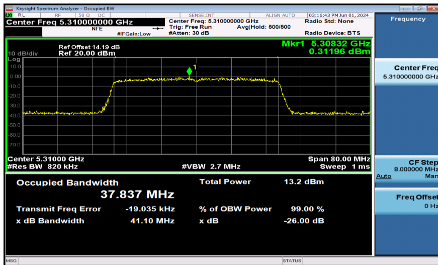
11AX40SISO-Ant1-5310-484Tone-RU61
