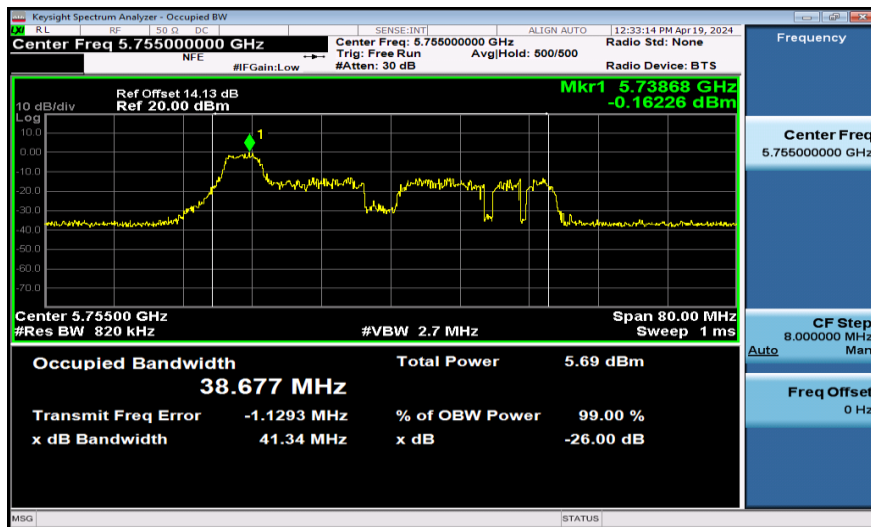
11AX40SISO-Ant1-5755-52Tone
