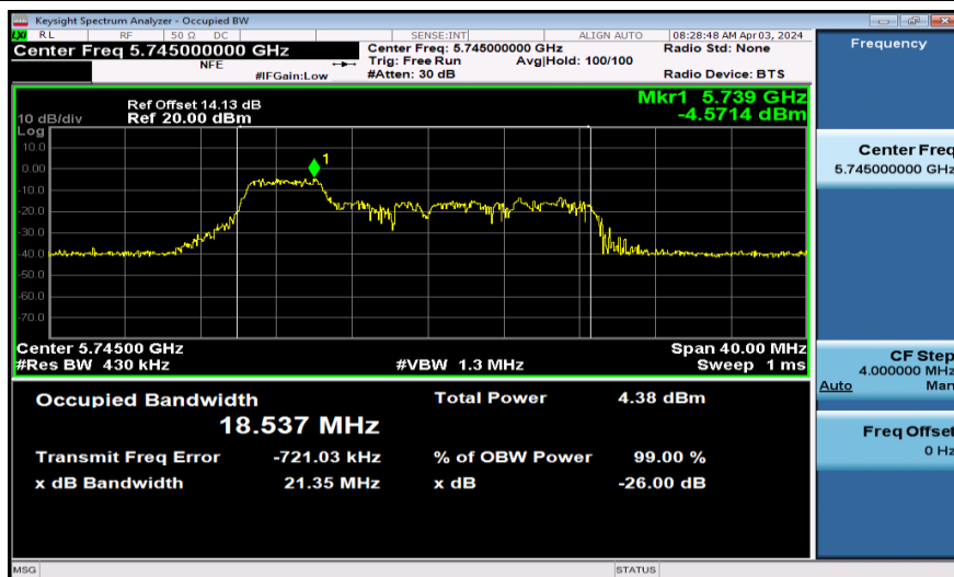
11AX20SISO-Ant1-5745-52Tone
