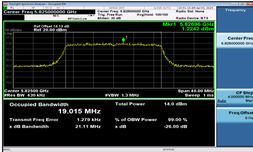
11AX20SISO-Ant1-5825-242Tone
