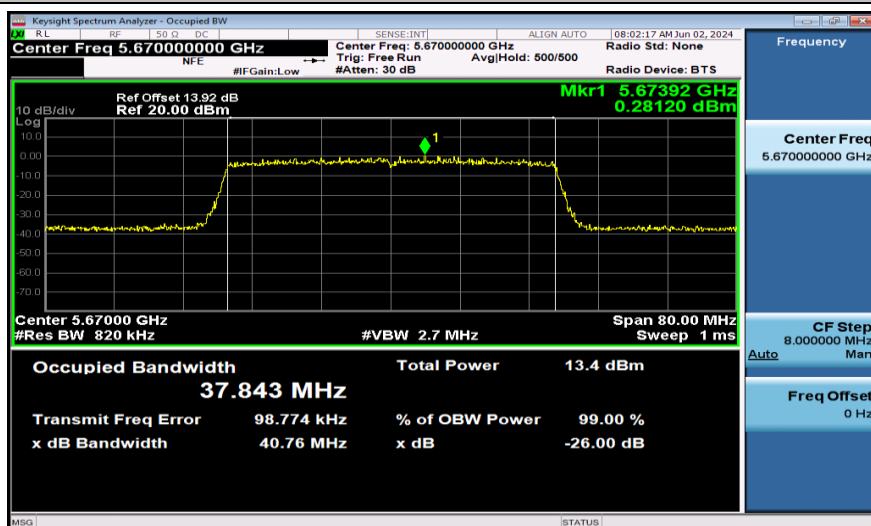
11AX40SISO-Ant1-5670-484Tone
