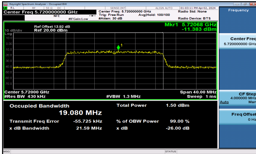
11AX20SISO-Ant1-5720-242Tone
