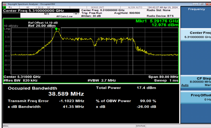
11AX40SISO-Ant1-5310-26Tone-RU0
