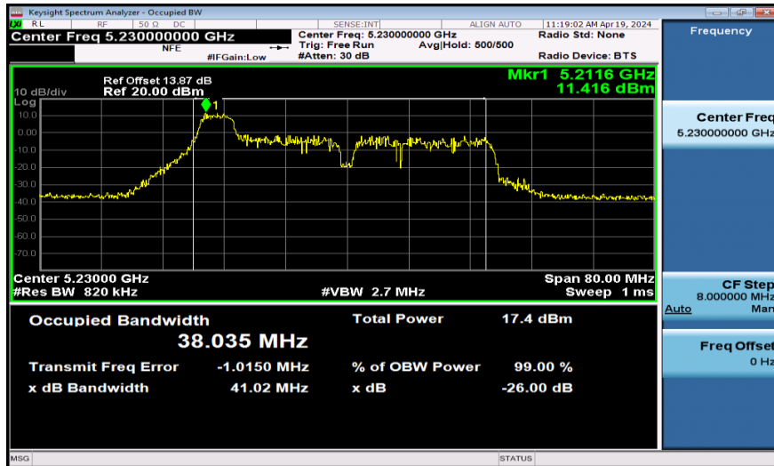
11AX40SISO-Ant1-5230-52Tone-RU37
