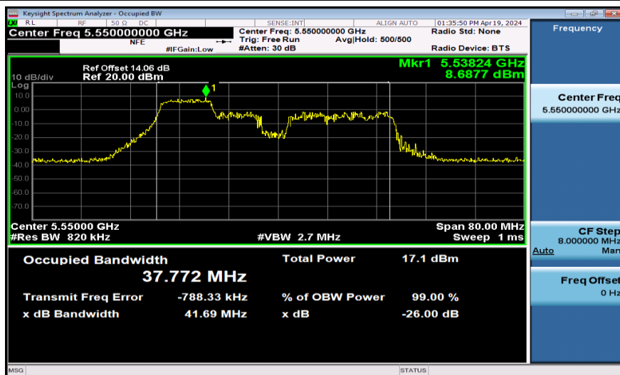
11AX40SISO-Ant1-5550-106Tone
