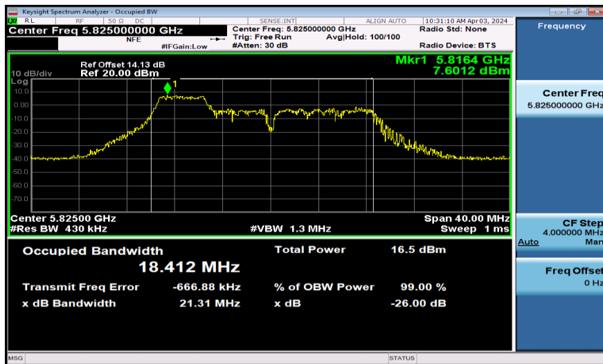
11AX20SISO-Ant1-5825-52Tone
