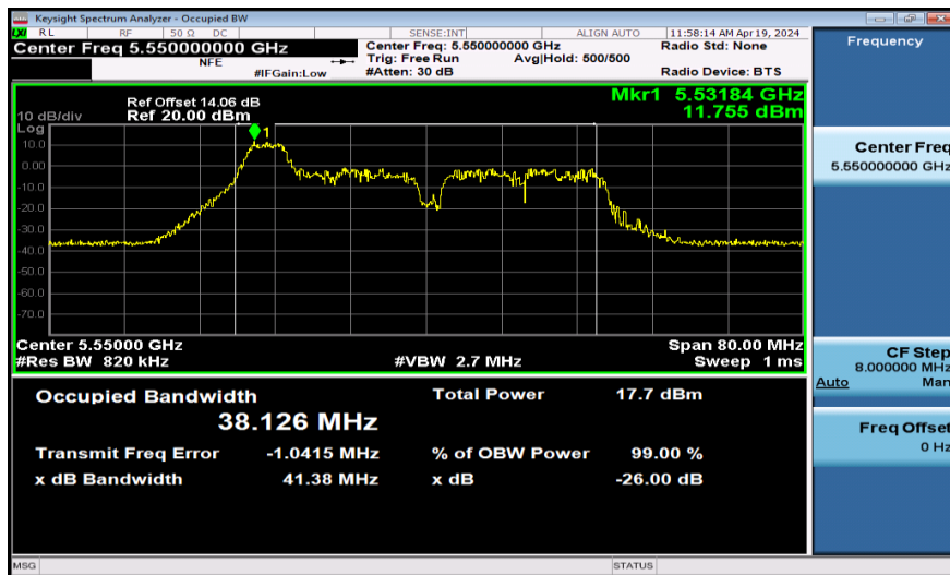
11AX40SISO-Ant1-5550-52Tone
