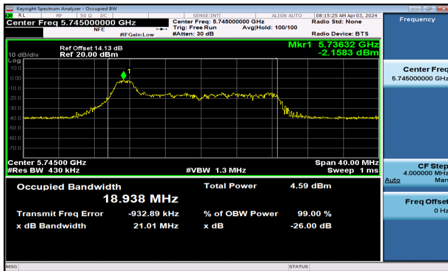
11AX20SISO-Ant1-5745-26Tone
