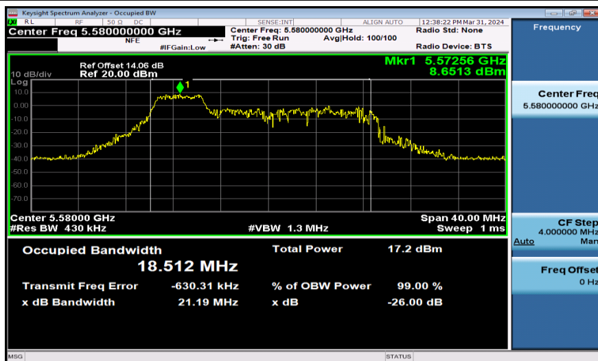
11AX20SISO-Ant1-5580-52Tone
