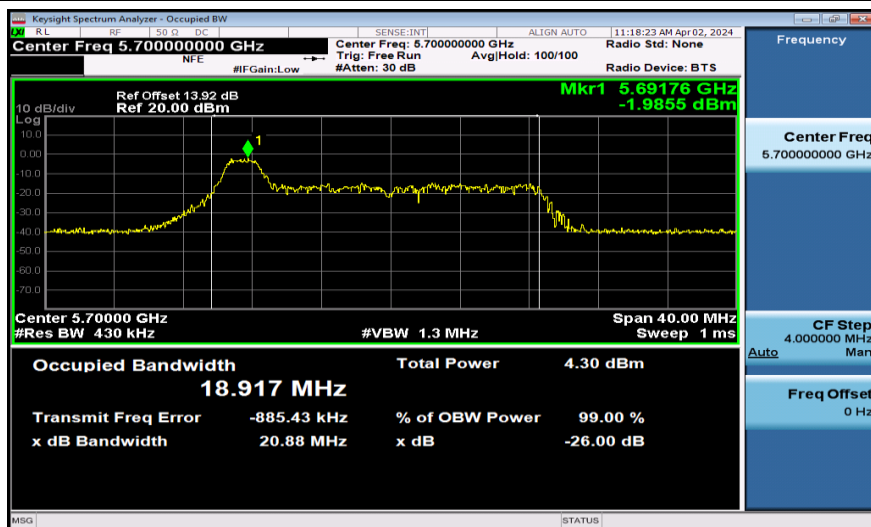
11AX20SISO-Ant1-5700-26Tone
