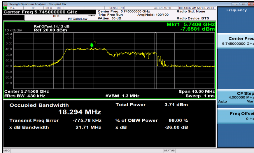
11AX20SISO-Ant1-5745-106Tone
