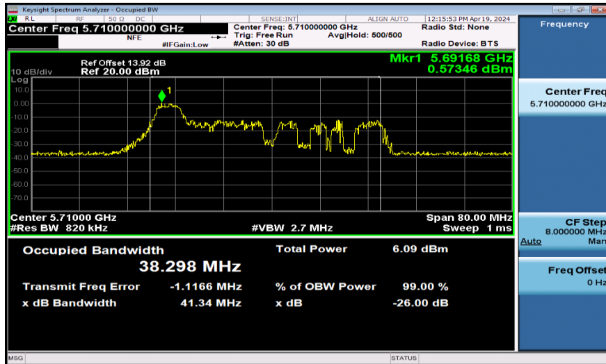
11AX40SISO-Ant1-5710-52Tone
