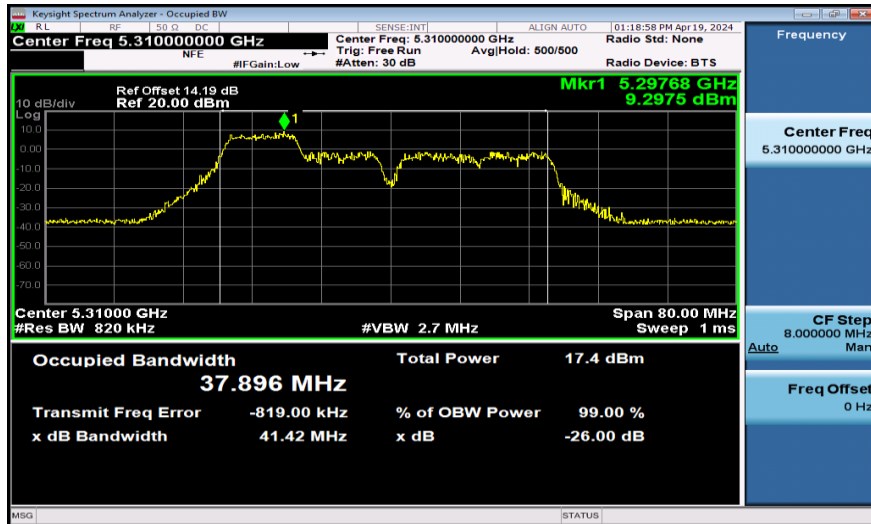
11AX40SISO-Ant1-5310-106Tone-RU53
