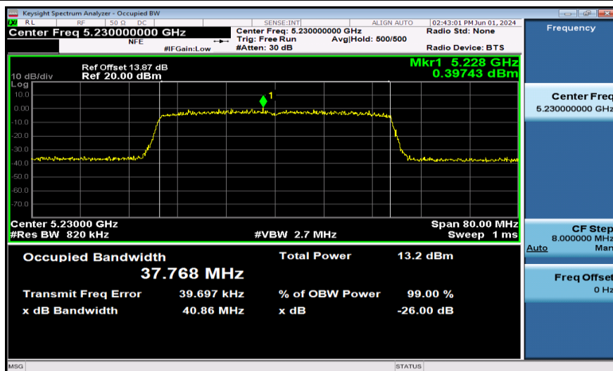
11AX40SISO-Ant1-5230-484Tone-RU61
