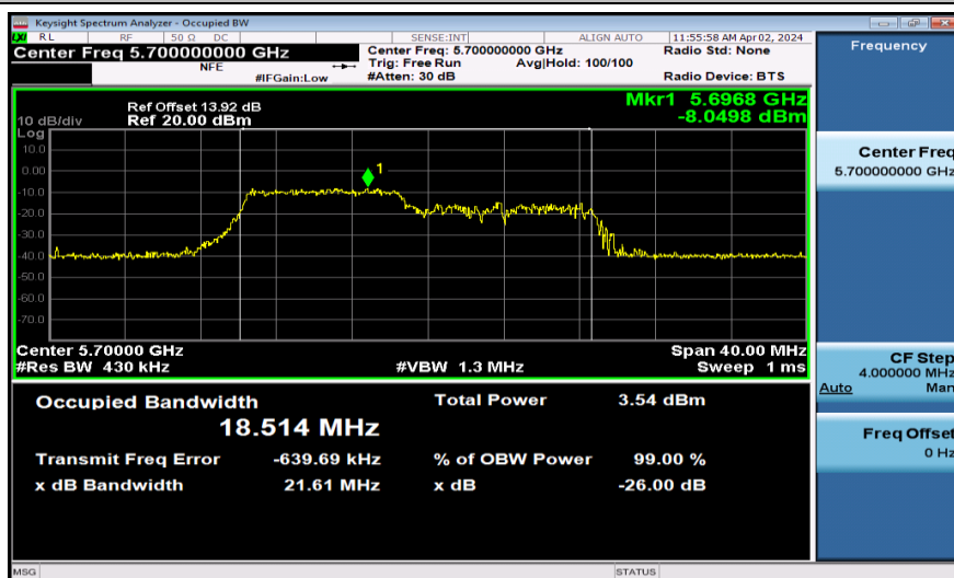
11AX20SISO-Ant1-5700-106Tone
