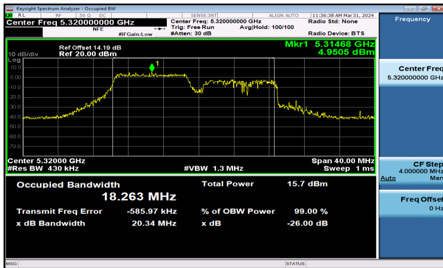
11AX20SISO-Ant1-5320-106Tone
