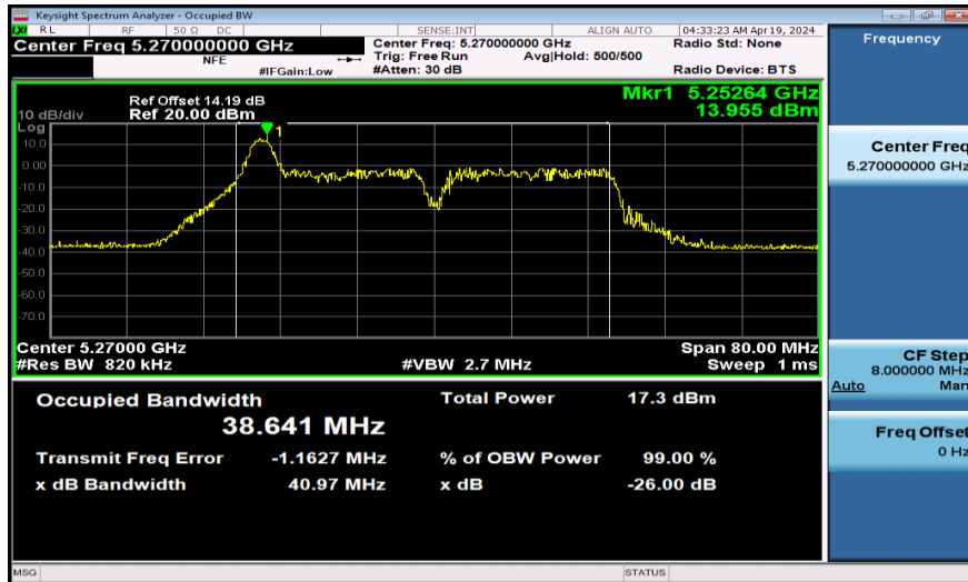
11AX40SISO-Ant1-5270-26Tone-RU0
