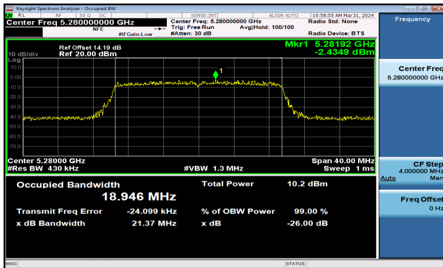
11AX20SISO-Ant1-5280-242Tone
