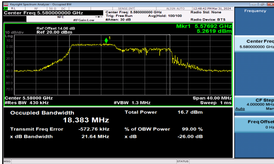
11AX20SISO-Ant1-5580-106Tone
