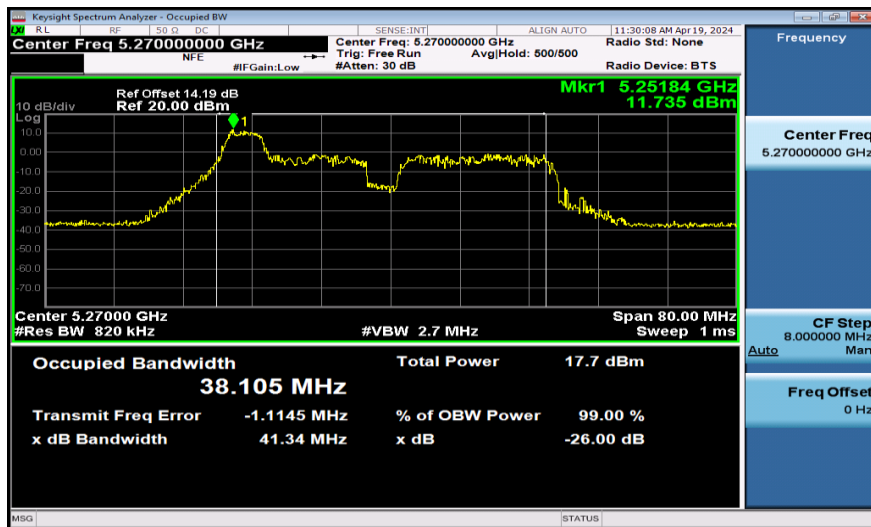
11AX40SISO-Ant1-5270-52Tone-RU37
