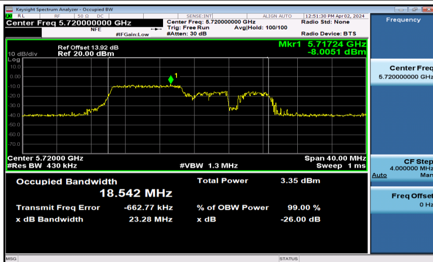
11AX20SISO-Ant1-5720-106Tone
