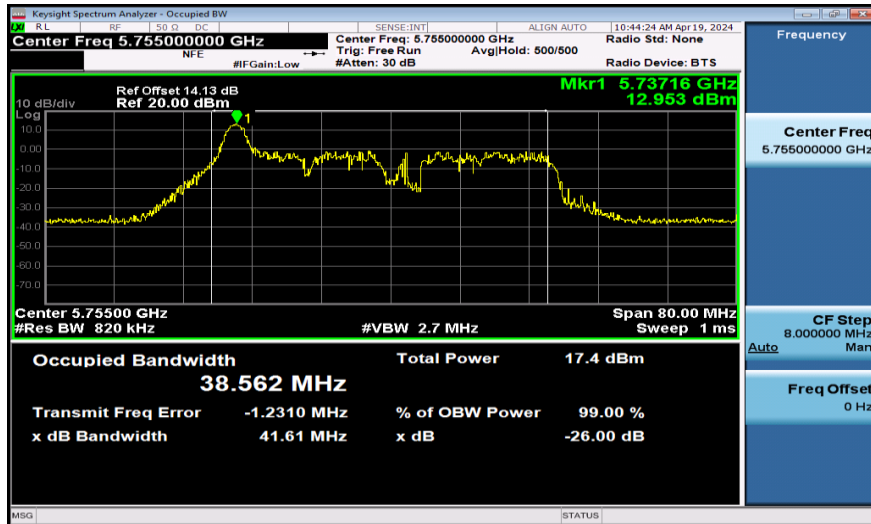
11AX40SISO-Ant1-5755-26Tone
