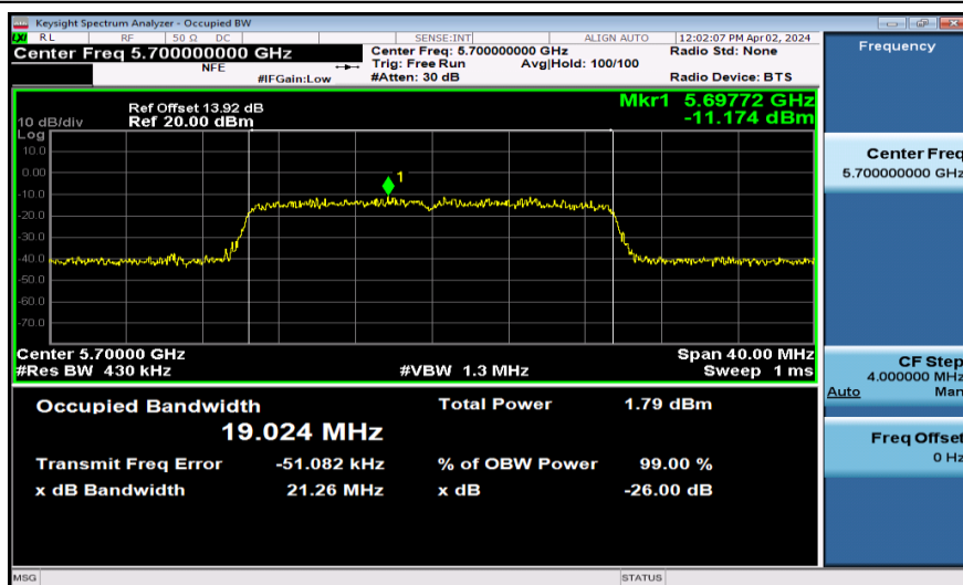
11AX20SISO-Ant1-5700-242Tone
