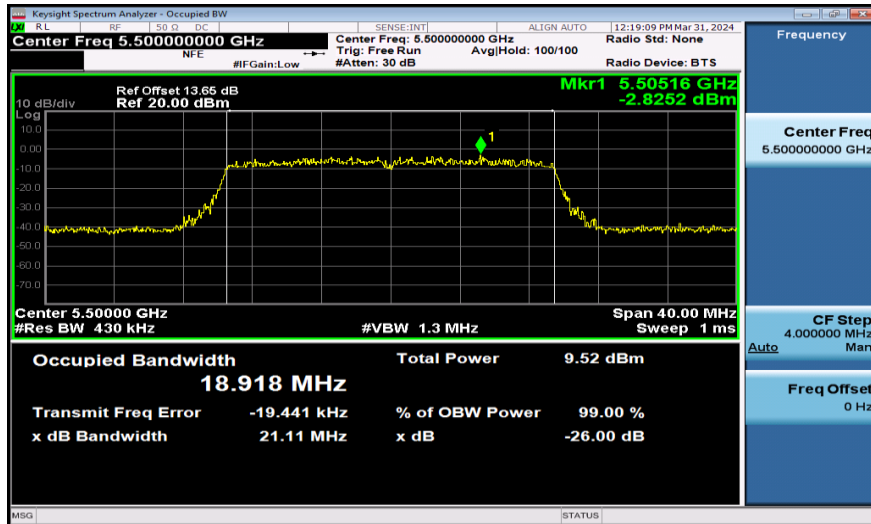
11AX20SISO-Ant1-5500-242Tone
