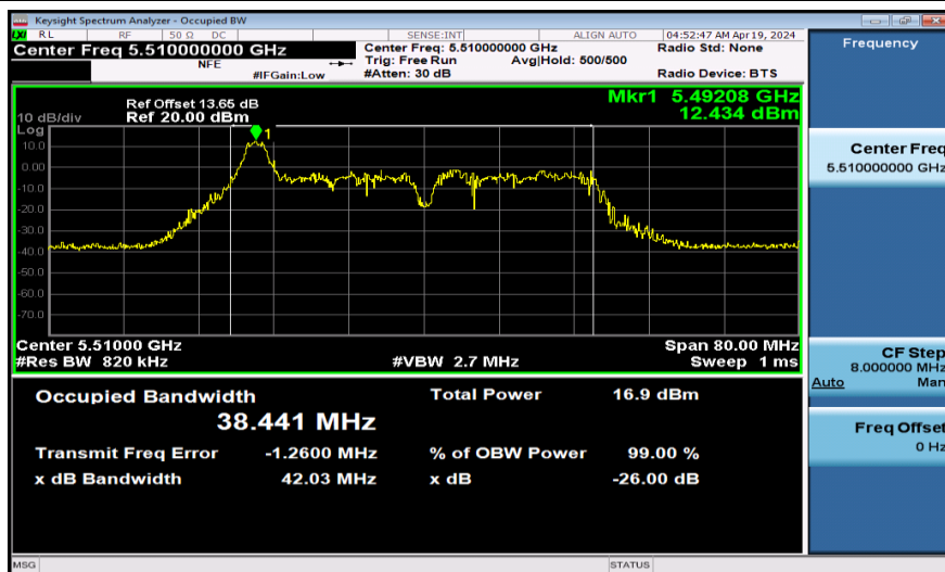
11AX40SISO-Ant1-5510-26Tone-RU0
