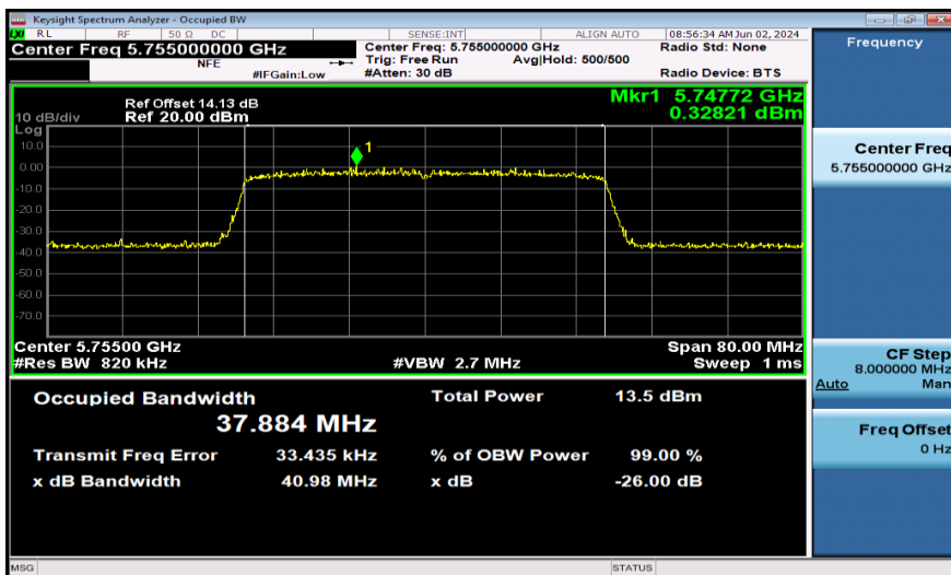
11AX40SISO-Ant1-5755-484Tone
