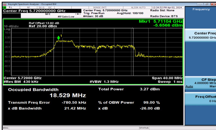
11AX20SISO-Ant1-5720-52Tone
