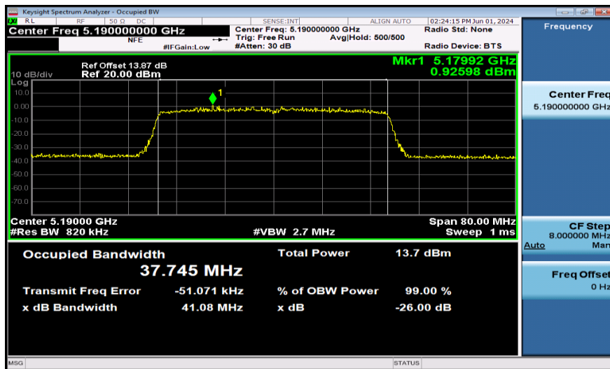
11AX40SISO-Ant1-5190-484Tone-RU61
