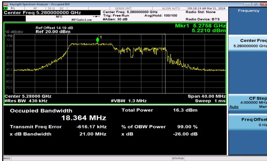
11AX20SISO-Ant1-5280-106Tone
