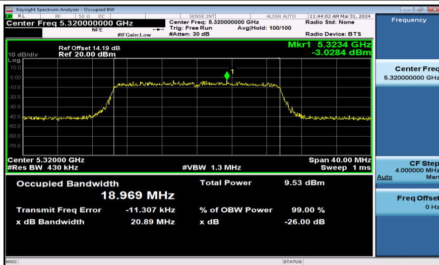
11AX20SISO-Ant1-5320-242Tone
