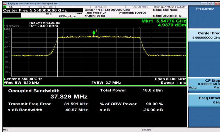
11AX40SISO-Ant1-5550-484Tone
