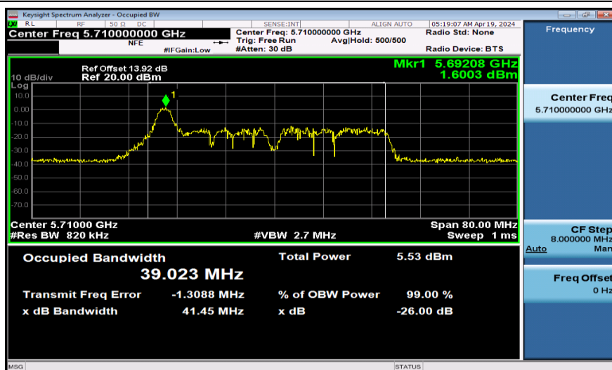
11AX40SISO-Ant1-5710-26Tone
