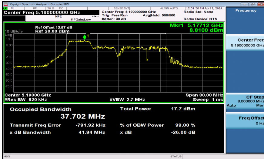
11AX40SISO-Ant1-5190-106Tone-RU53
