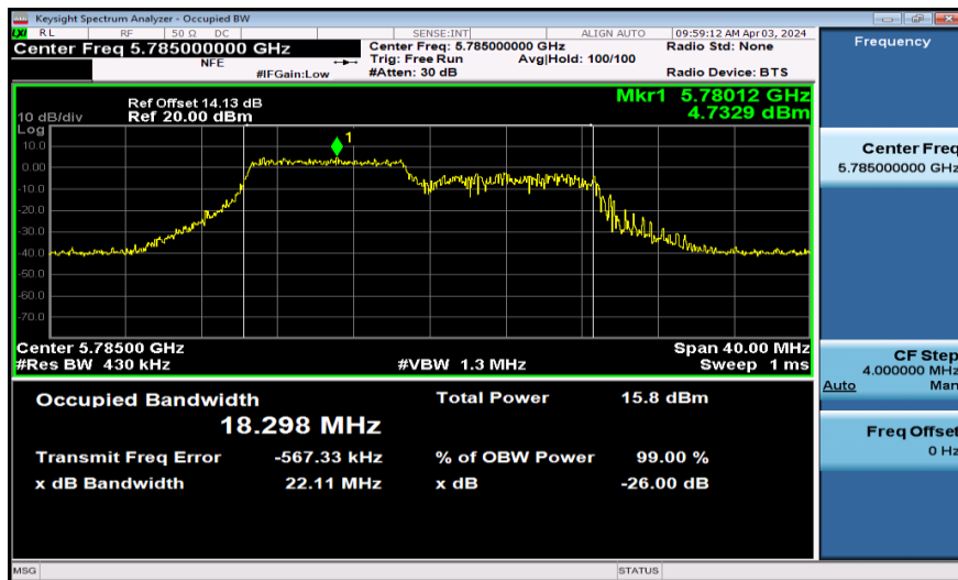
11AX20SISO-Ant1-5785-106Tone
