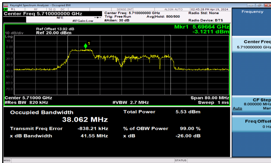
11AX40SISO-Ant1-5710-106Tone
