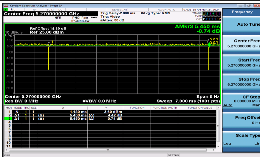
NTNV-11N40SISO-Ant1-5270
