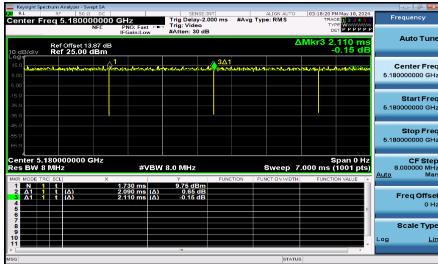
NTNV-11A-Ant1-5180
