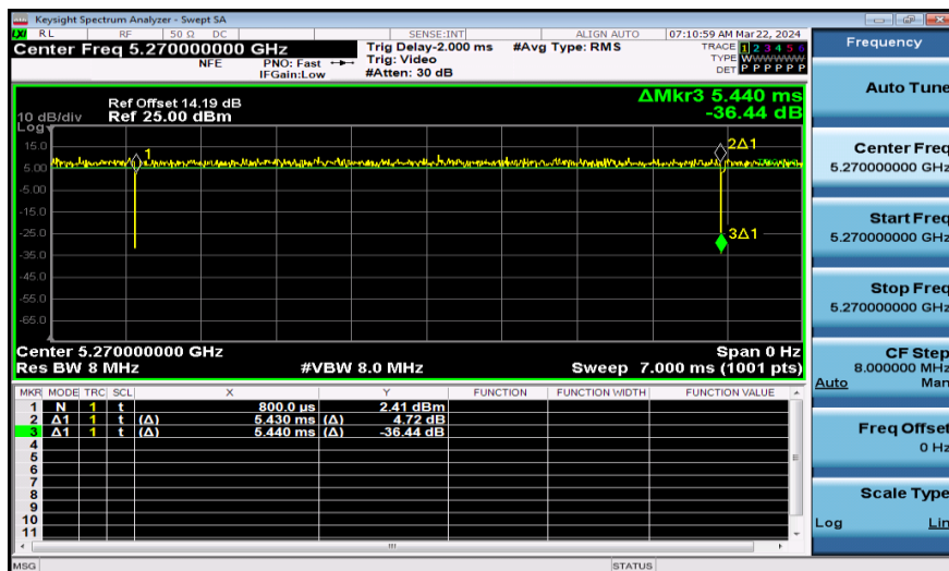
NTNV-11AC40SISO-Ant1-5270
