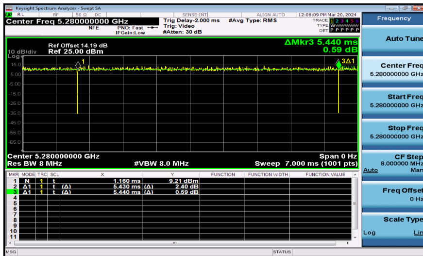
NTNV-11AC20SISO-Ant1-5280
