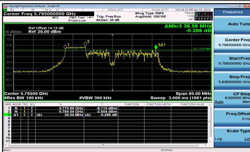
11AX40SISO-Ant1-5795-106Tone-PASS
