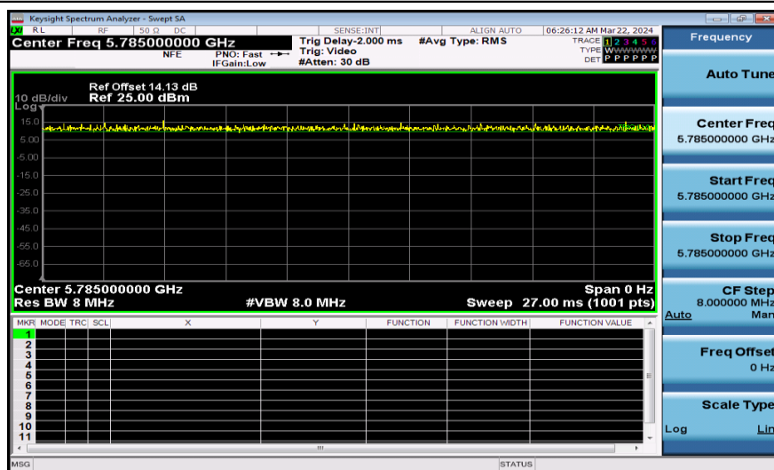
NTNV-11AC20SISO-Ant1-5785
