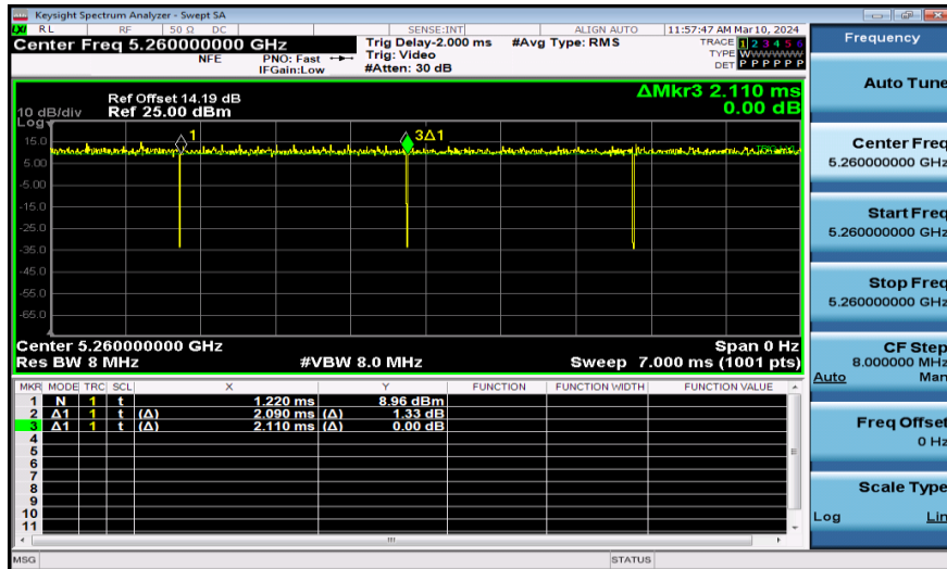
NTNV-11A-Ant1-5260
