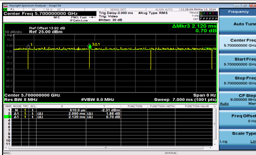
NTNV-11A-Ant1-5700
