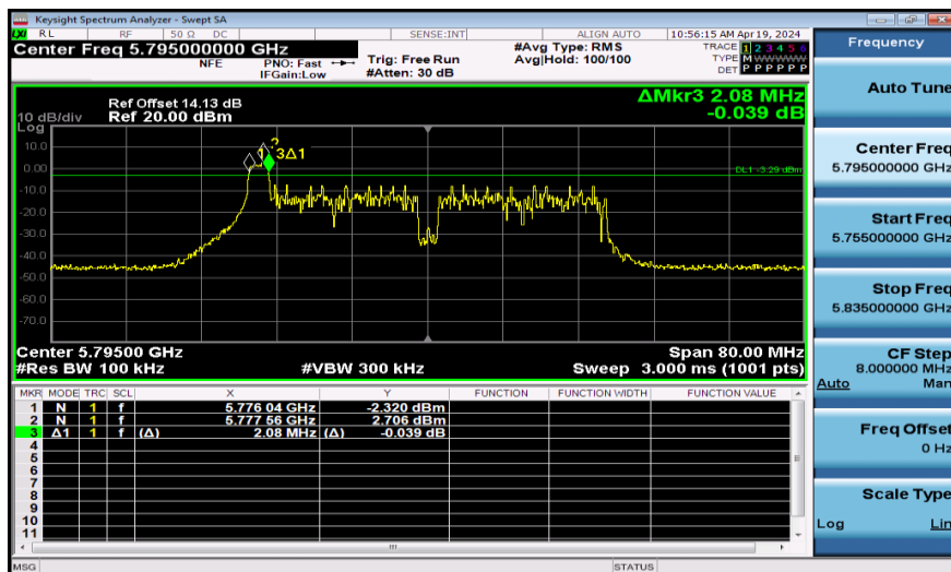
11AX40SISO-Ant1-5795-26Tone-PASS
