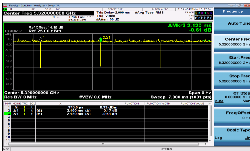
NTNV-11A-Ant1-5320
