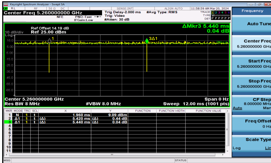
NTNV-11AC20SISO-Ant1-5260
