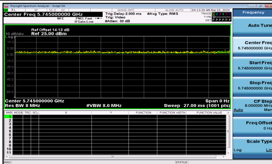
NTNV-11AC20SISO-Ant1-5745
