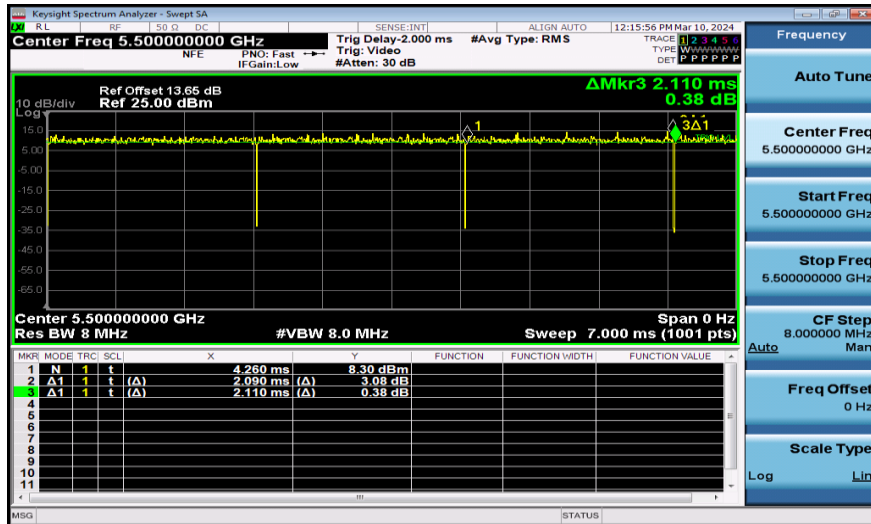
NTNV-11A-Ant1-5500
