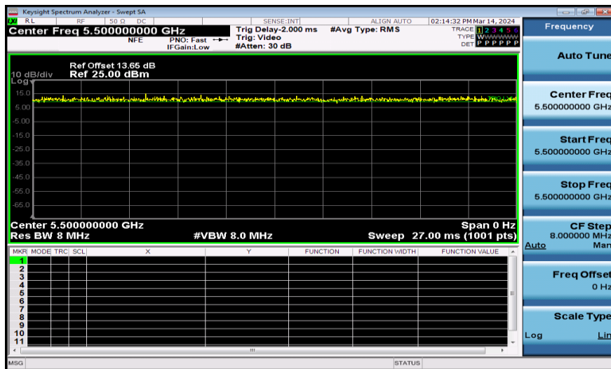
NTNV-11N20SISO-Ant1-5500
