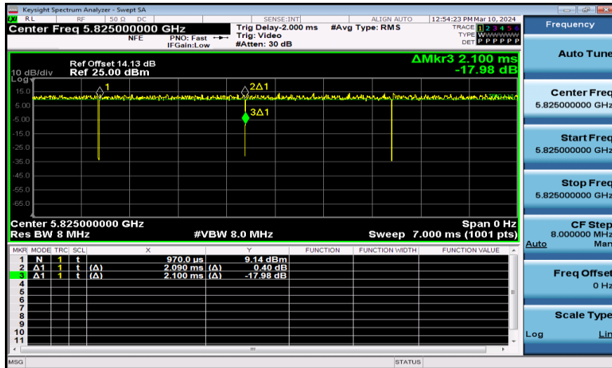
NTNV-11A-Ant1-5825
