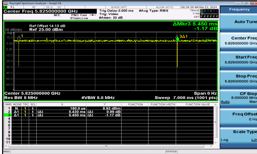
NTNV-11AC20SISO-Ant1-5825
