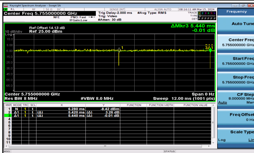
NTNV-11N40SISO-Ant1-5755
