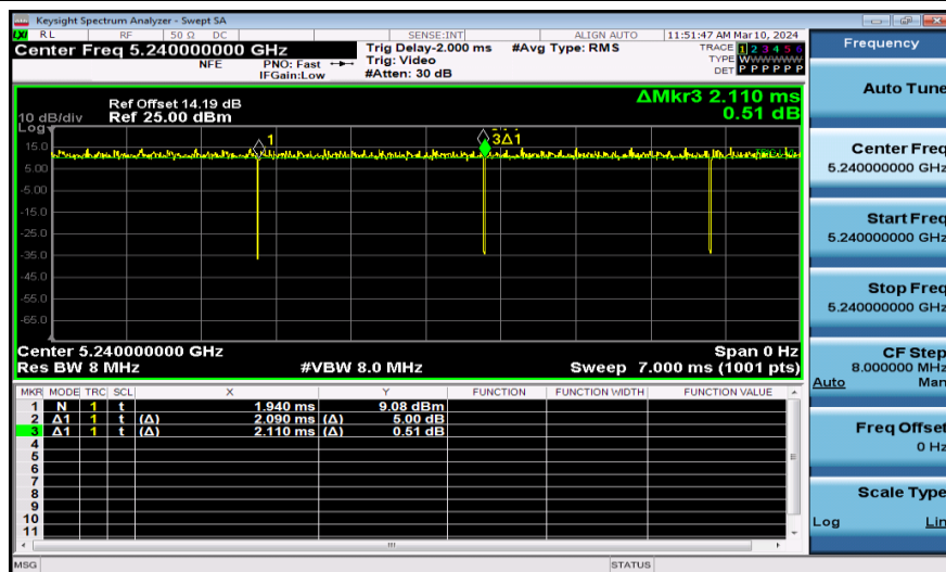
NTNV-11A-Ant1-5240
