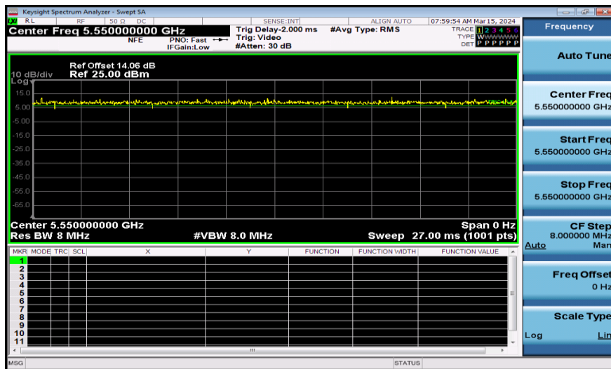
NTNV-11N40SISO-Ant1-5550
