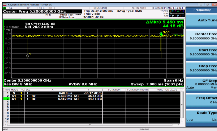
NTNV-11N20SISO-Ant1-5200
