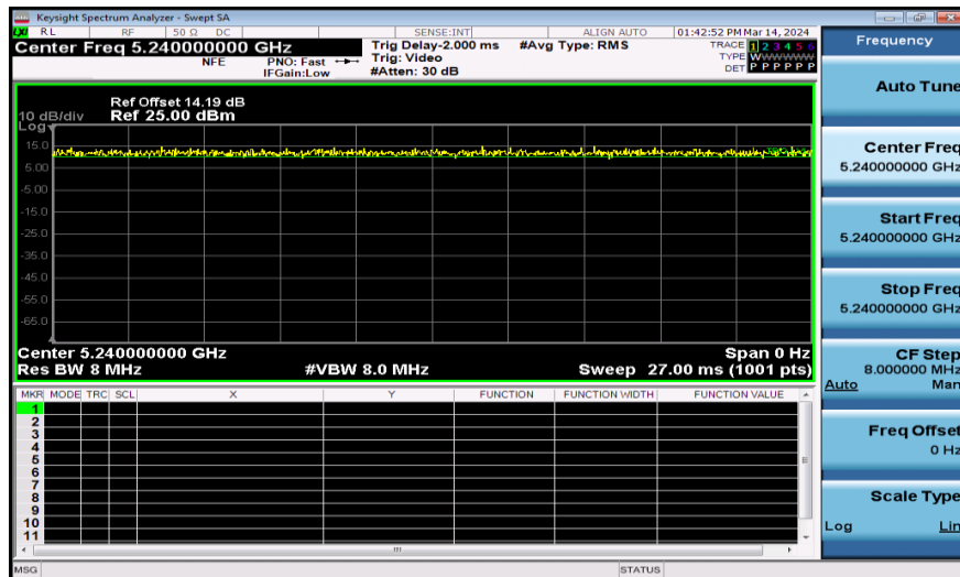
NTNV-11N20SISO-Ant1-5240
