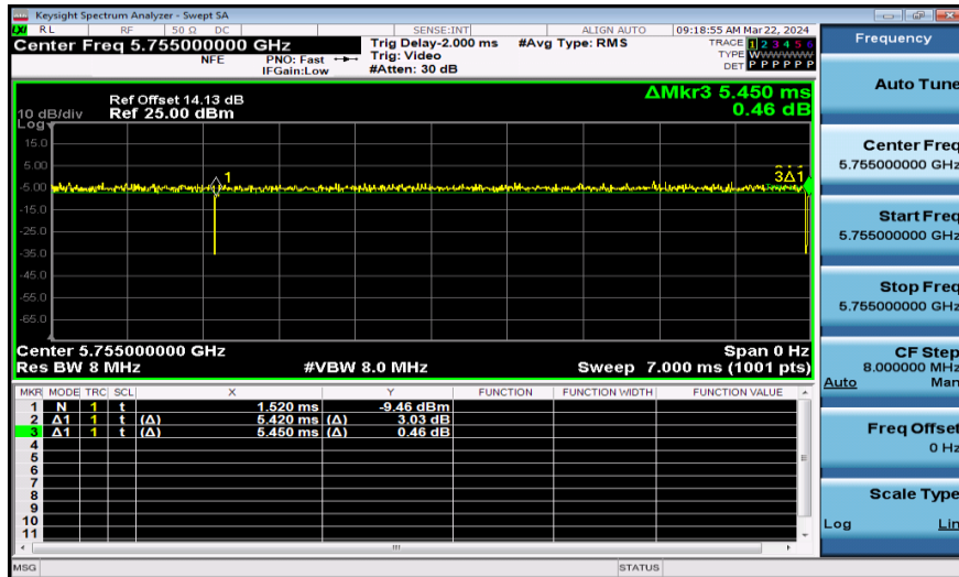
NTNV-11AC40SISO-Ant1-5755
