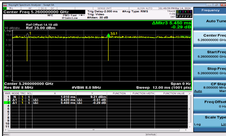
NTNV-11N20SISO-Ant1-5260
