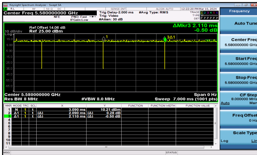
NTNV-11A-Ant1-5580
