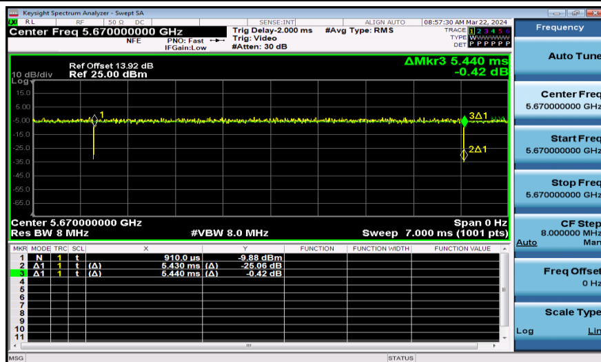
NTNV-11AC40SISO-Ant1-5670
