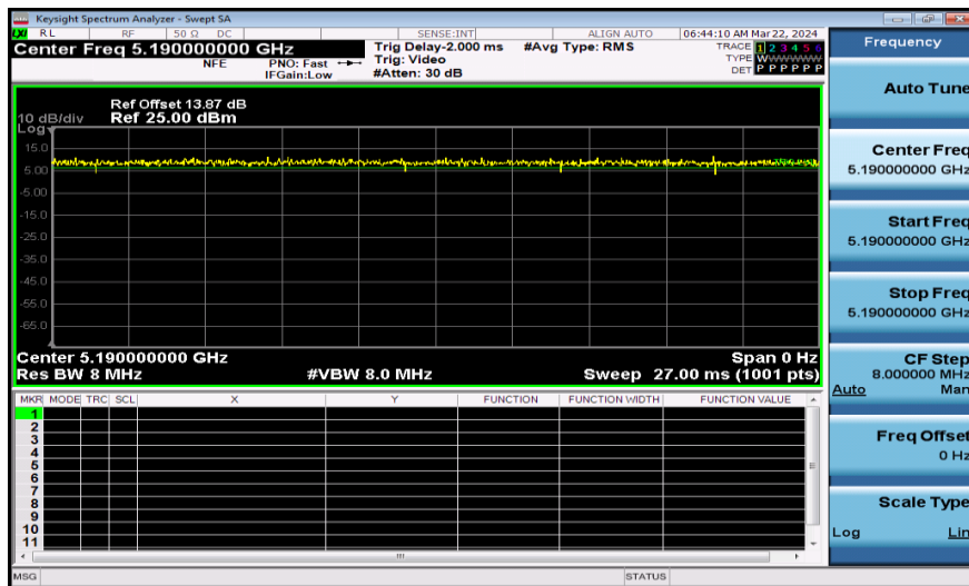
NTNV-11AC40SISO-Ant1-5190
