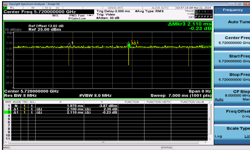
NTNV-11A-Ant1-5720
