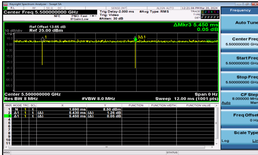
NTNV-11AC20SISO-Ant1-5500
