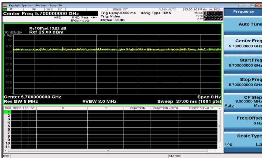
NTNV-11N20SISO-Ant1-5700
