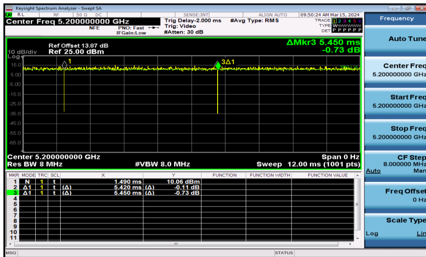
NTNV-11AC20SISO-Ant1-5200
