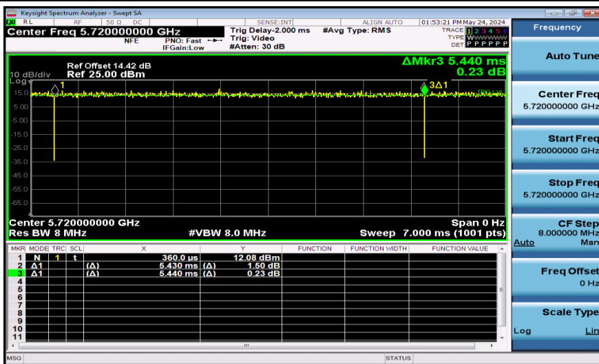
NTNV-11N20SISO-Ant1-5720
