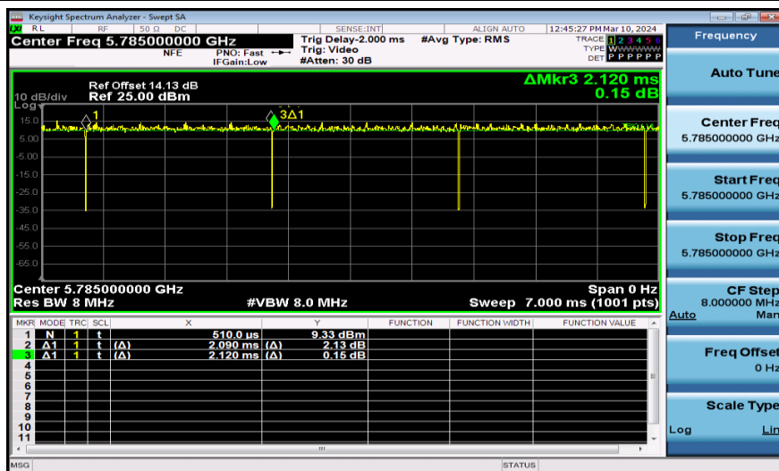
NTNV-11A-Ant1-5785
