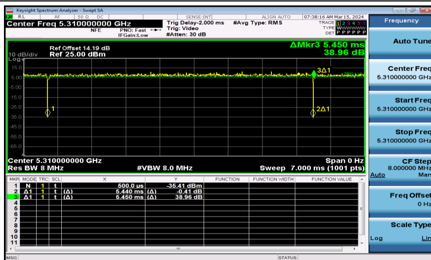
NTNV-11N40SISO-Ant1-5310
