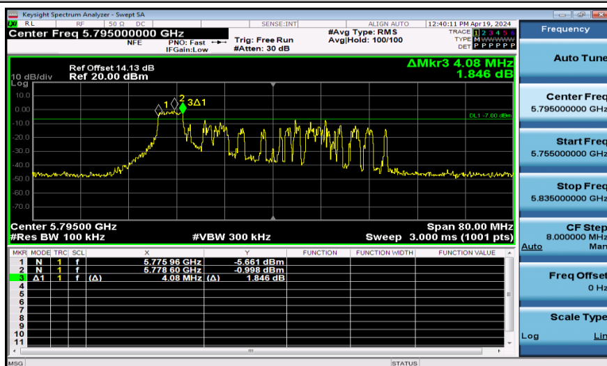
11AX40SISO-Ant1-5795-52Tone-PASS
