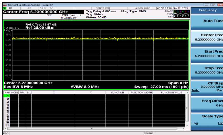
NTNV-11AC40SISO-Ant1-5230
