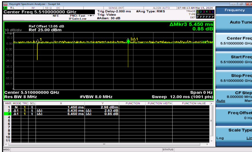
NTNV-11N40SISO-Ant1-5510
