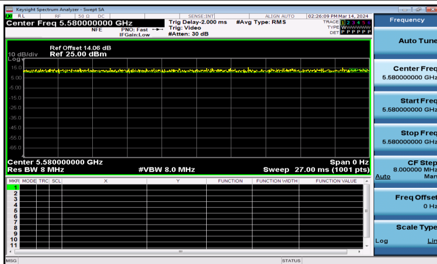
NTNV-11N20SISO-Ant1-5580
