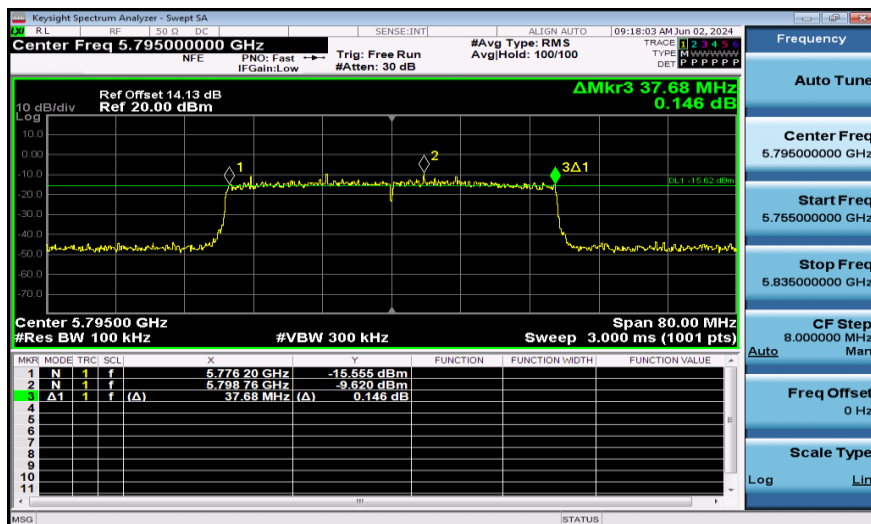
11AX40SISO-Ant1-5795-484Tone-PASS
