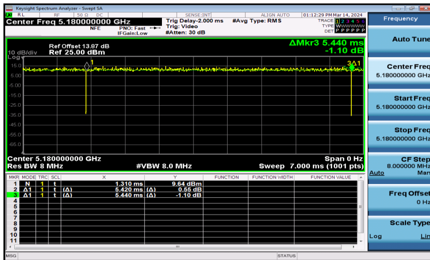
NTNV-11N20SISO-Ant1-5180
