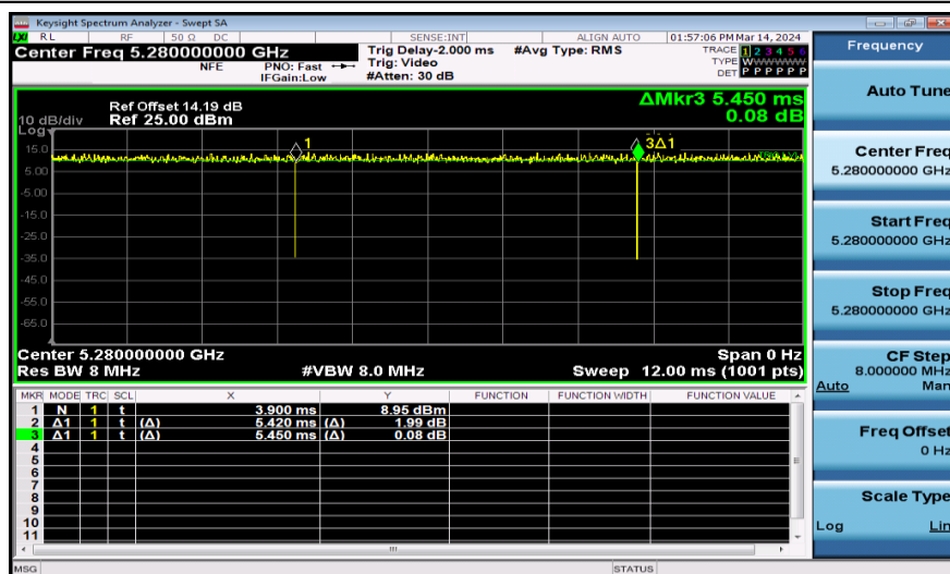
NTNV-11N20SISO-Ant1-5280
