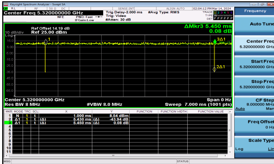
NTNV-11N20SISO-Ant1-5320
