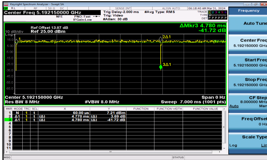
NTNV-11AX20SISO-Ant1-5200-106Tone
