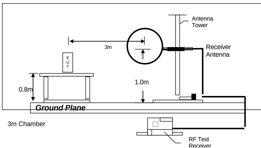
Test setup of radiated emissions up to 30MHz
