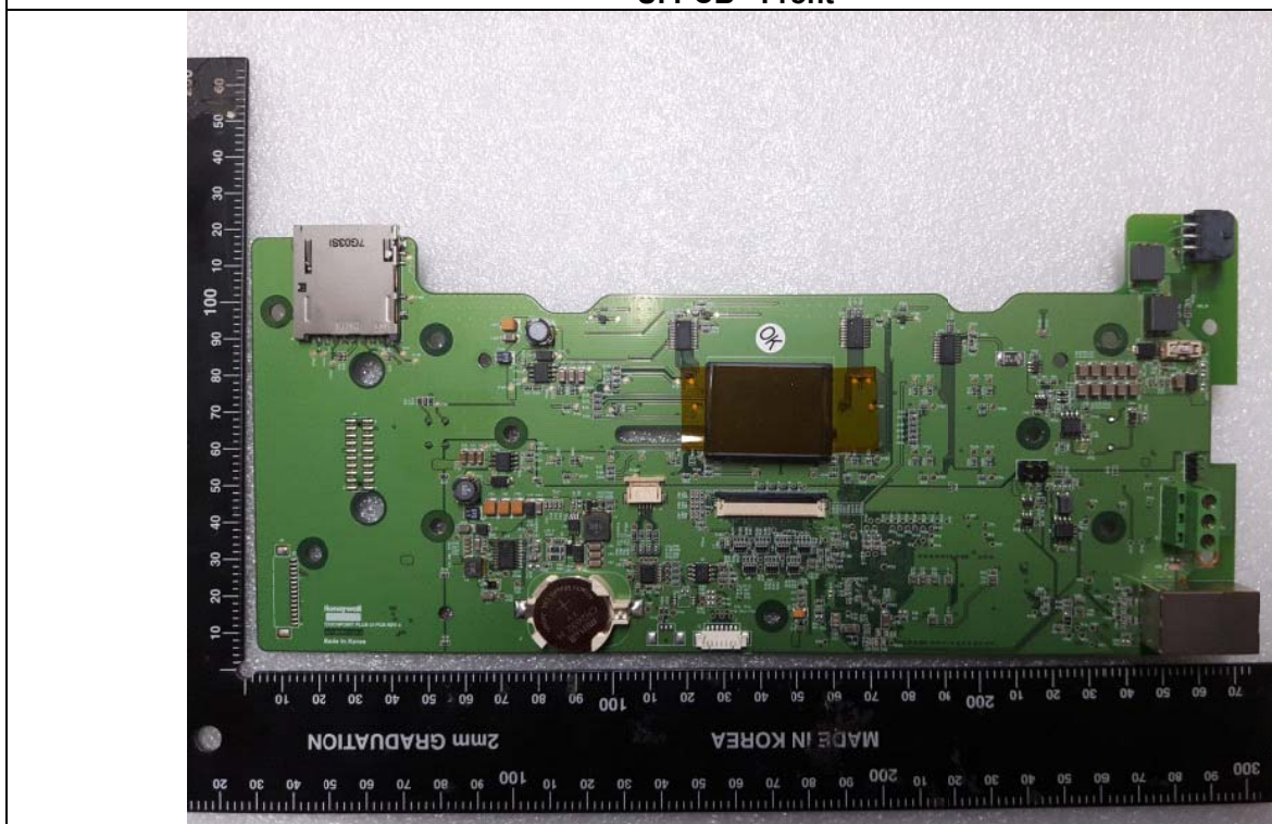
UI PCB - Front
