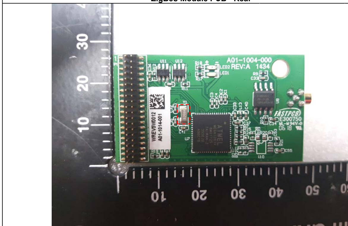
ZigBee Module PCB - Rear
