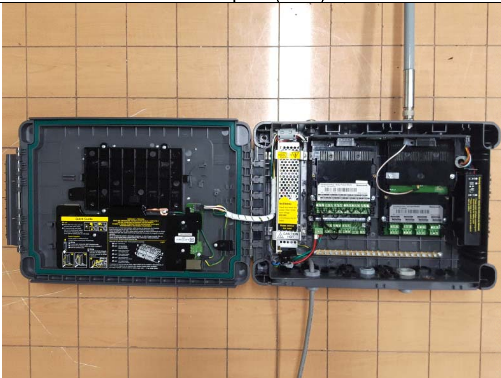
Cover opened (Indoor)
