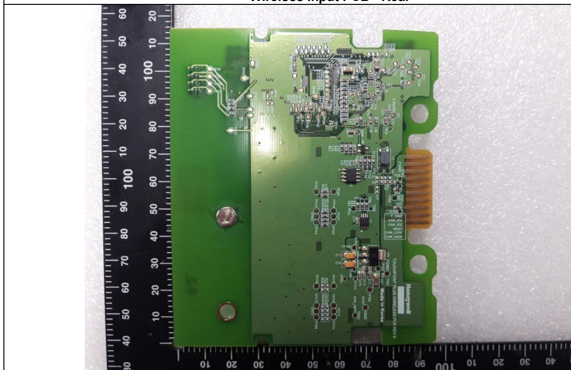
Wireless Input PCB - Rear
