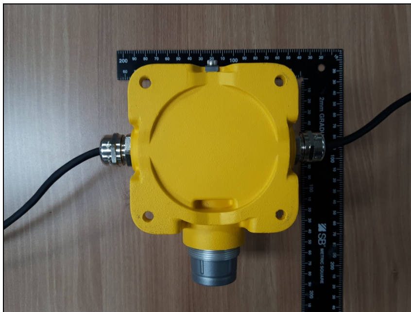
Bottom view of Host (SPLIFRBAXCMNZZ)
