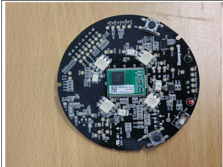
Top view of Host(Main board)
