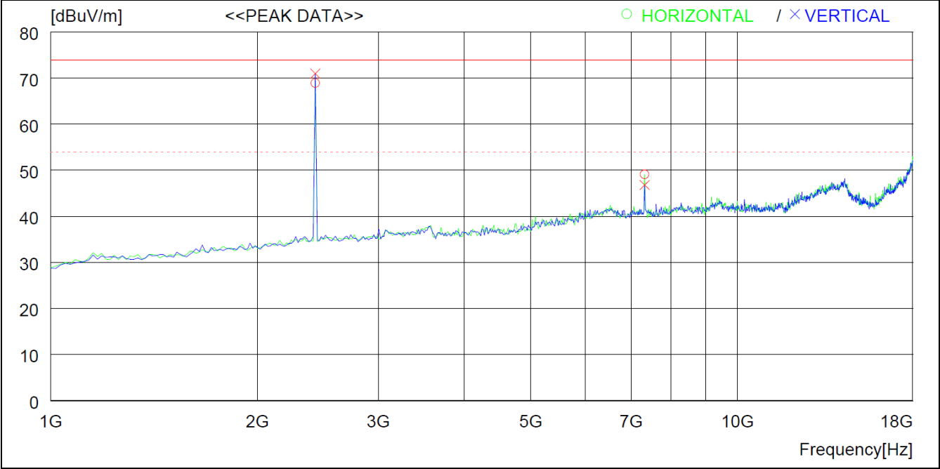
Figure 5. GFSK: Mid
