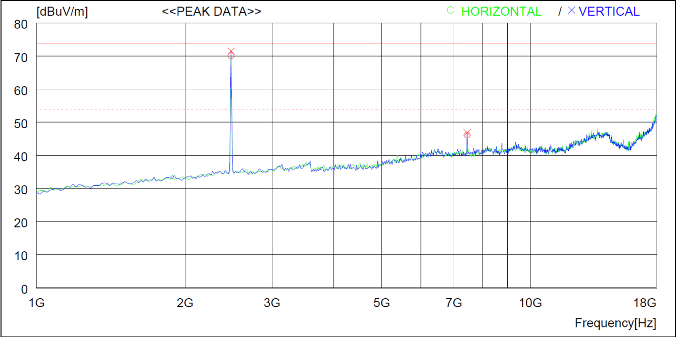
Figure 6. GFSK: High
