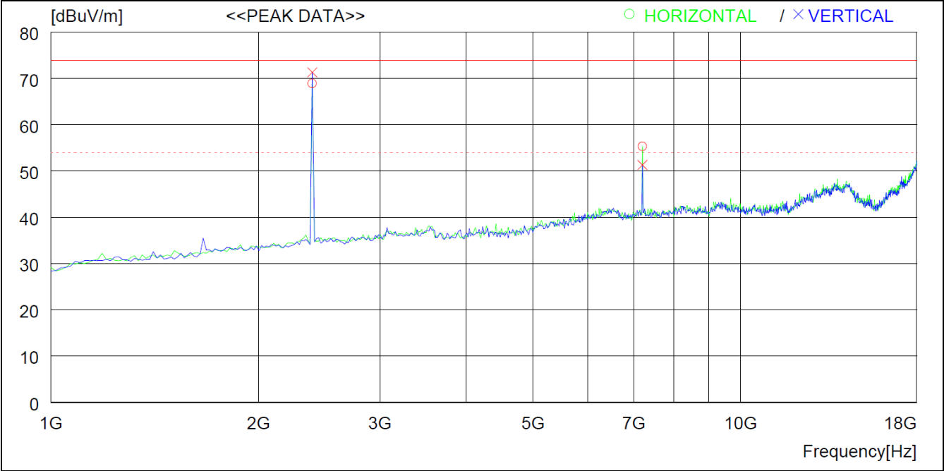
Figure 4. GFSK : Low
