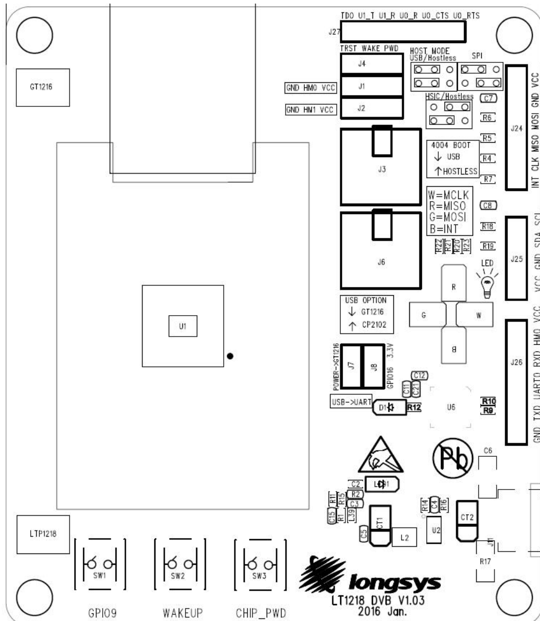
Figure 2-1 Top Screen of the LTP1218 development board
