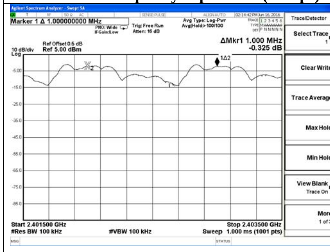
Test Plot of Frequency Separation (3Mbps)
