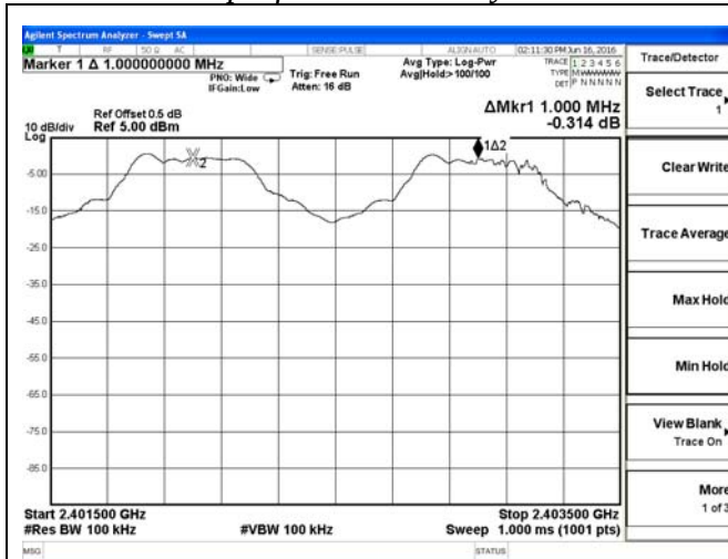
Test Plot of Frequency Separation (1Mbps)
