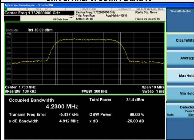
Channel 1413 / 1732.6 MHz
