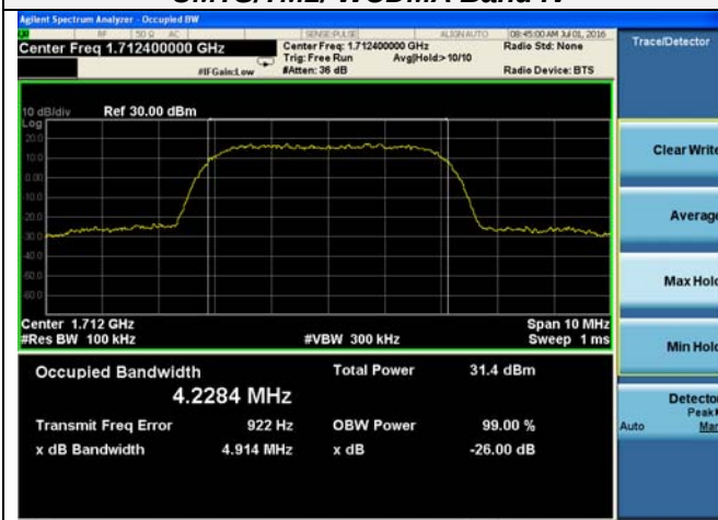
Channel 1312 / 1712.4 MHz
