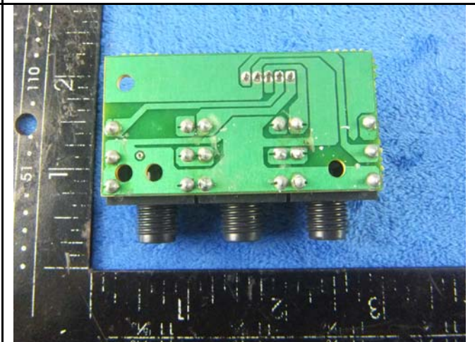
MIC&Guiton in board - Rear View
