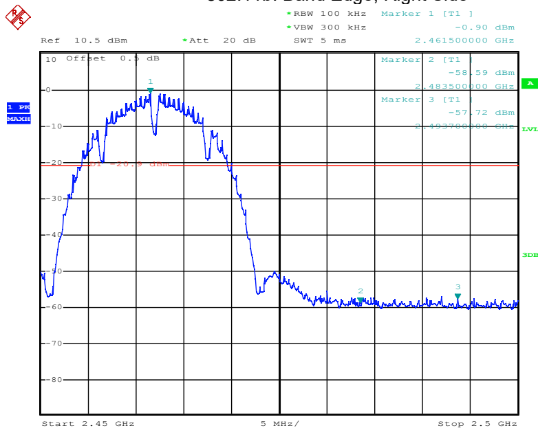
802.11b: Band Edge, Right Side
