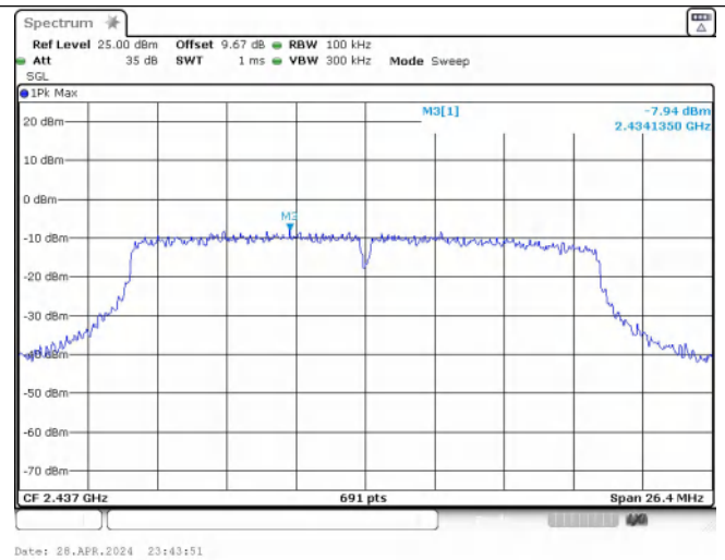
In-Band Reference Level IEEE 802.11n_Channel 6_20MHz_Antenna 0
