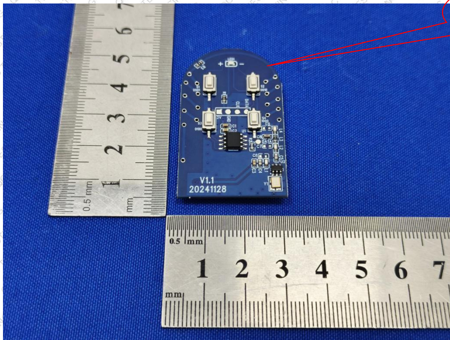
433M TX Antenna
