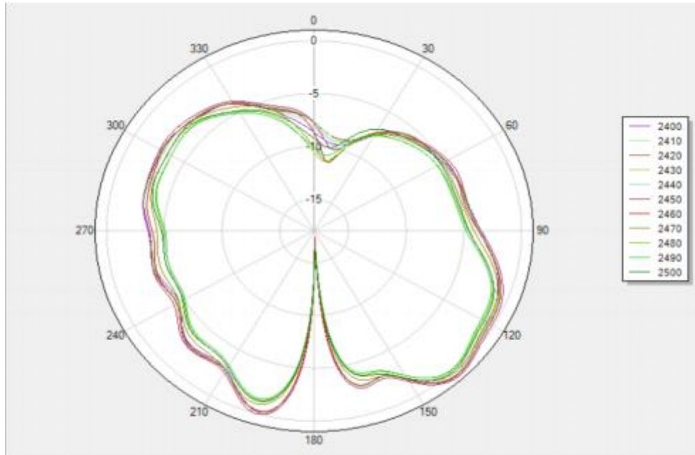
Phi 0 2D
