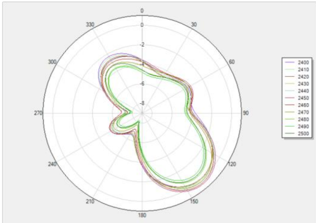
Theta 90 2D
