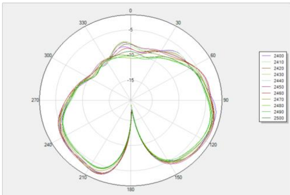
Phi 90 2D
