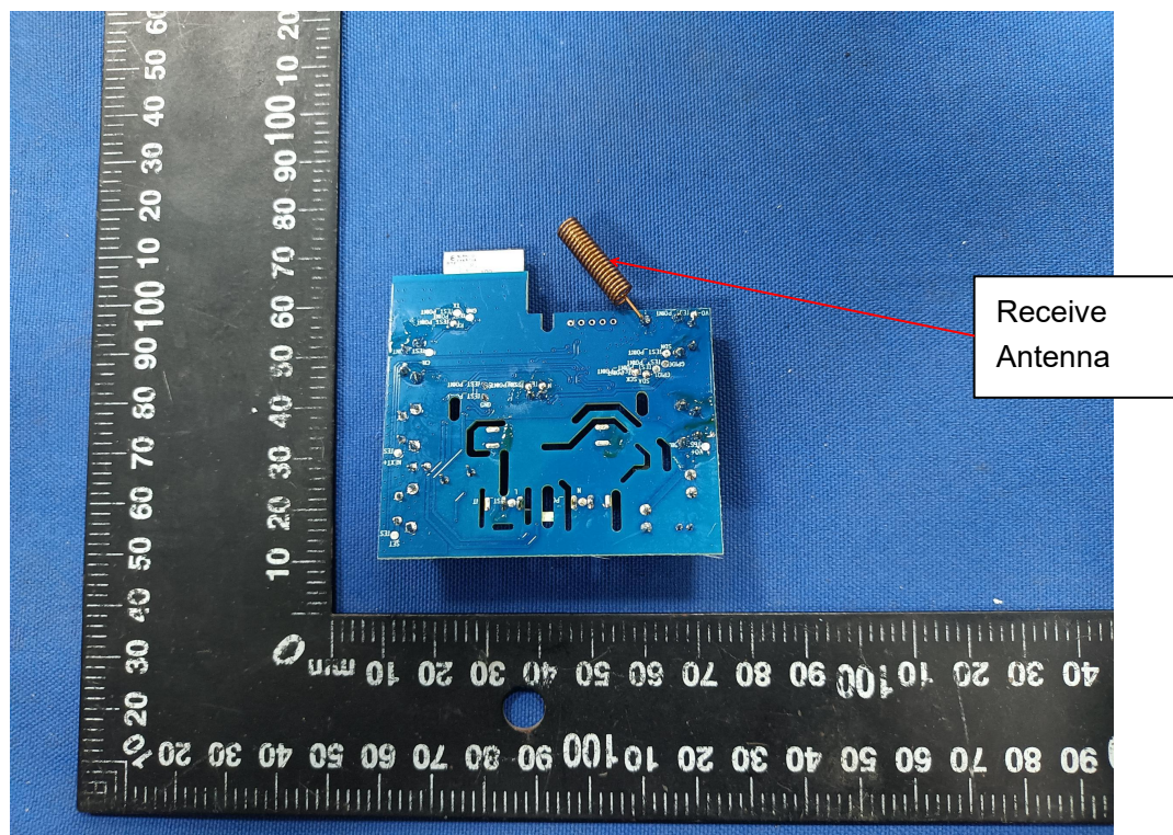
Fig.4 It is only receive antenna.(433.9200MHz)
