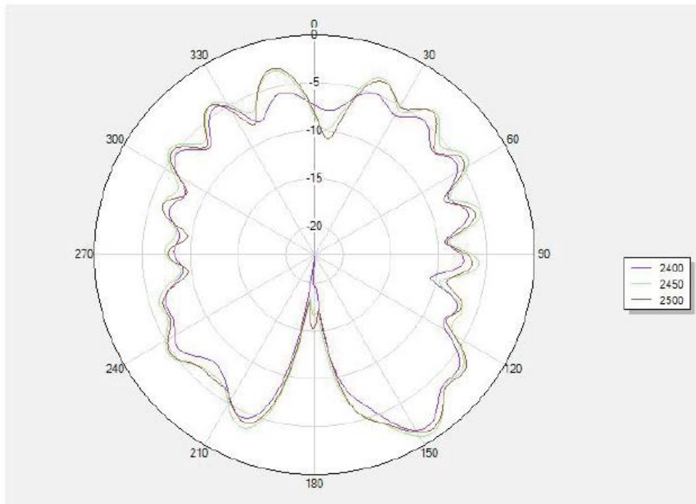
Phi 90 2D
