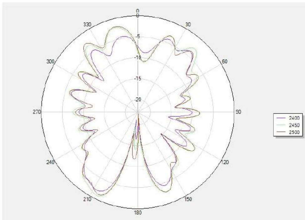
Phi 90 2D
