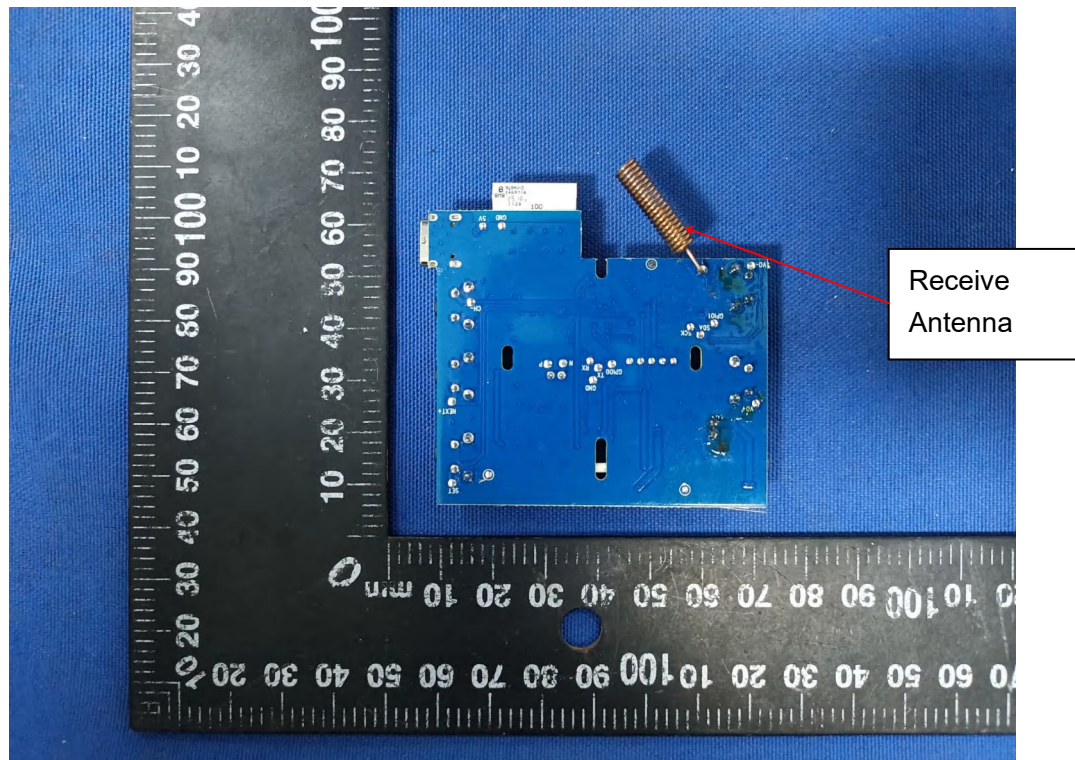
Fig.5 It is only receive antenna.(433.9200MHz)
