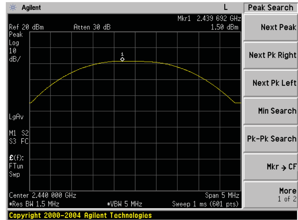
Peak output Power plot on channel 19
