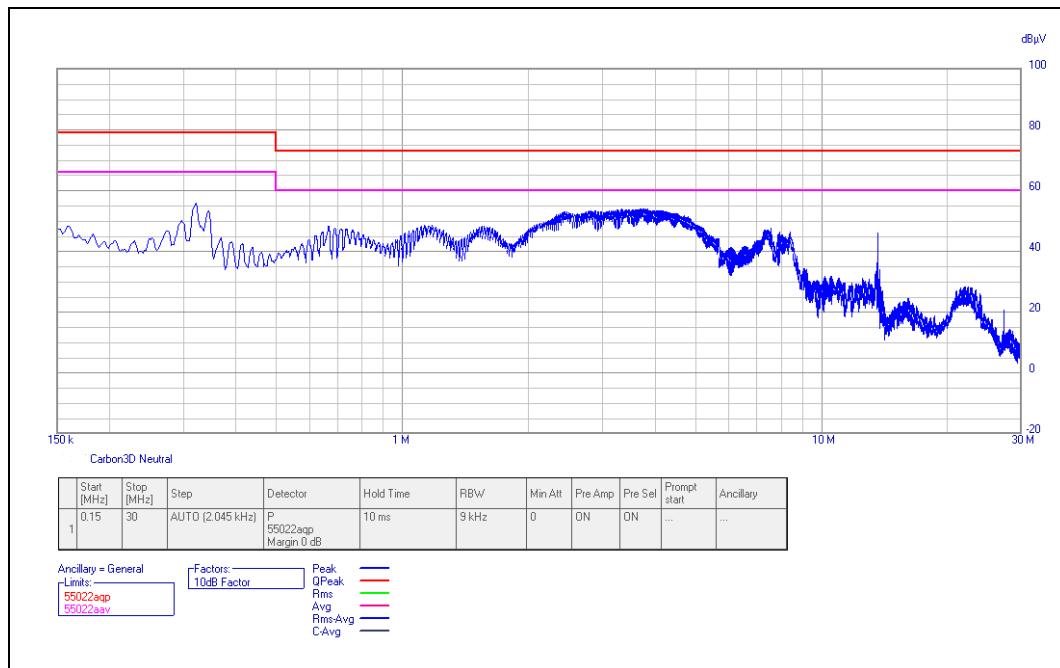
Plot 2. Conducted Emissions, 15.207(a), Neutral Line
