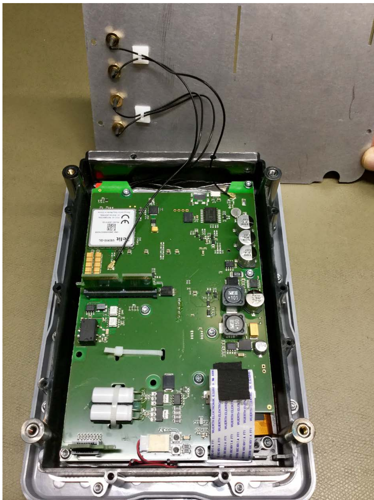
WK60_ElectronicOpenBack
